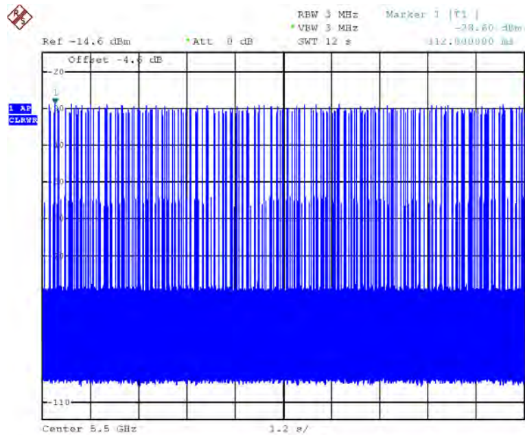
EUT (Slave) Data Traffic Plot (20 MHz)
