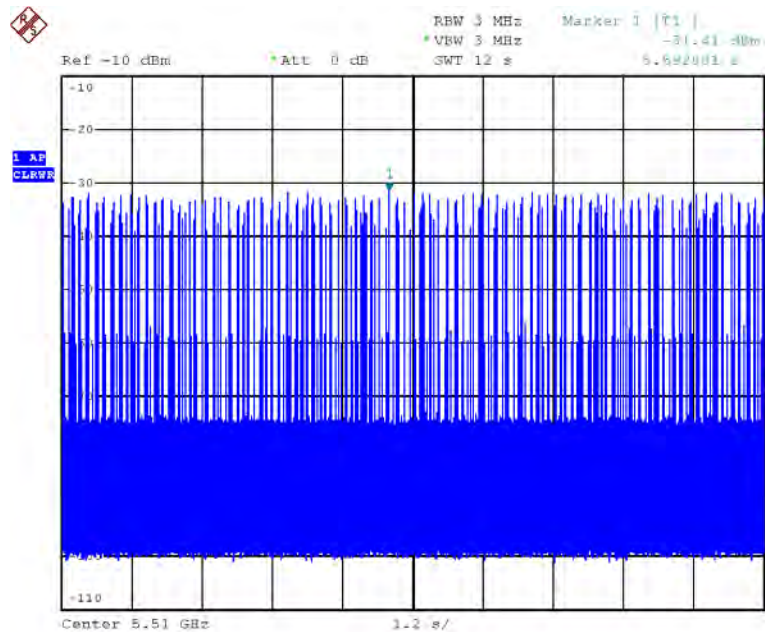
EUT (Slave) Data Traffic Plot (40 MHz)
