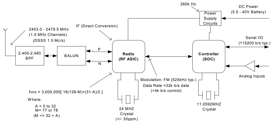
Figure 2 Block Diagram
