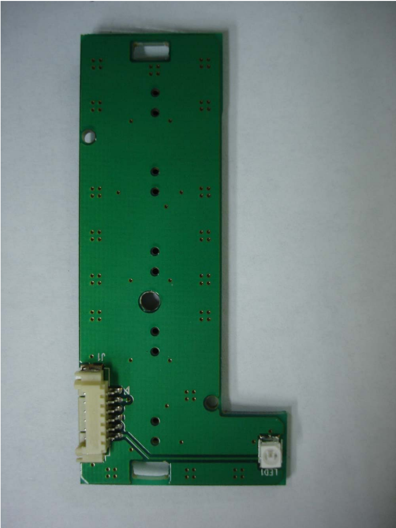
<Key Rear>
