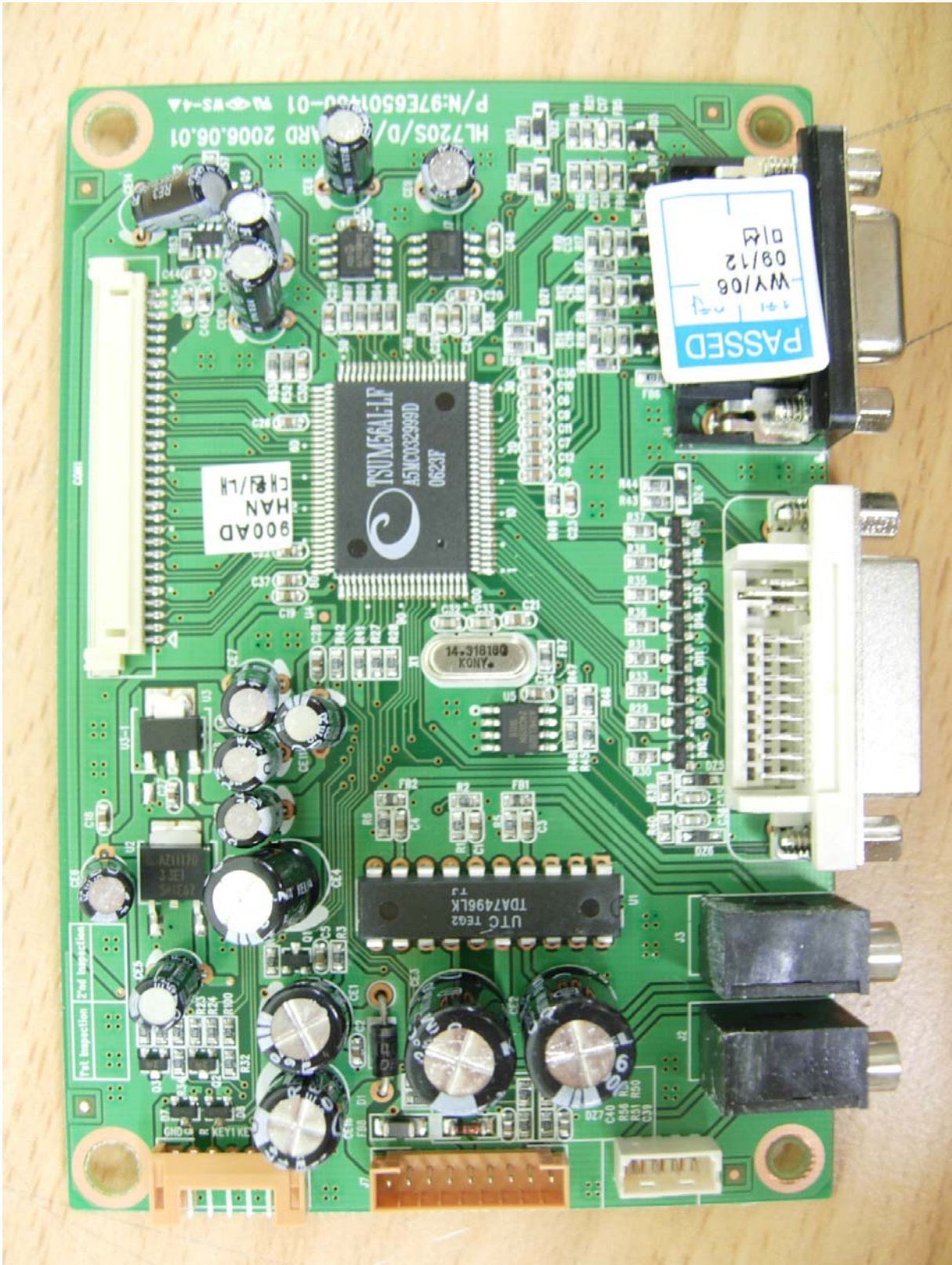
<Mainboard Front>
