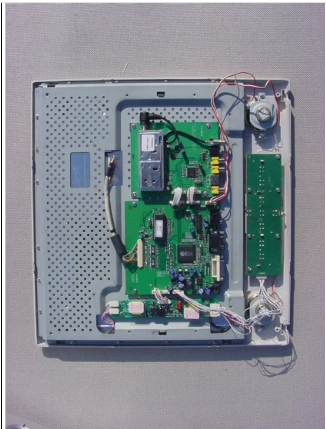
[ Inside View of the Hyundai Panel Installed after Shielded Case Open ]
