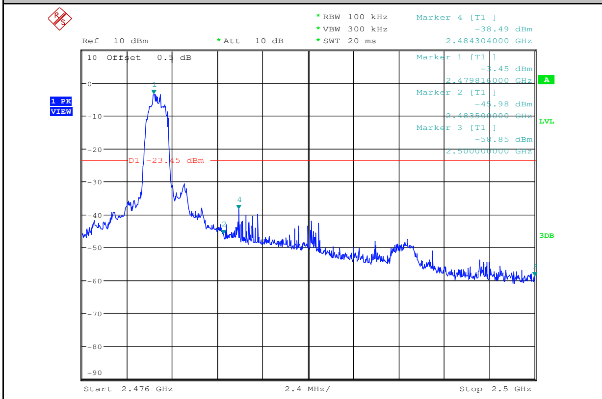
Band-edge for RF Conducted Emissions_3DH5_2480_Hopping Off
