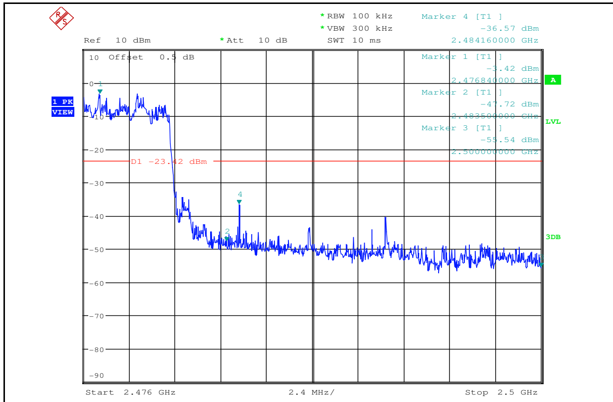
Band-edge for RF Conducted Emissions_2DH5_2480_Hopping Off
