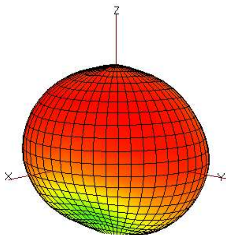
Passive Test E-Total (Y-Z Plane)
