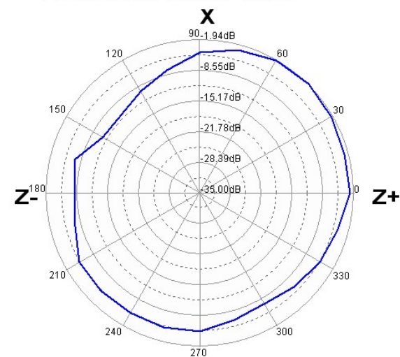
Passive Test E-Total (X-Z Plane)
