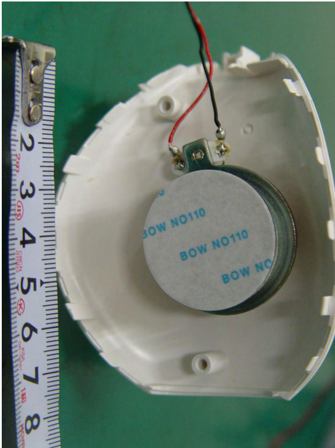
< Inside #3 >
