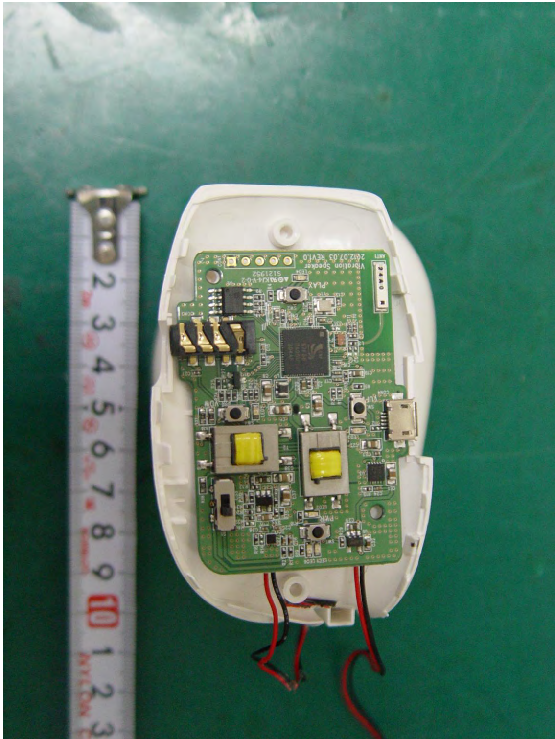
< Inside #1 >
