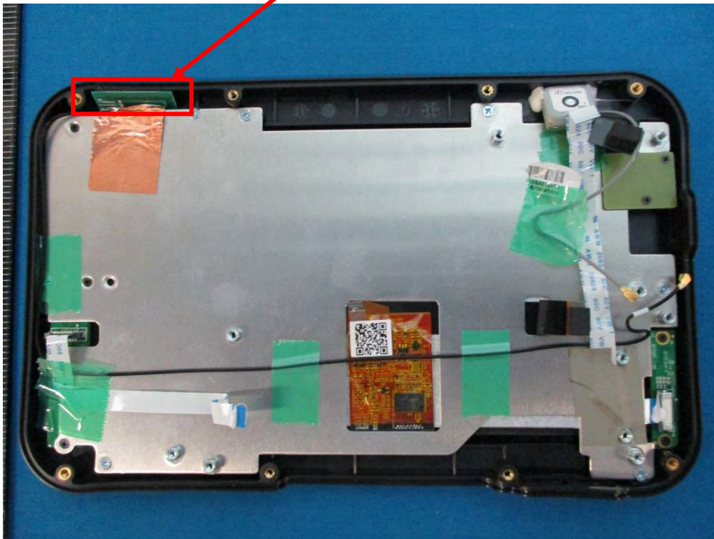
Bluetooth LE & WIFI Antenna – Location View 1
