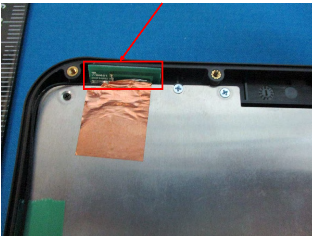
Bluetooth LE & WIFI Antenna – Location View 2
