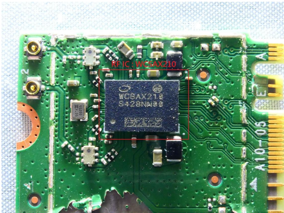
(29) EUT Photo
