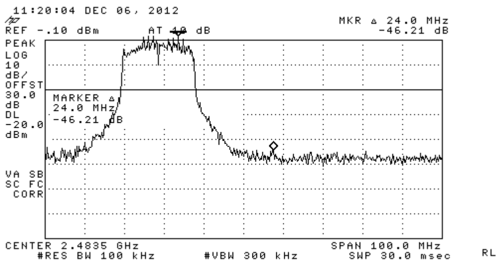
highow Band Edge(802.11n mode Modulation : : 64QAM)
