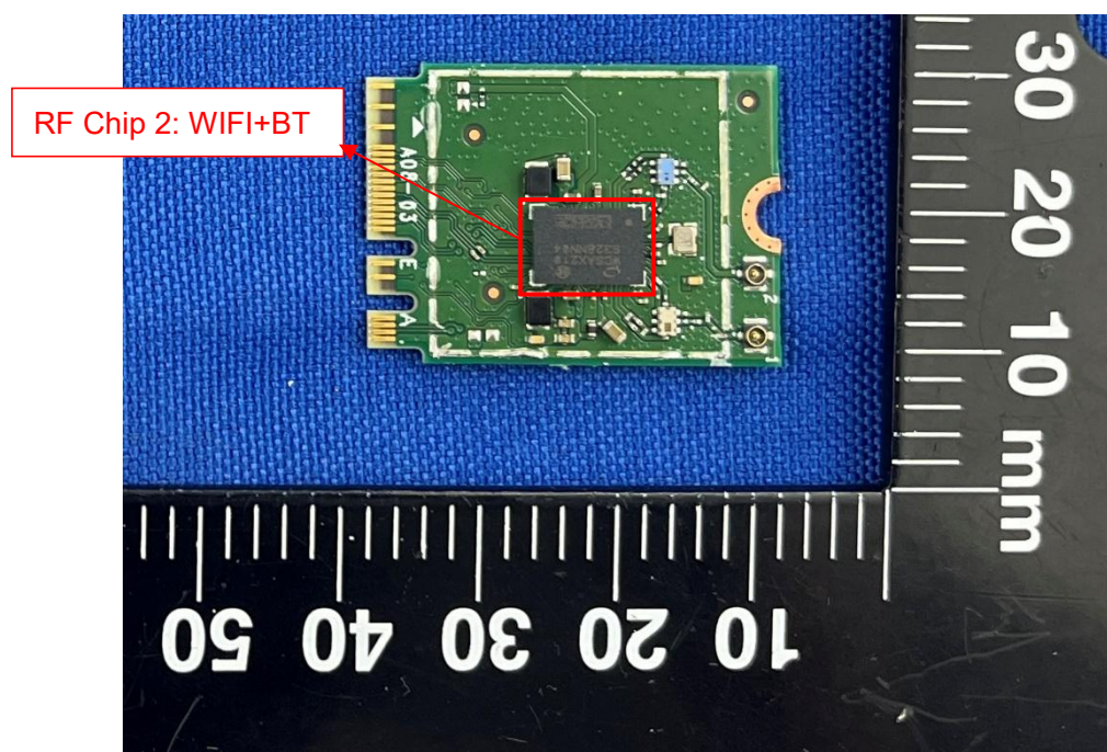
SECONDARY BOARD 1 TOP VIEW (WITHOUT SHIELDING)
