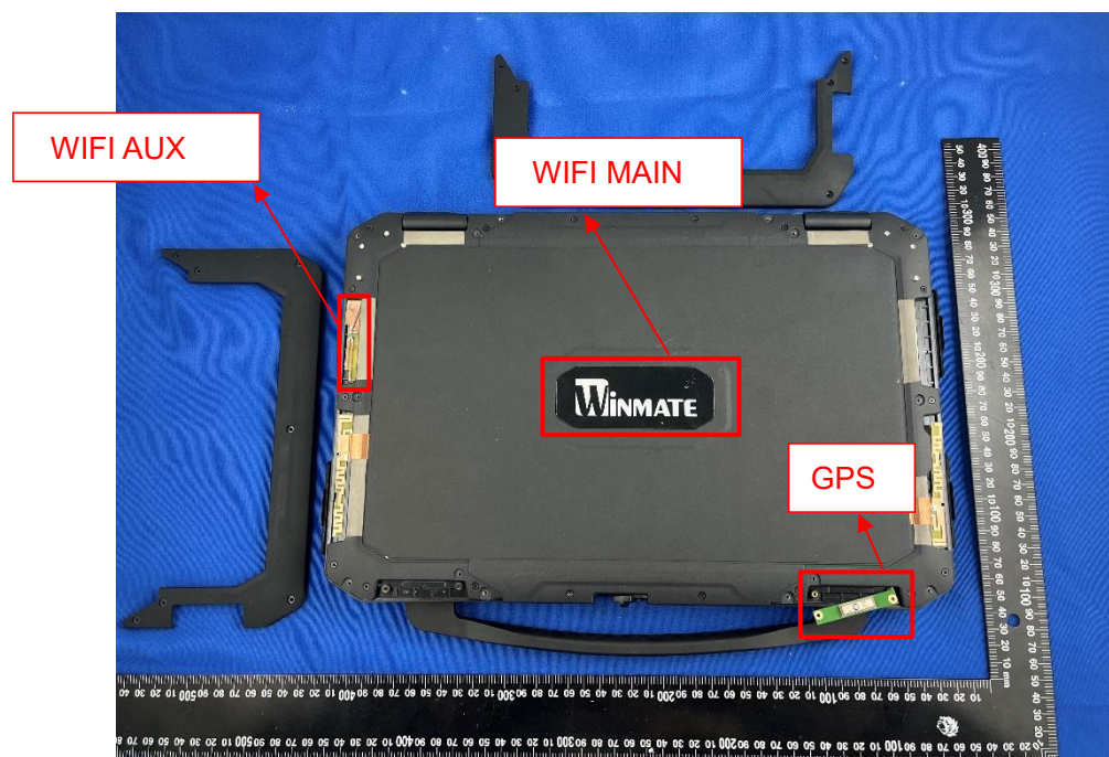
EUT UNCOVER VIEW 8
