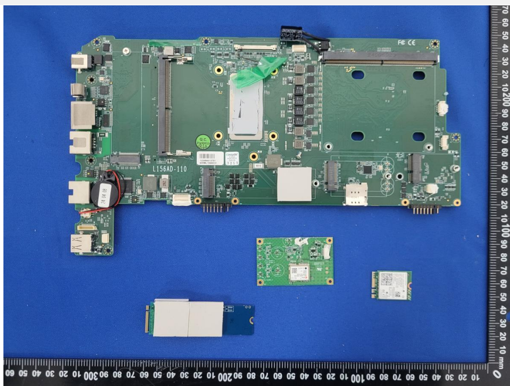
EUT UNCOVER VIEW 6
