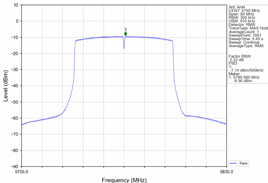
802.11ax(HEW40)_HCH_5795MHz_RU26_Left_MIMO_NTNV
