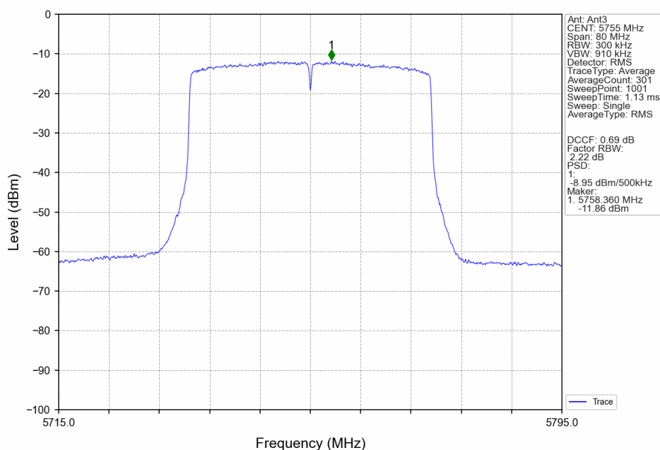
802.11ax(HEW40)_LCH_5755MHz_RU26_Right_Ant3_NTNV
