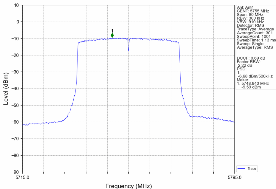
802.11ax(HEW40)_LCH_5755MHz_RU26_Right_MIMO_NTNV
