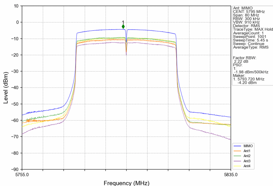
802.11ax(HEW40)_HCH_5795MHz_RU26_Right_MIMO_NTNV
