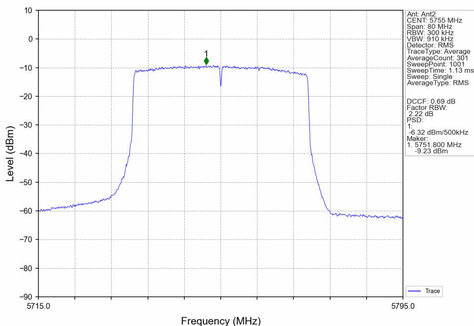
802.11ax(HEW40)_LCH_5755MHz_RU26_Mid_Ant2_NTNV
