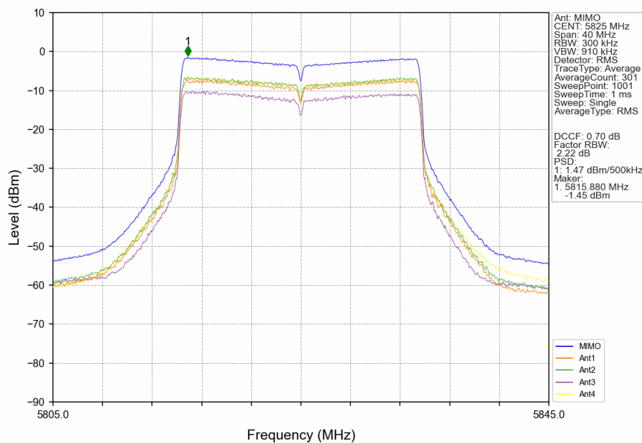
802.11ax(HEW20)_HCH_5825MHz_RU26_Left_MIMO_NTNV
