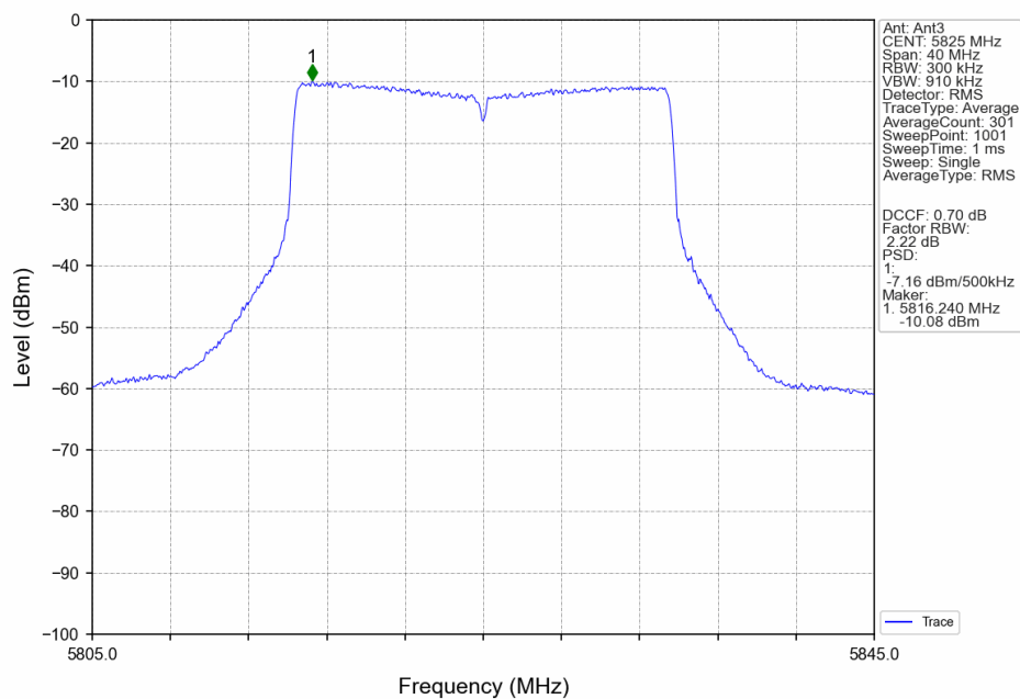
802.11ax(HEW20)_HCH_5825MHz_RU26_Left_Ant3_NTNV
