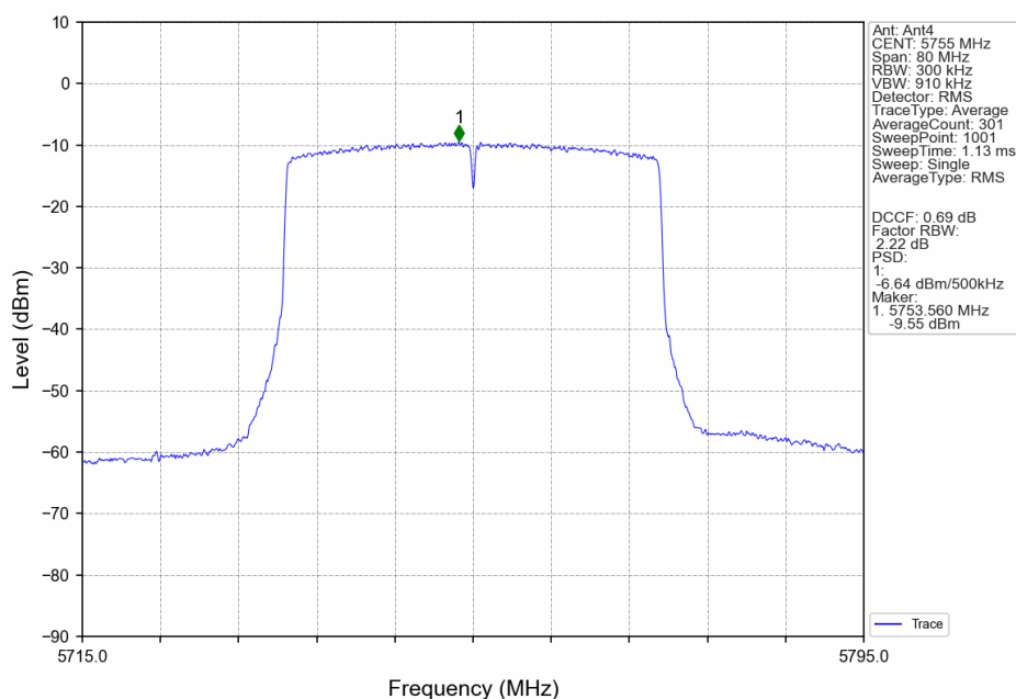
802.11ax(HEW40)_LCH_5755MHz_RU26_Mid_Ant4_NTNV
