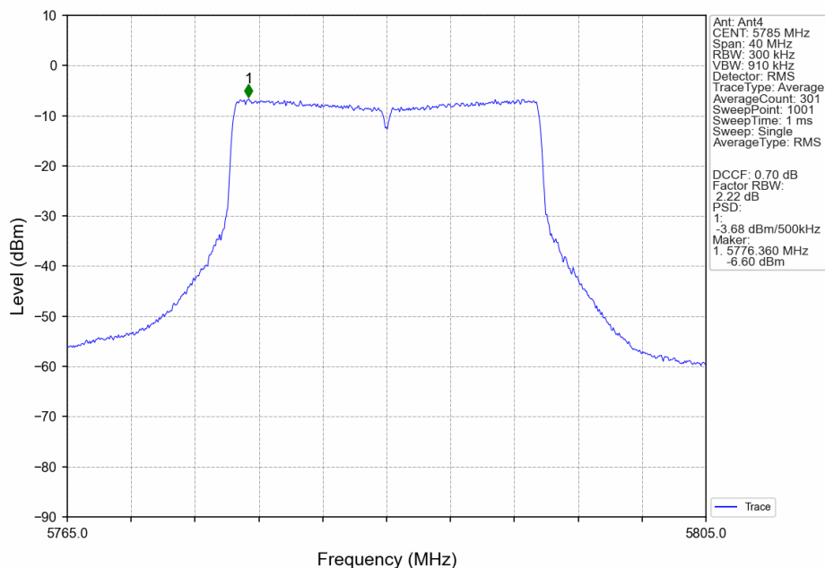
802.11ax(HEW20)_MCH_5785MHz_RU26_Right_MIMO_NTNV
