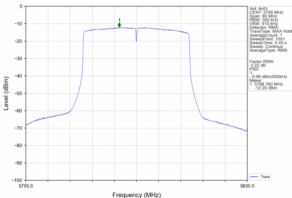
802.11ax(HEW40)_HCH_5795MHz_RU26_Right_Ant3_NTNV
