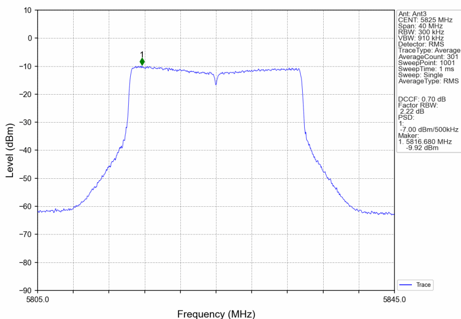
802.11ax(HEW20)_HCH_5825MHz_RU26_Right_Ant3_NTNV
