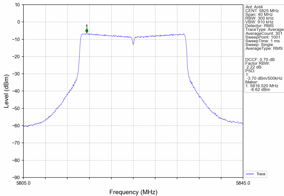
802.11ax(HEW20)_HCH_5825MHz_RU26_Right_MIMO_NTNV
