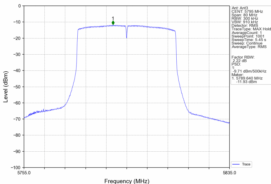
802.11ax(HEW40)_HCH_5795MHz_RU26_Left_Ant3_NTNV
