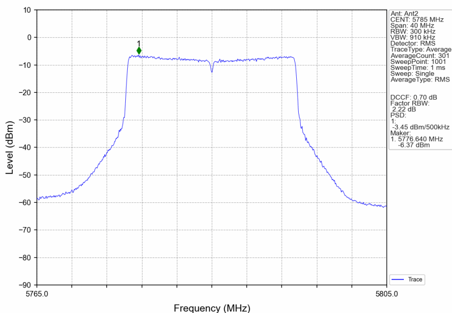
802.11ax(HEW20)_MCH_5785MHz_RU26_Mid_Ant2_NTNV
