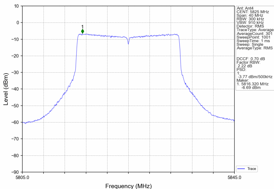
802.11ax(HEW20)_HCH_5825MHz_RU242_Left_Ant4_NTNV
