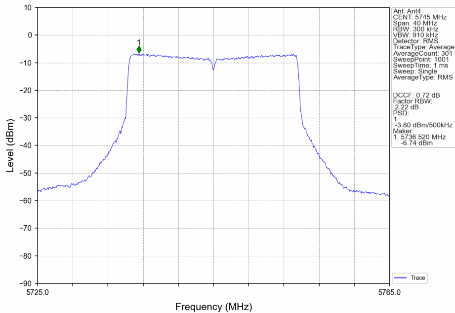
802.11ax(HEW20)_LCH_5745MHz_RU26_Right_MIMO_NTNV
