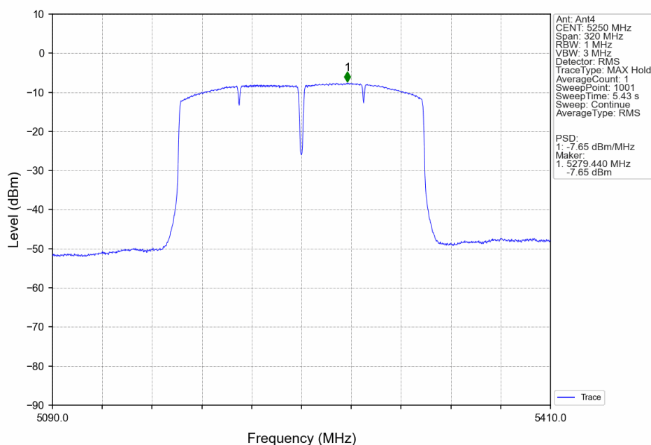
802.11ax(HEW160)_MCH_5250MHz_RU26_Mid_Ant4_NTNV
