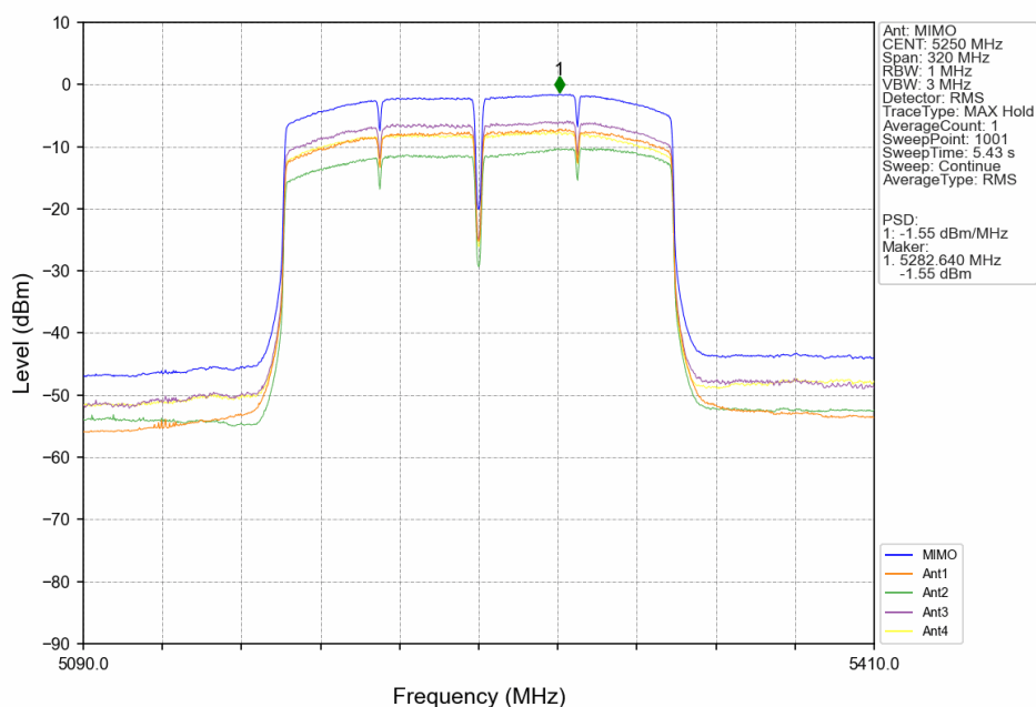
802.11ax(HEW160)_MCH_5250MHz_RU26_Right_MIMO_NTNV
