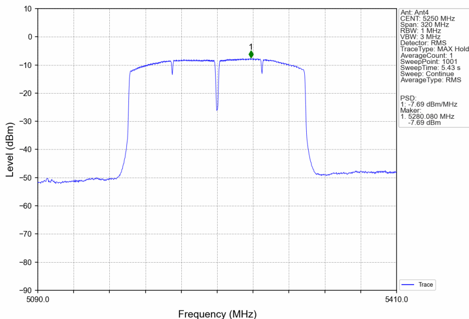
802.11ax(HEW160)_MCH_5250MHz_RU26_Left_MIMO_NTNV
