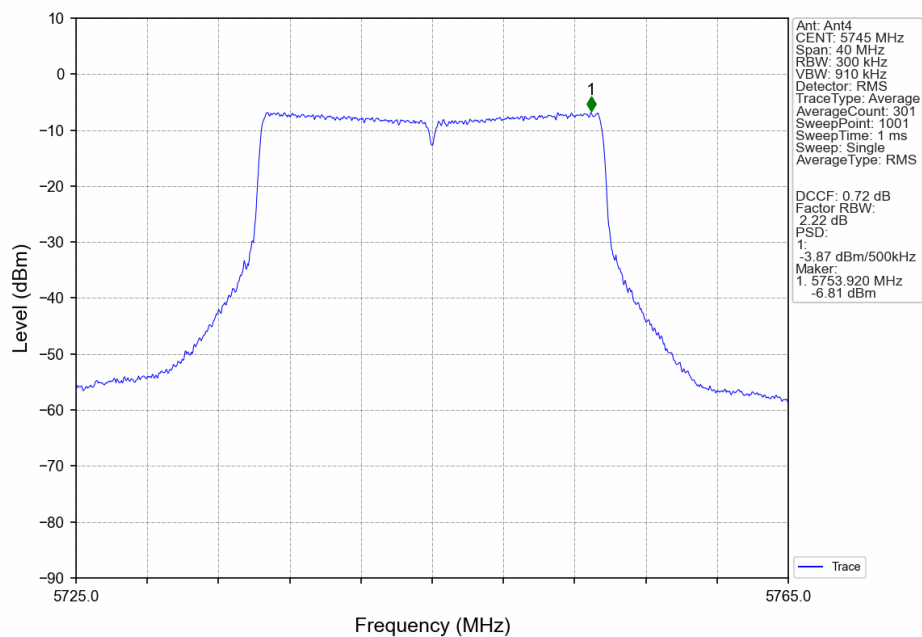
802.11ax(HEW20)_LCH_5745MHz_RU26_Mid_Ant4_NTNV
