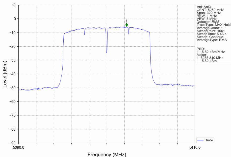
802.11ax(HEW160)_MCH_5250MHz_RU26_Right_Ant3_NTNV
