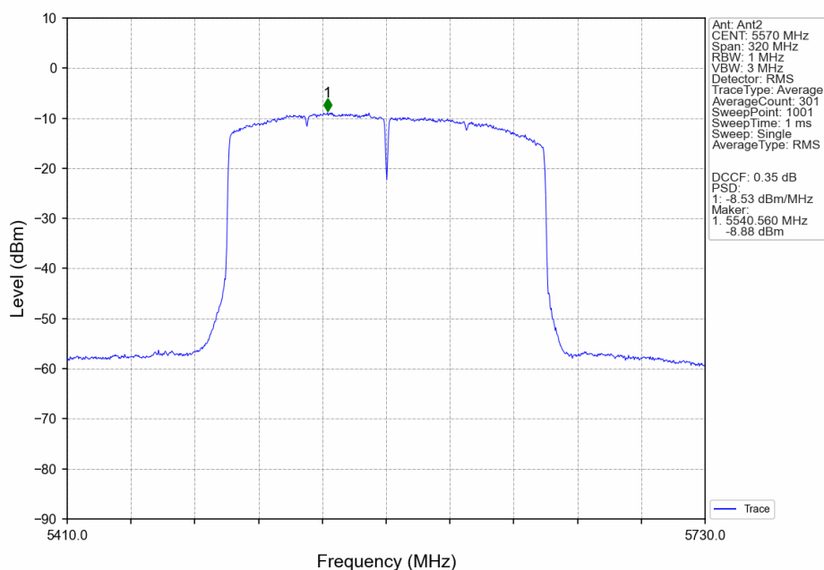
802.11ax(HEW160)_MCH_5570MHz_RU26_Left_Ant2_NTNV
