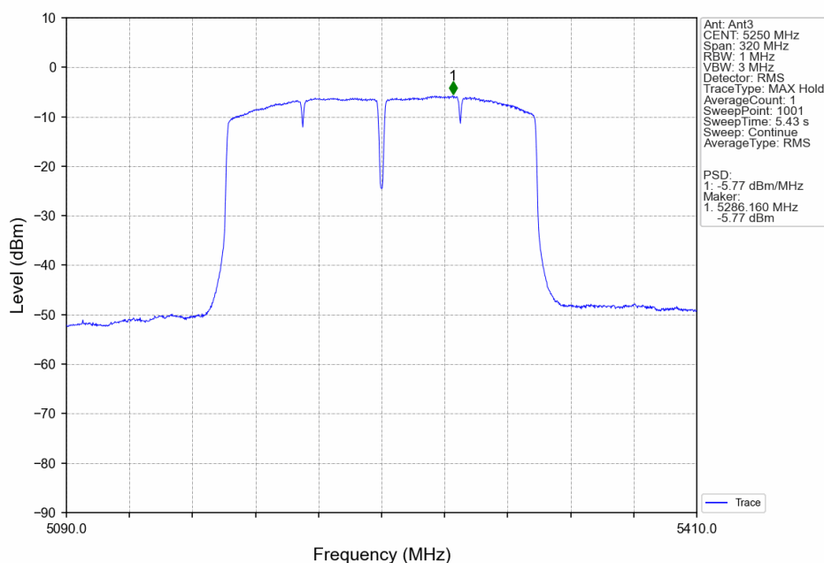
802.11ax(HEW160)_MCH_5250MHz_RU26_Left_Ant3_NTNV
