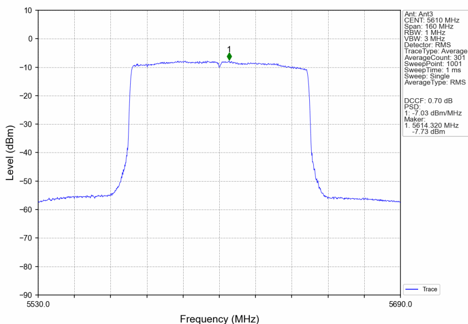
802.11ax(HEW80)_HCH_5610MHz_RU26_Mid_Ant3_NTNV
