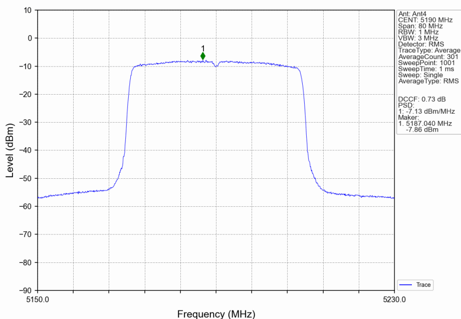
802.11ax(HEW40)_LCH_5190MHz_RU26_Right_Ant4_NTNV
