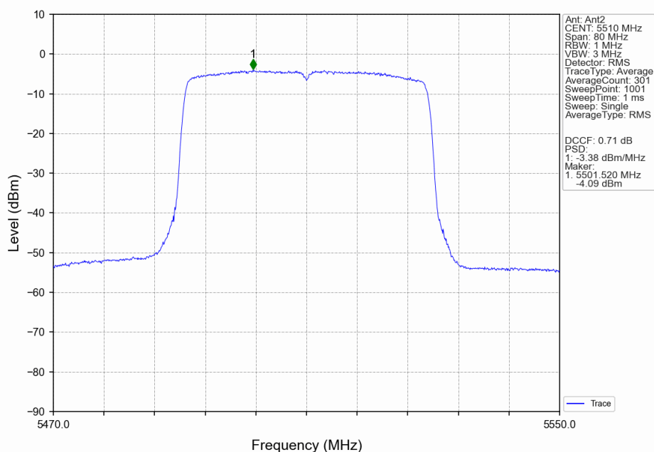
802.11ax(HEW40)_LCH_5510MHz_RU26_Right_Ant2_NTNV
