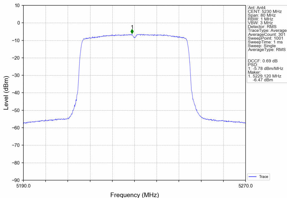
802.11ax(HEW40)_HCH_5230MHz_RU26_Mid_MIMO_NTNV
