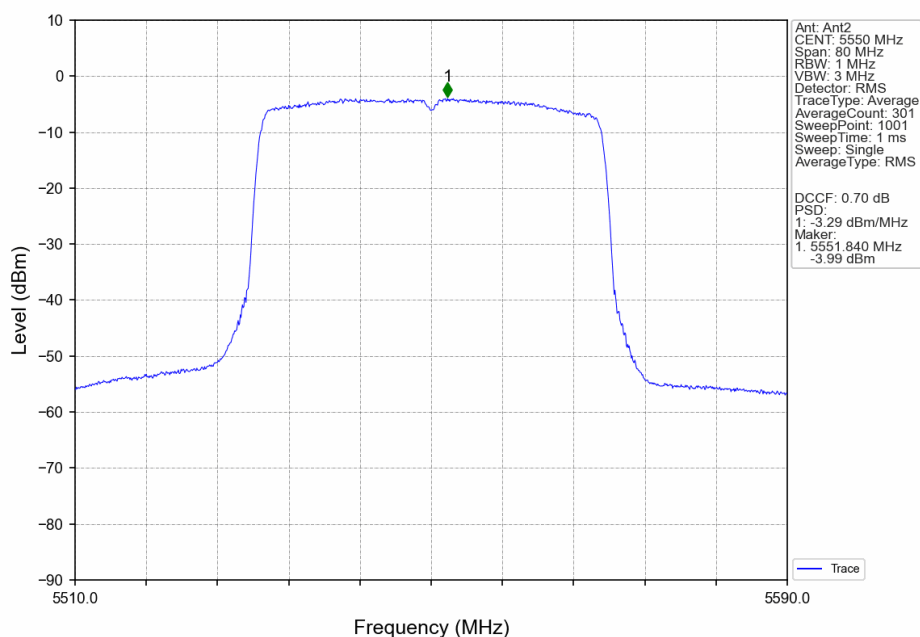
802.11ax(HEW40)_MCH_5550MHz_RU26_Left_Ant2_NTNV
