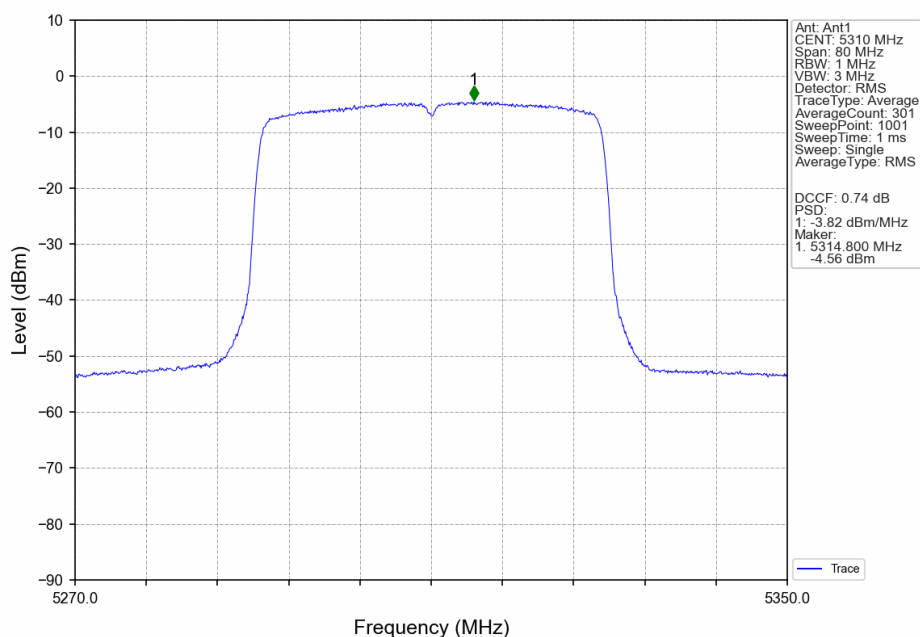
802.11ax(HEW40)_HCH_5310MHz_RU26_Mid_Ant1_NTNV
