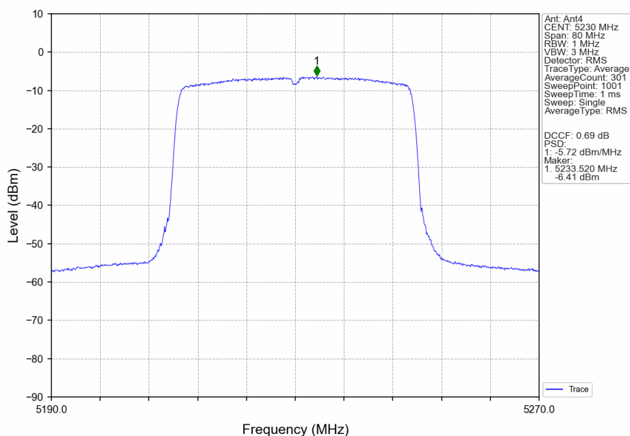
802.11ax(HEW40)_HCH_5230MHz_RU26_Right_Ant4_NTNV
