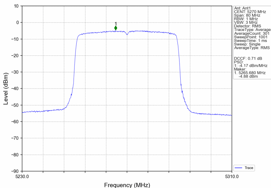
802.11ax(HEW40)_LCH_5270MHz_RU26_Mid_Ant1_NTNV
