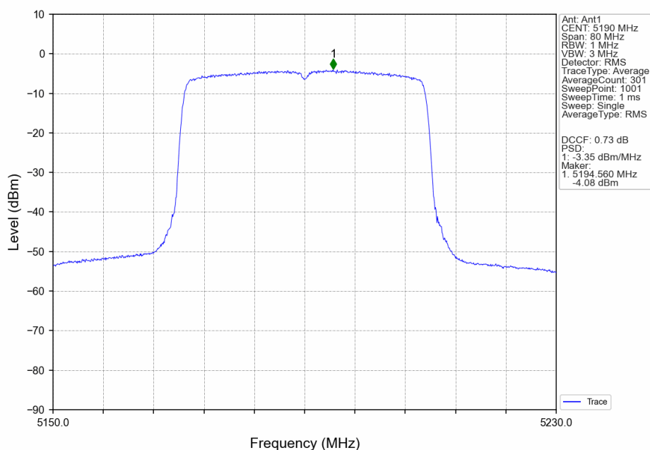
802.11ax(HEW40)_LCH_5190MHz_RU26_Mid_Ant1_NTNV
