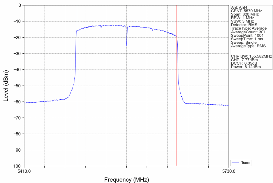
802.11ax(HEW160)_MCH_5570MHz_2xRU996_Left_Ant4_NTNV
