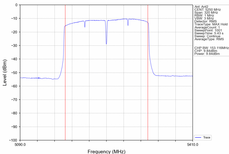
802.11ax(HEW160)_MCH_5250MHz_RU26_Mid_Ant2_NTNV
