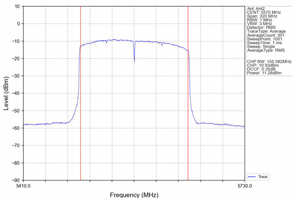
802.11ax(HEW160)_MCH_5570MHz_RU26_Right_Ant2_NTNV
