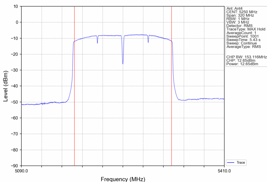
802.11ax(HEW160)_MCH_5250MHz_RU26_Right_Ant4_NTNV
