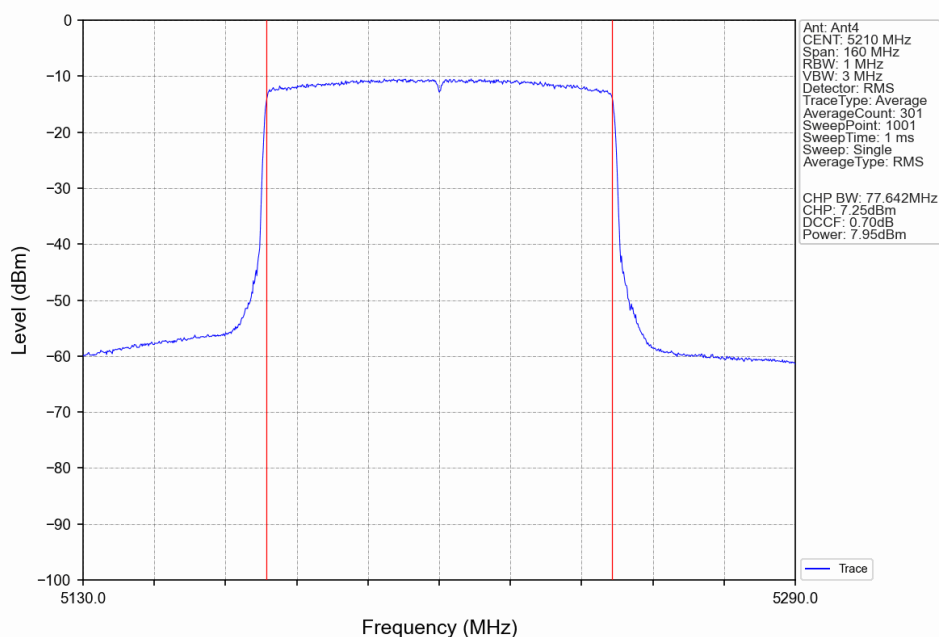
802.11ax(HEW80)_MCH_5210MHz_RU26_Mid_Ant4_NTNV
