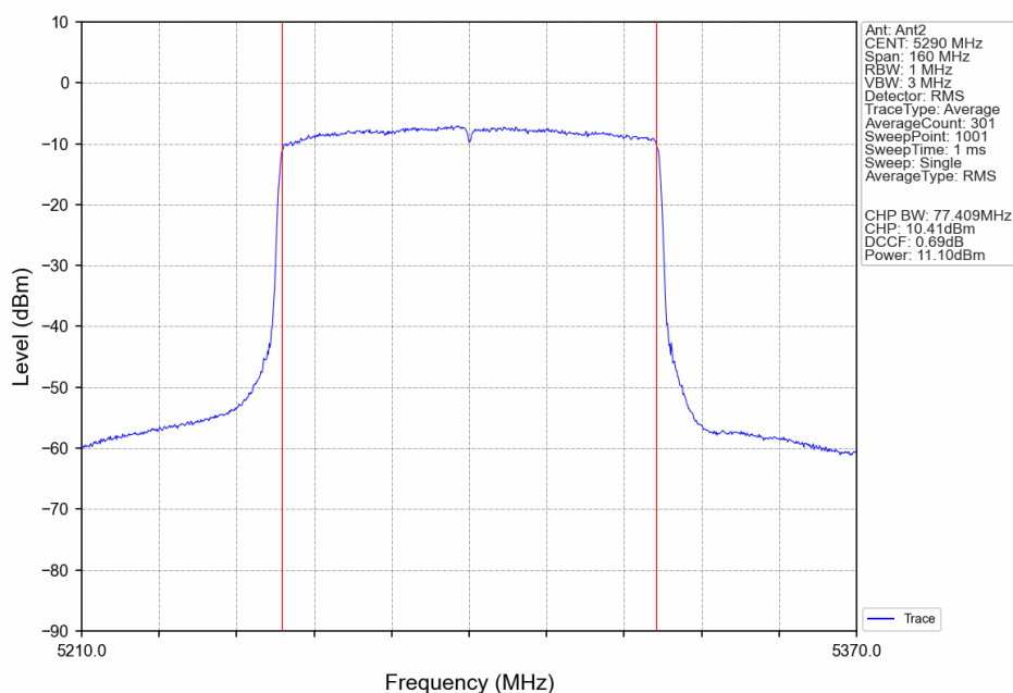
802.11ax(HEW80)_MCH_5290MHz_RU26_Mid_Ant2_NTNV
