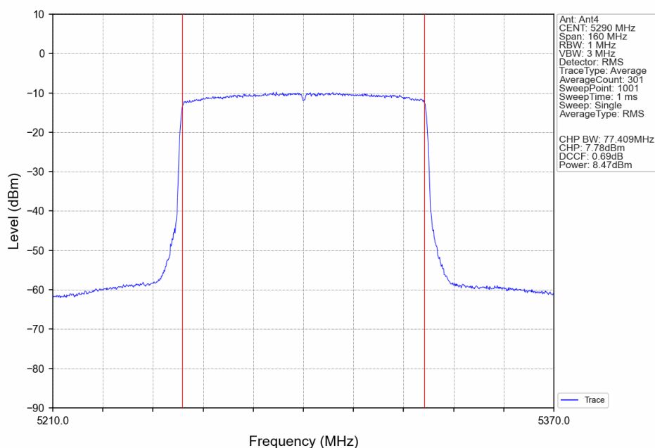
802.11ax(HEW80)_MCH_5290MHz_RU26_Mid_Ant4_NTNV
