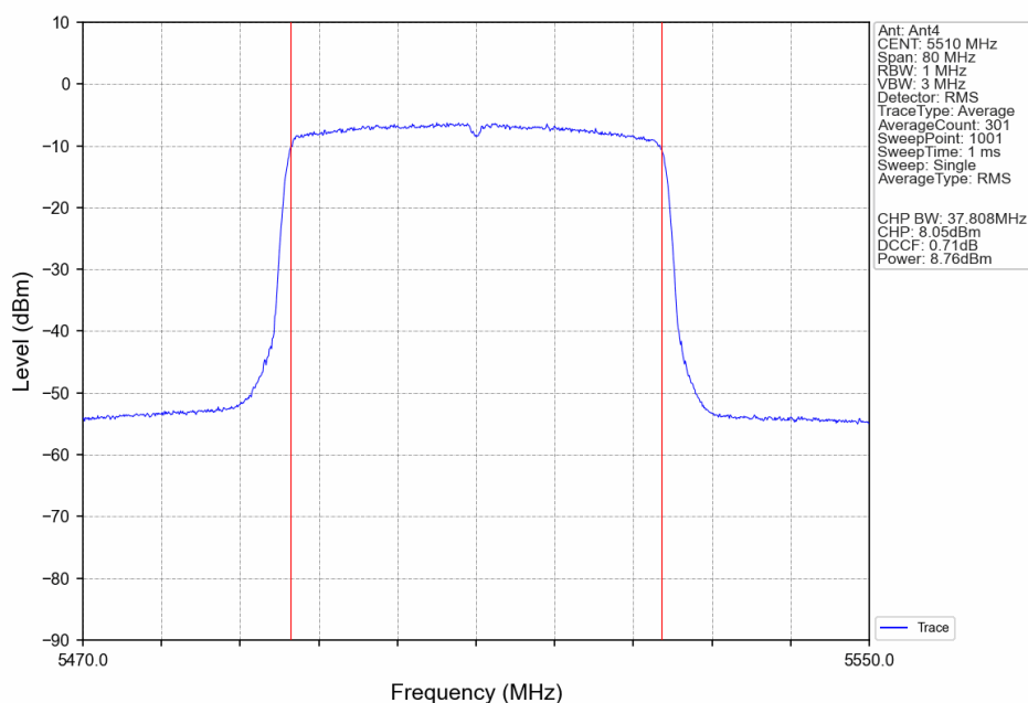
802.11ax(HEW40)_LCH_5510MHz_RU26_Mid_Ant4_NTNV
