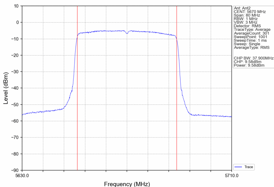
802.11ax(HEW40)_HCH_5670MHz_RU26_Left_Ant2_NTNV
