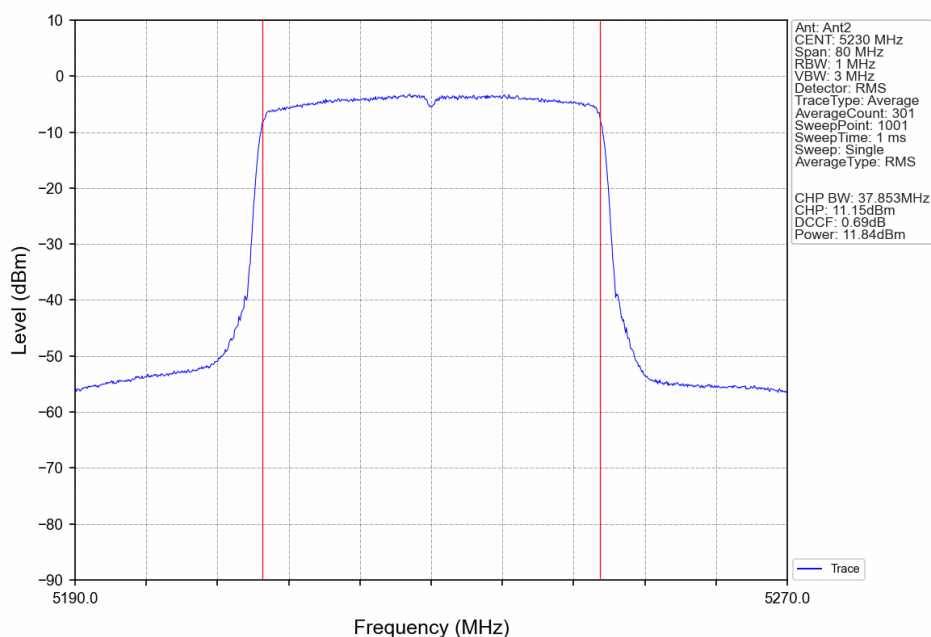
802.11ax(HEW40)_HCH_5230MHz_RU26_Mid_Ant2_NTNV
