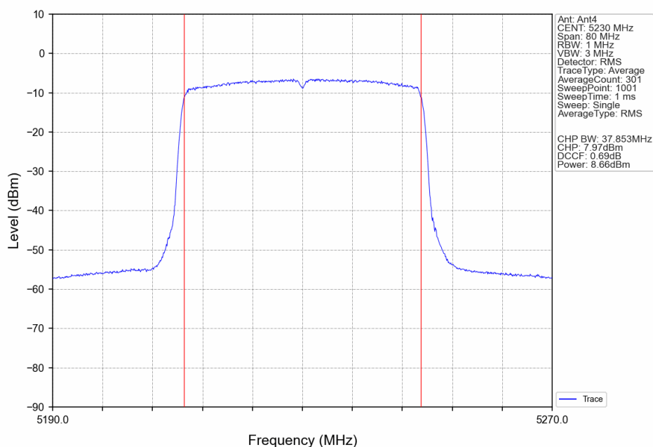
802.11ax(HEW40)_HCH_5230MHz_RU26_Mid_Ant4_NTNV
