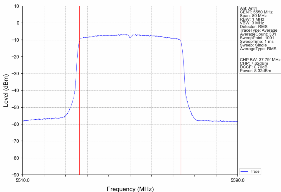
802.11ax(HEW40)_MCH_5550MHz_RU26_Right_Ant4_NTNV
