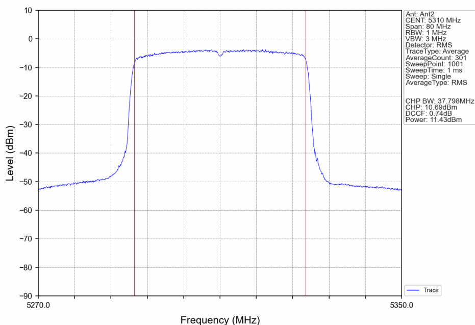
802.11ax(HEW40)_HCH_5310MHz_RU26_Right_Ant2_NTNV
