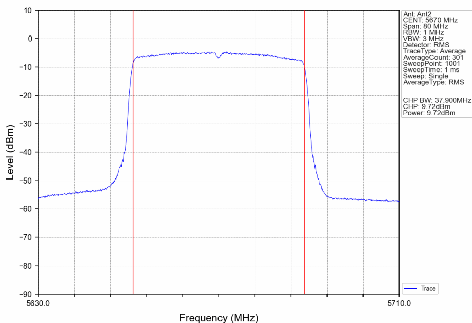
802.11ax(HEW40)_HCH_5670MHz_RU26_Right_Ant2_NTNV
