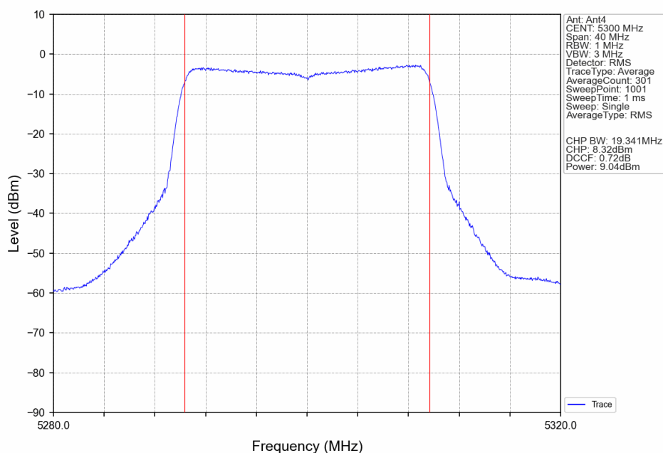
802.11ax(HEW20)_MCH_5300MHz_RU26_Mid_Ant4_NTNV
