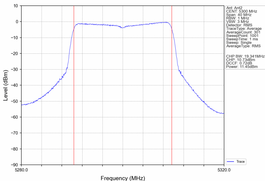
802.11ax(HEW20)_MCH_5300MHz_RU26_Mid_Ant2_NTNV
