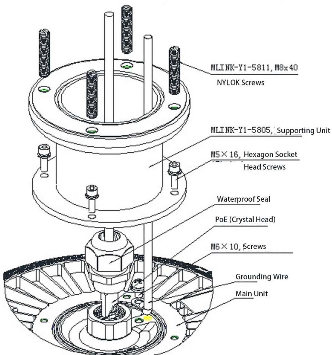
Details A, Scale 1:2
