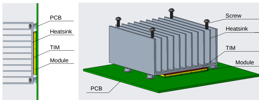
Figure 18: Placement and Fixing of the Heatsink
