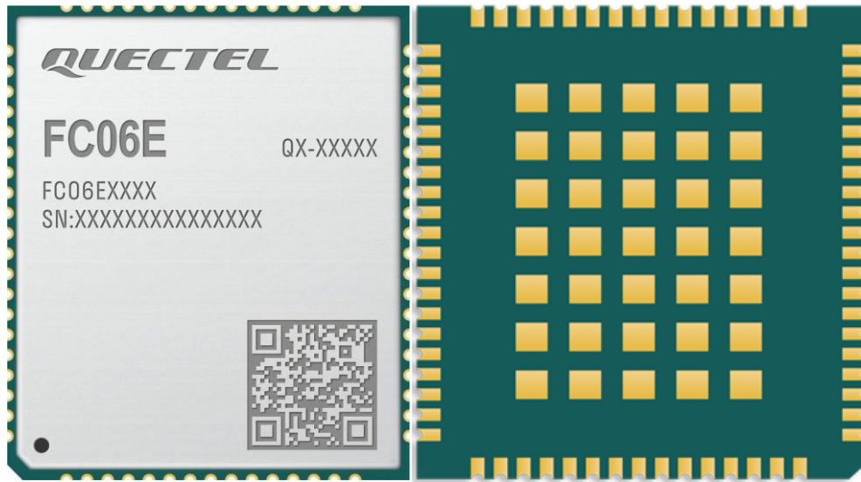
Figure 22: Top and Bottom Views of the Module
