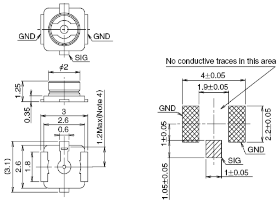
Figure 15: Dimensions of the Receptacle (Unit: mm)
