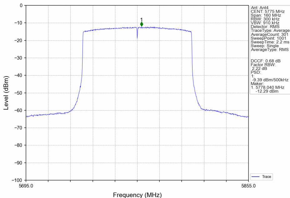
802.11ax(HEW80)_MCH_5775MHz_RU26_Right_MIMO_NTNV
