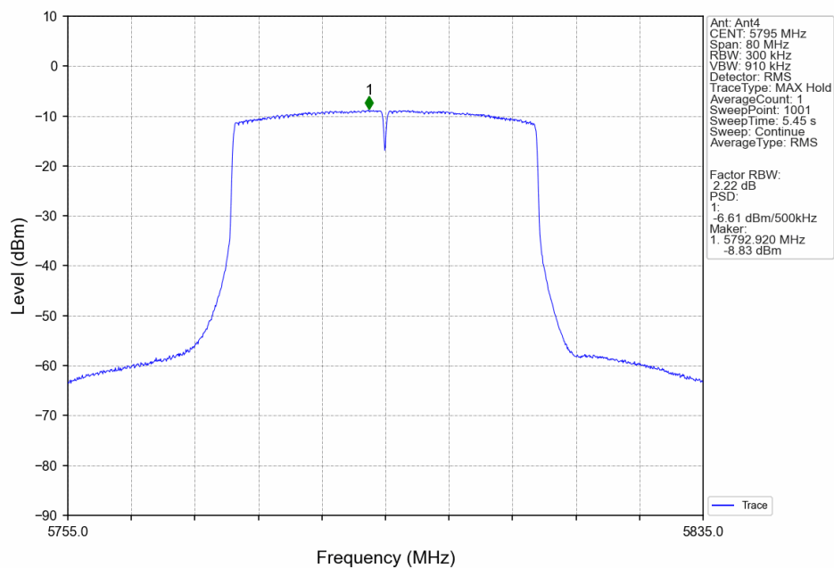
802.11ax(HEW40)_HCH_5795MHz_RU26_Mid_Ant4_NTNV
