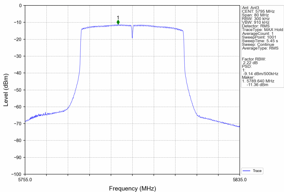
802.11ax(HEW40)_HCH_5795MHz_RU26_Left_Ant3_NTNV
