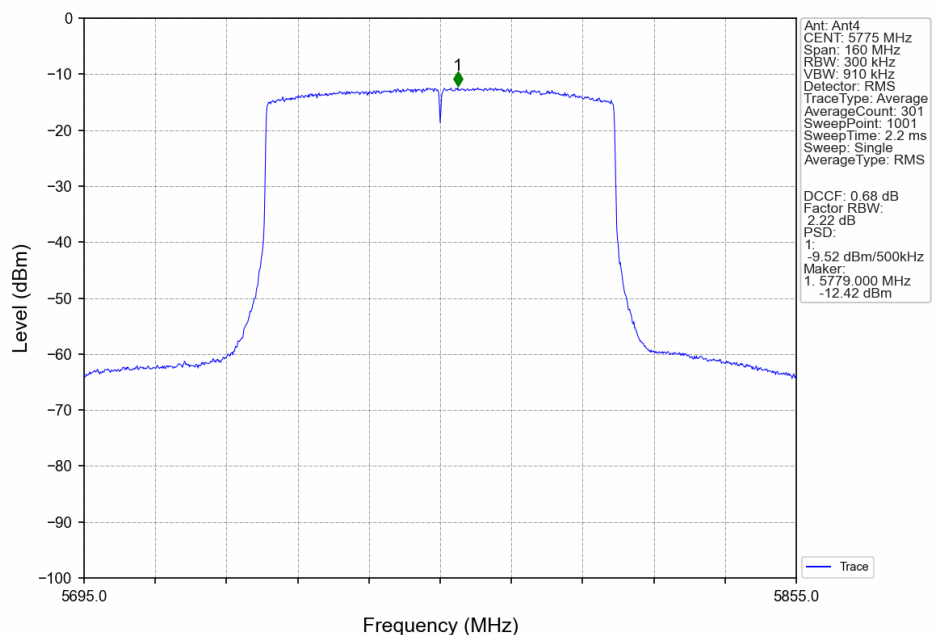
802.11ax(HEW80)_MCH_5775MHz_RU26_Mid_Ant4_NTNV
