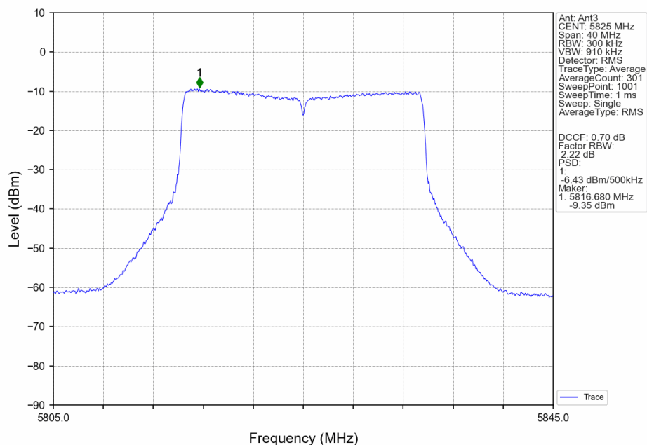
802.11ax(HEW20)_HCH_5825MHz_RU26_Right_Ant3_NTNV
