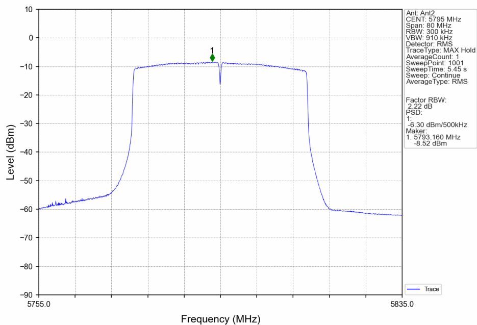
802.11ax(HEW40)_HCH_5795MHz_RU26_Mid_Ant2_NTNV
