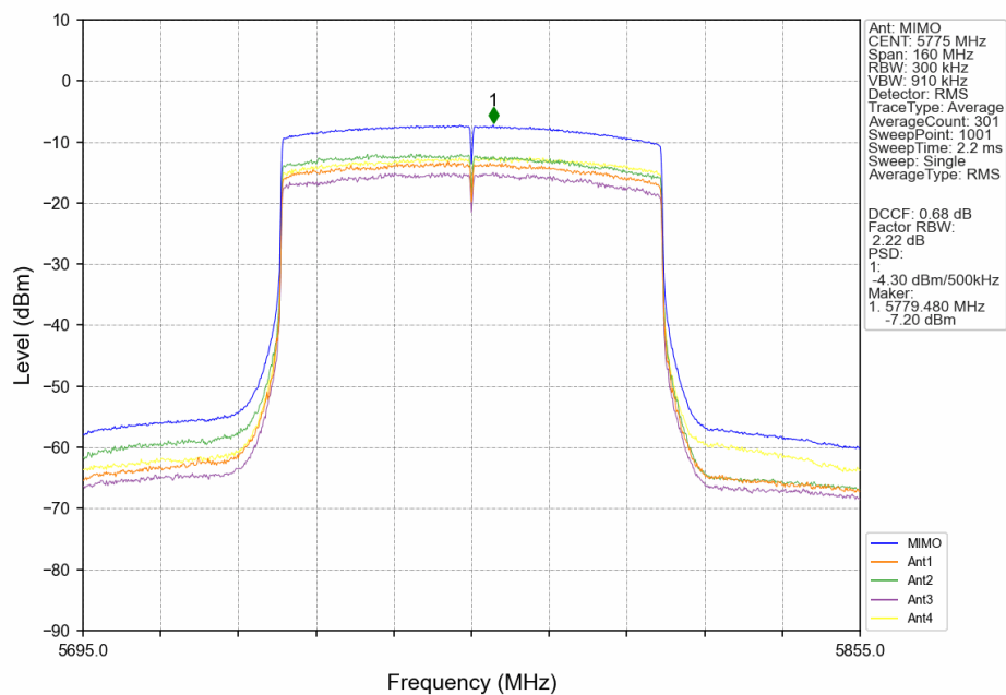
802.11ax(HEW80)_MCH_5775MHz_RU26_Left_MIMO_NTNV
