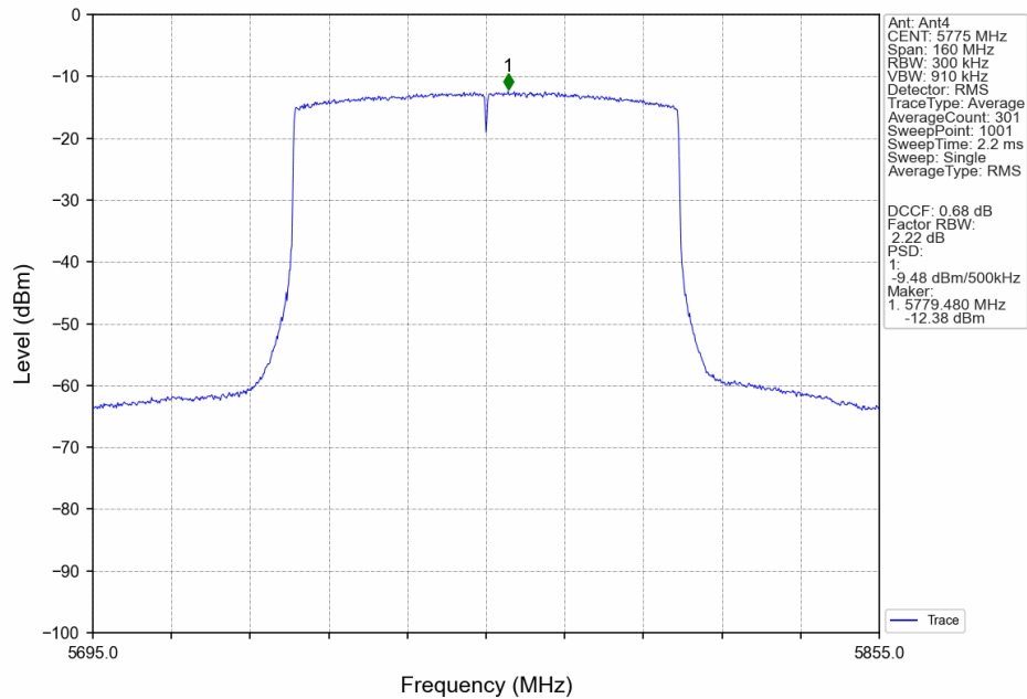
802.11ax(HEW80)_MCH_5775MHz_RU26_Left_MIMO_NTNV
