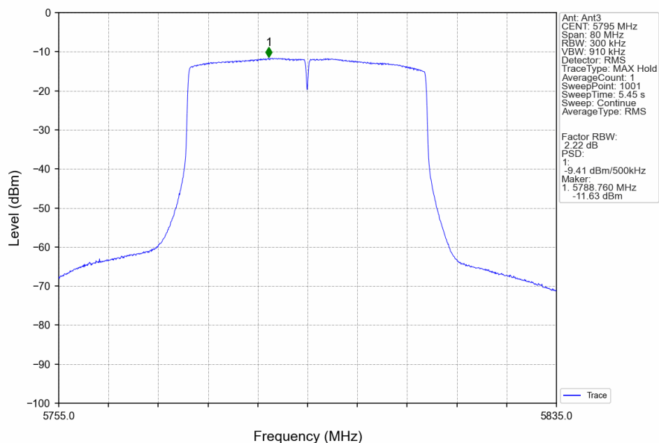
802.11ax(HEW40)_HCH_5795MHz_RU26_Right_Ant3_NTNV
