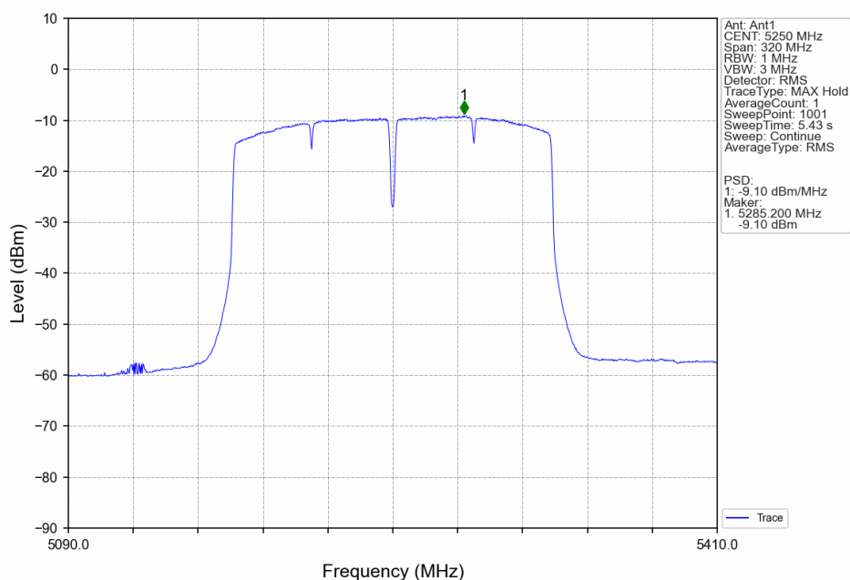
802.11ax(HEW160)_MCH_5250MHz_RU26_Mid_Ant1_NTNV
