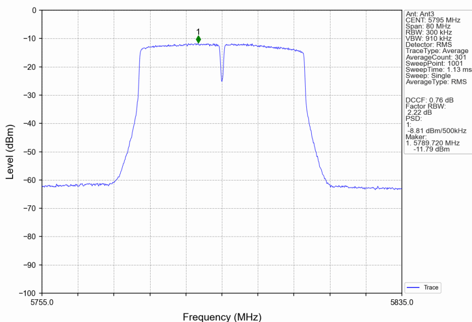
802.11n(HT40)_HCH_5795MHz_Ant3_NTNV
