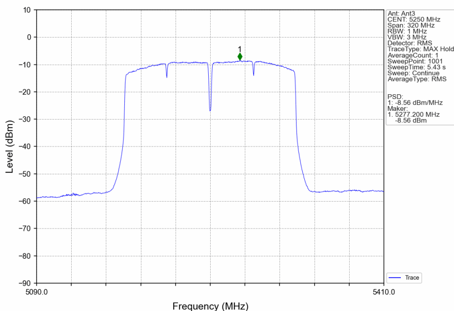
802.11ax(HEW160)_MCH_5250MHz_RU26_Mid_Ant3_NTNV
