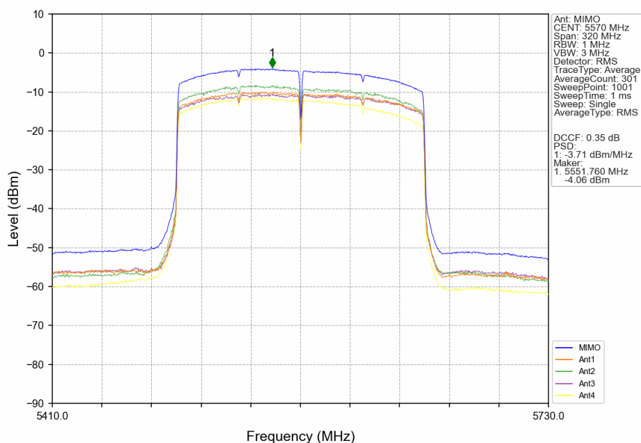
802.11ax(HEW160)_MCH_5570MHz_RU26_Mid_MIMO_NTNV
