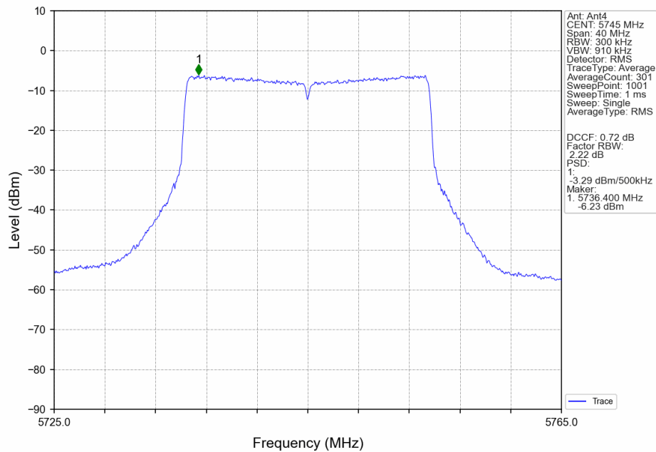
802.11ax(HEW20)_LCH_5745MHz_RU26_Left_MIMO_NTNV
