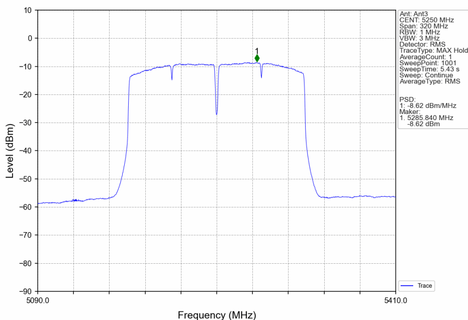
802.11ax(HEW160)_MCH_5250MHz_2xRU996_Left_Ant3_NTNV
