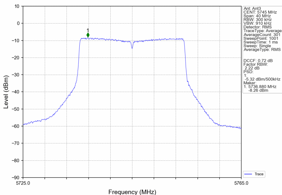
802.11ax(HEW20)_LCH_5745MHz_RU26_Left_Ant3_NTNV
