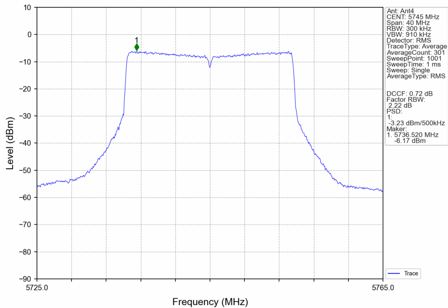
802.11ax(HEW20)_LCH_5745MHz_RU26_Right_MIMO_NTNV
