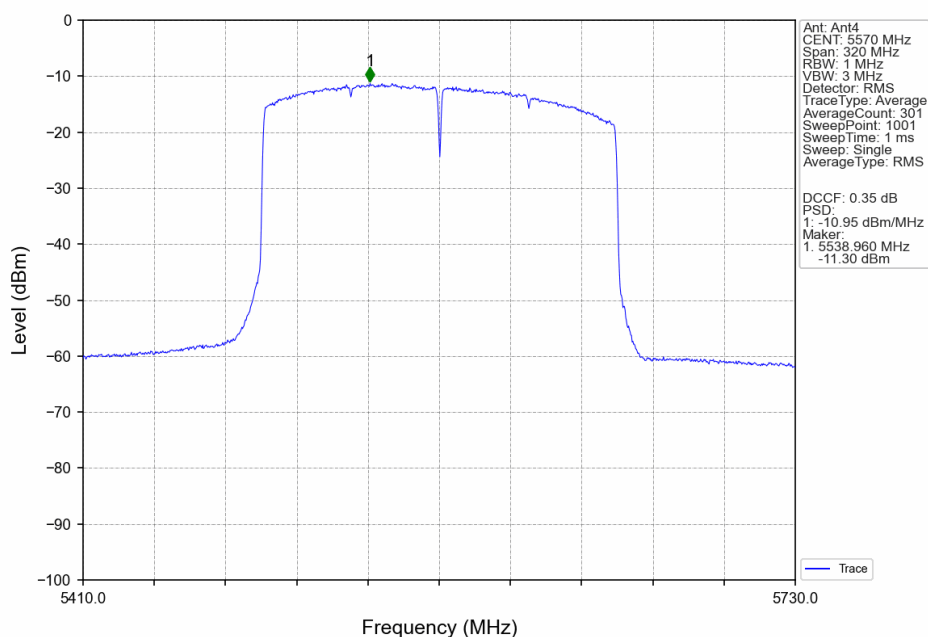
802.11ax(HEW160)_MCH_5570MHz_RU26_Left_Ant4_NTNV
