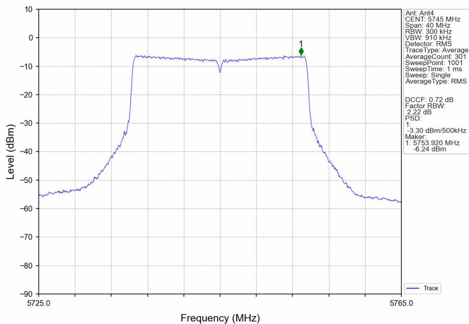
802.11ax(HEW20)_LCH_5745MHz_RU26_Mid_Ant4_NTNV
