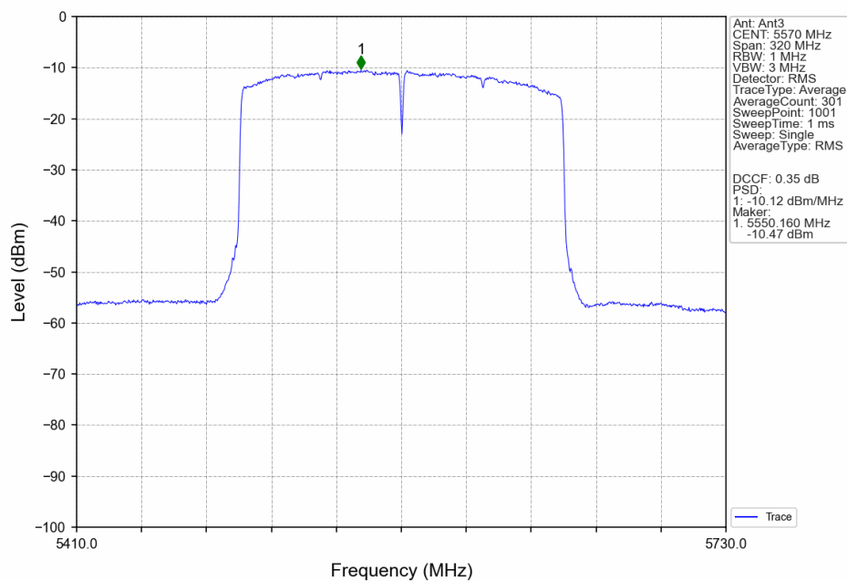
802.11ax(HEW160)_MCH_5570MHz_2xRU996_Left_Ant3_NTNV
