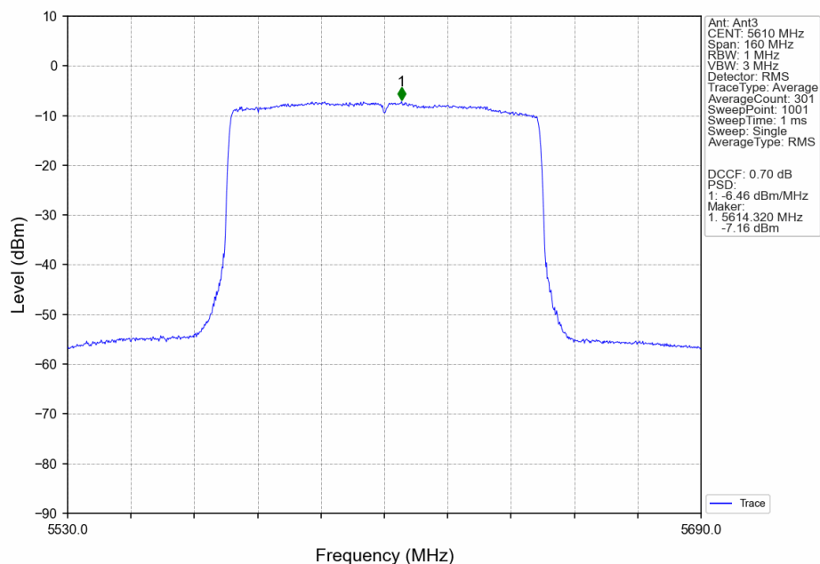
802.11ax(HEW80)_HCH_5610MHz_RU26_Mid_Ant3_NTNV
