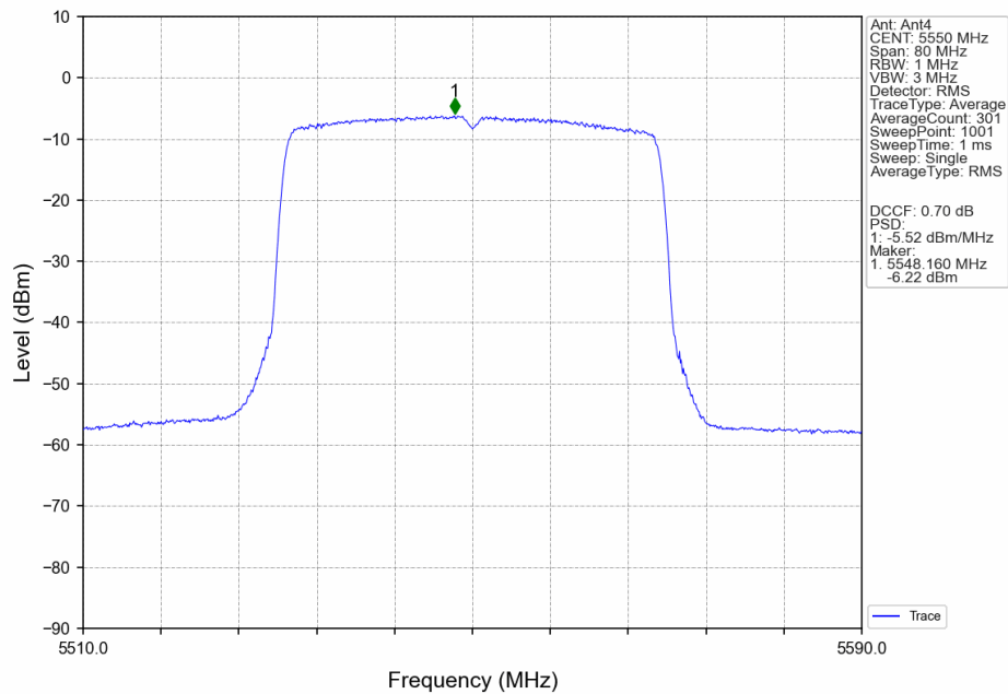
802.11ax(HEW40)_MCH_5550MHz_RU484_Left_MIMO_NTNV
