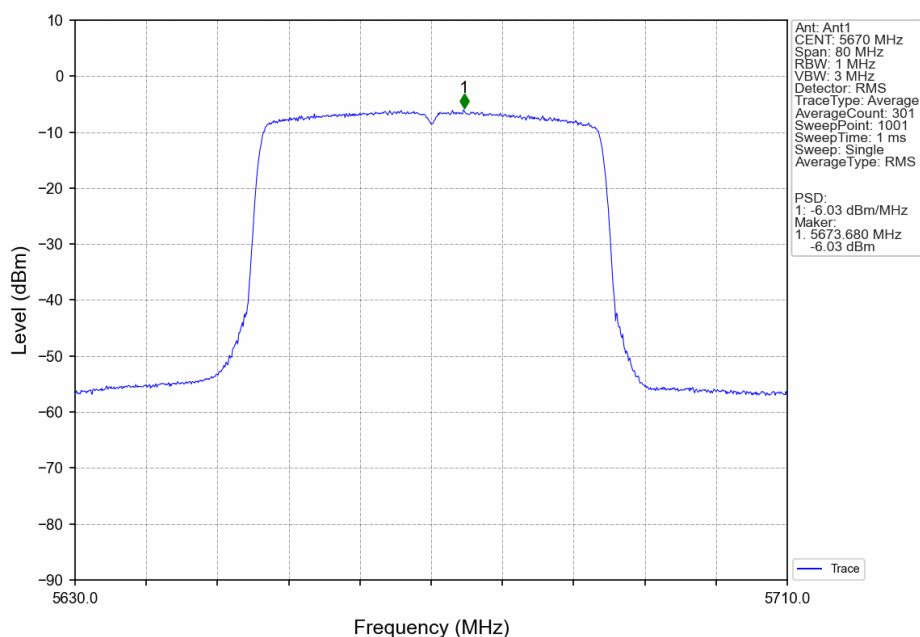
802.11ax(HEW40)_HCH_5670MHz_RU26_Mid_Ant1_NTNV
