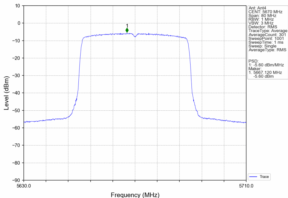
802.11ax(HEW40)_HCH_5670MHz_RU26_Left_Ant4_NTNV
