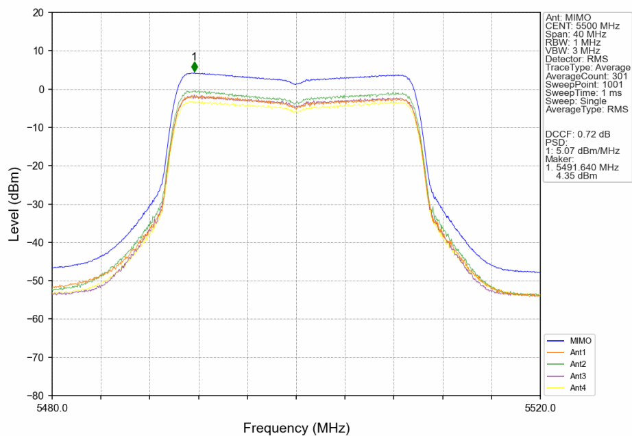
802.11ax(HEW20)_LCH_5500MHz_RU26_Mid_MIMO_NTNV
