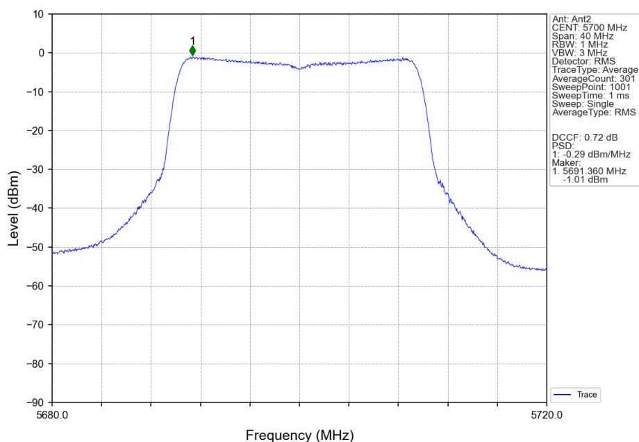
802.11ax(HEW20)_HCH_5700MHz_RU26_Right_Ant2_NTNV
