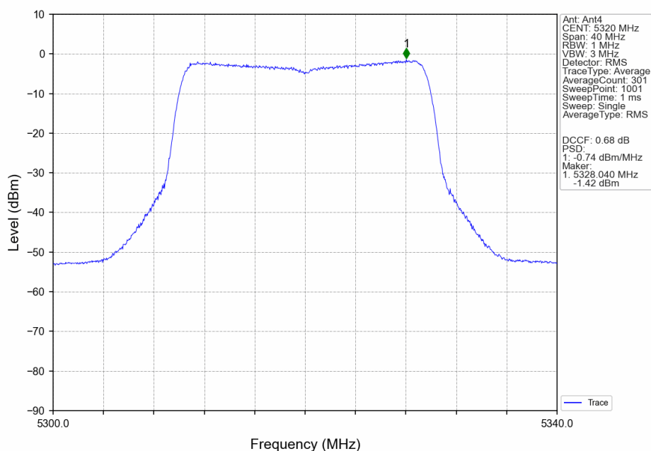
802.11ax(HEW20)_HCH_5320MHz_RU26_Right_Ant4_NTNV
