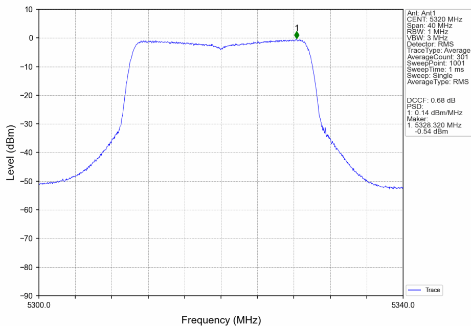
802.11ax(HEW20)_HCH_5320MHz_RU26_Mid_Ant1_NTNV
