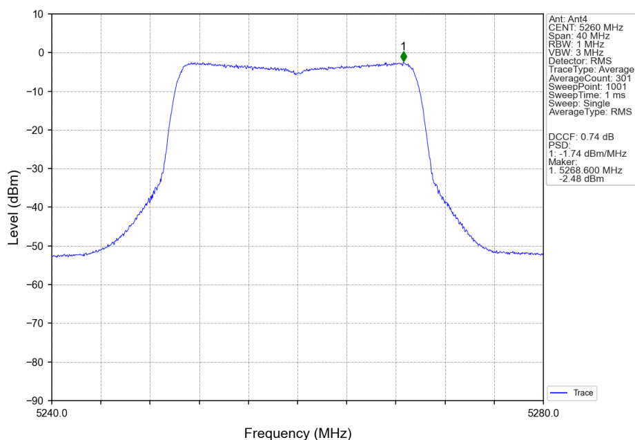
802.11ax(HEW20)_LCH_5260MHz_RU26_Right_Ant4_NTNV
