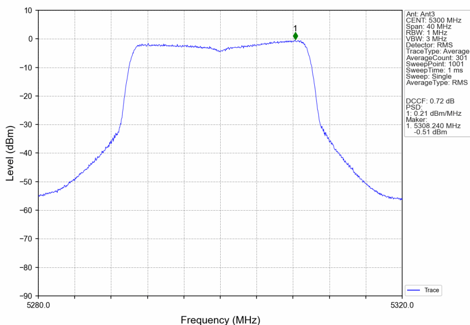
802.11ax(HEW20)_MCH_5300MHz_RU26_Mid_Ant3_NTNV
