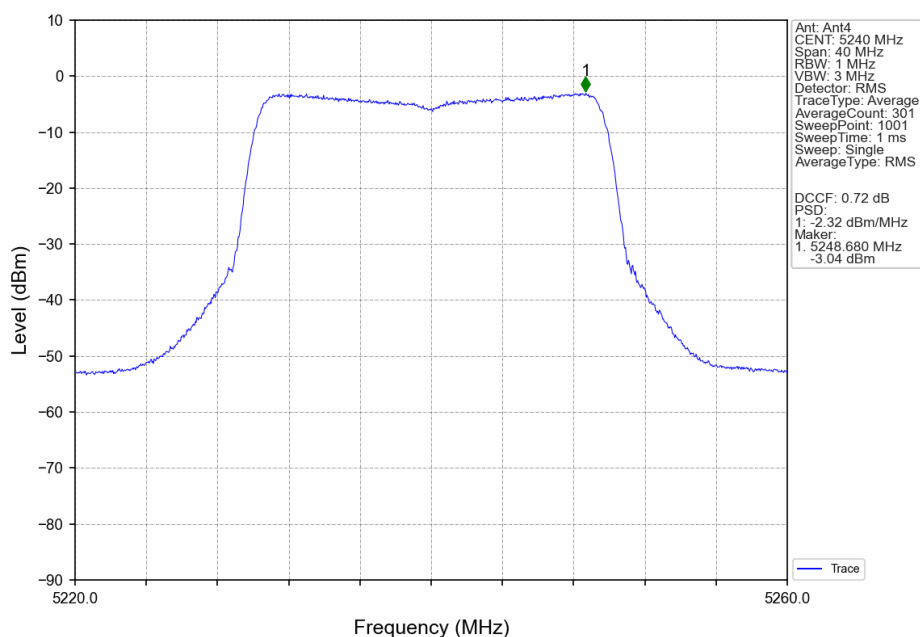
802.11ax(HEW20)_HCH_5240MHz_RU26_Right_Ant4_NTNV
