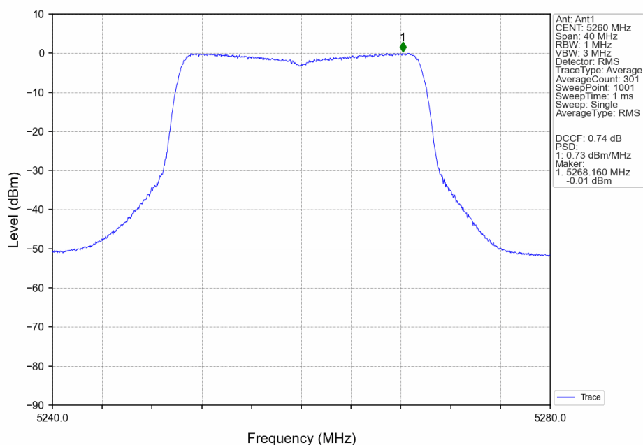
802.11ax(HEW20)_LCH_5260MHz_RU26_Mid_Ant1_NTNV
