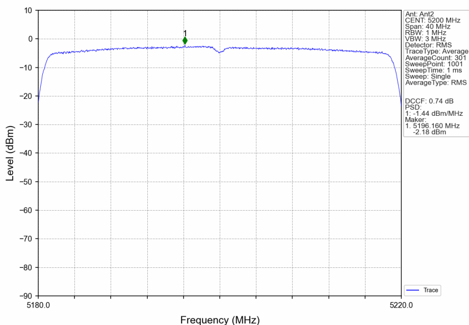
802.11ax(HEW20)_MCH_5200MHz_RU26_Right_Ant2_NTNV
