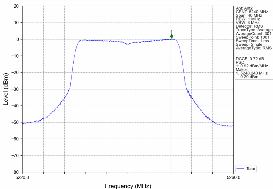
802.11ax(HEW20)_HCH_5240MHz_RU26_Left_Ant2_NTNV
