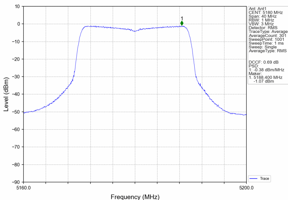
802.11ax(HEW20)_LCH_5180MHz_RU26_Right_Ant1_NTNV
