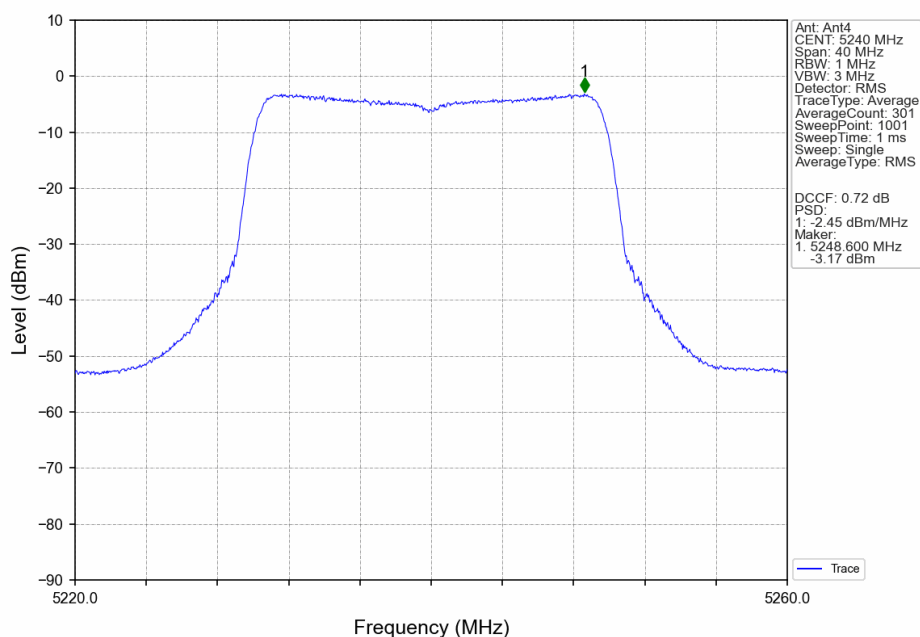
802.11ax(HEW20)_HCH_5240MHz_RU26_Left_Ant4_NTNV
