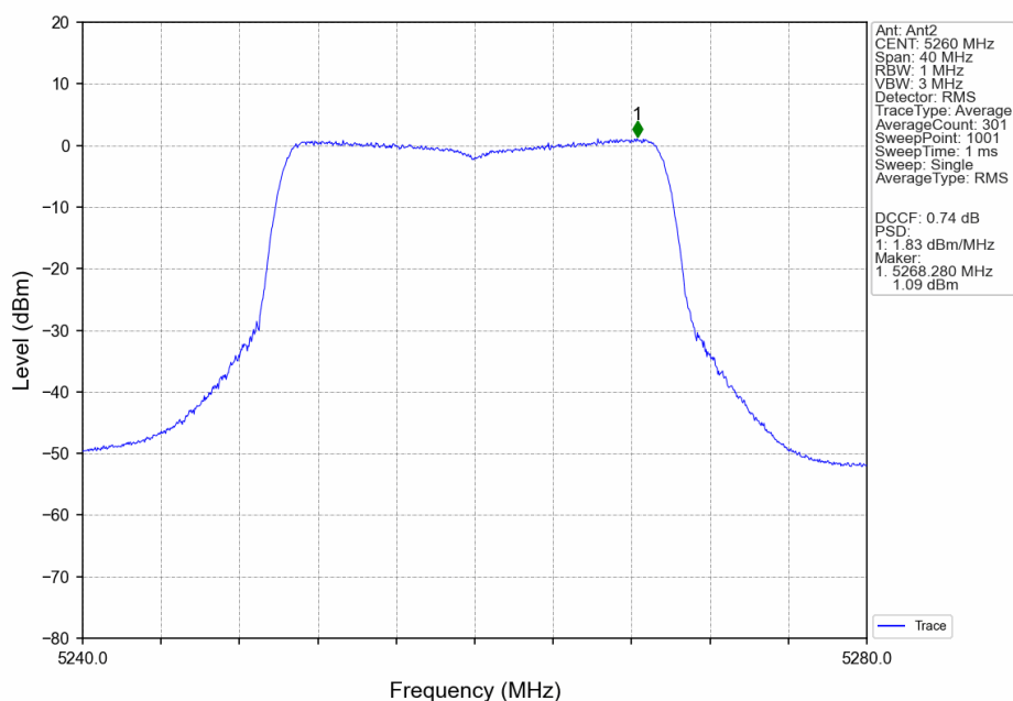
802.11ax(HEW20)_LCH_5260MHz_RU26_Right_Ant2_NTNV
