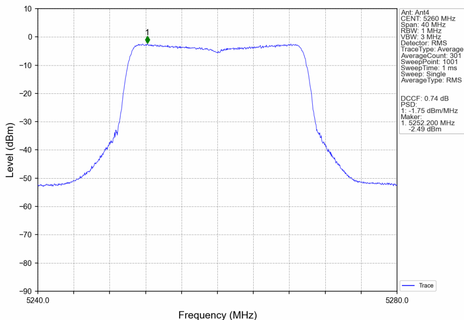
802.11ax(HEW20)_LCH_5260MHz_RU26_Mid_MIMO_NTNV
