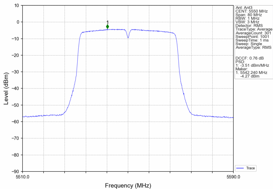
802.11n(HT40)_MCH_5550MHz_Ant3_NTNV
