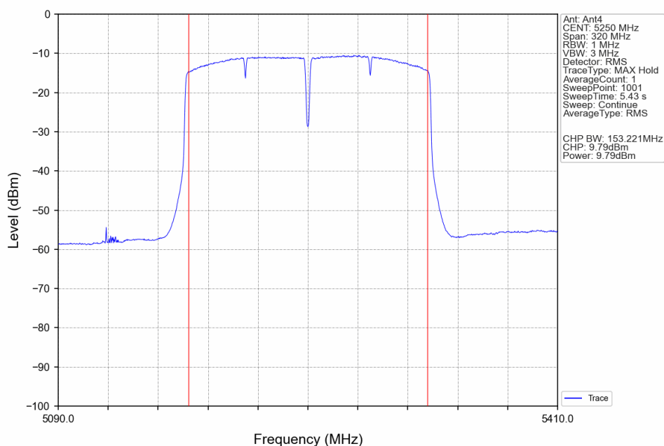
802.11ax(HEW160)_MCH_5250MHz_2xRU996_Left_Ant4_NTNV
