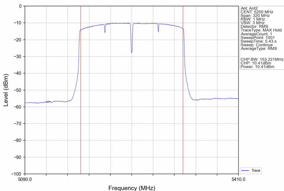
802.11ax(HEW160)_MCH_5250MHz_RU26_Mid_Ant2_NTNV
