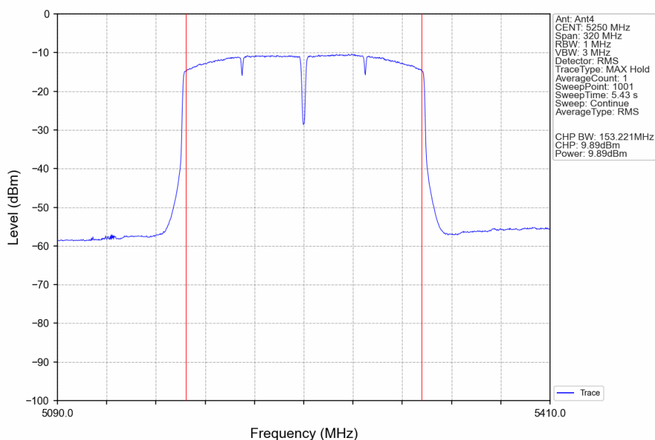
802.11ax(HEW160)_MCH_5250MHz_RU26_Mid_Ant4_NTNV
