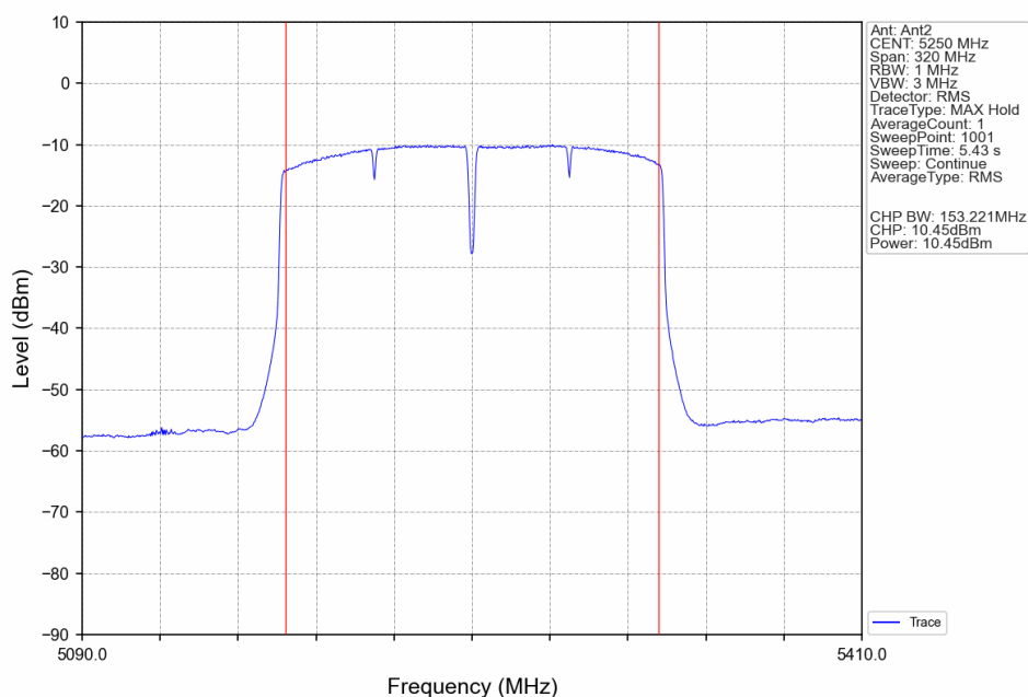
802.11ax(HEW160)_MCH_5250MHz_RU26_Right_Ant2_NTNV
