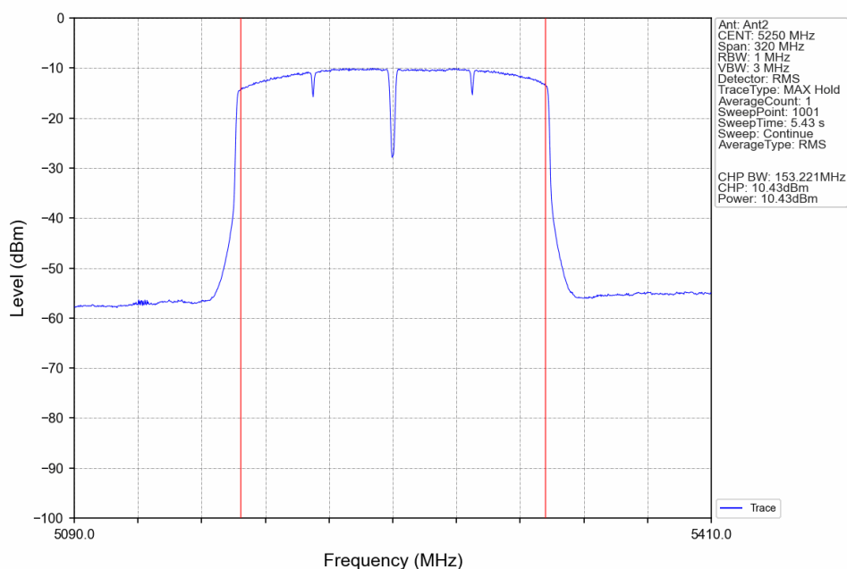
802.11ax(HEW160)_MCH_5250MHz_RU26_Left_Ant2_NTNV
