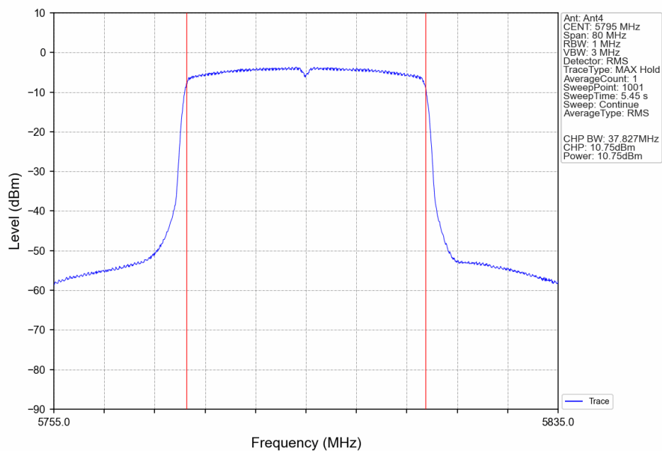
802.11ax(HEW40)_HCH_5795MHz_RU26_Right_Ant4_NTNV
