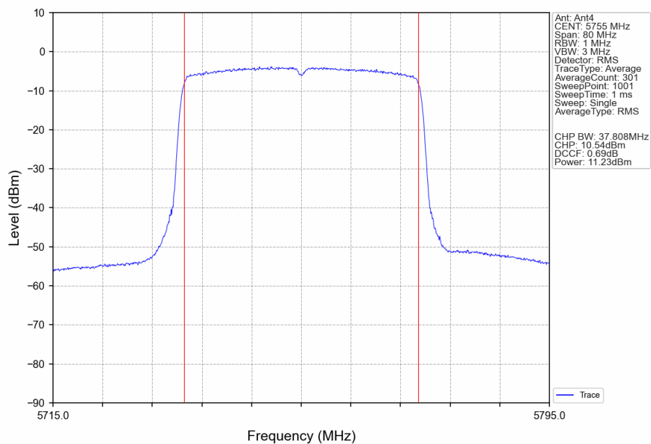
802.11ax(HEW40)_LCH_5755MHz_RU26_Mid_Ant4_NTNV
