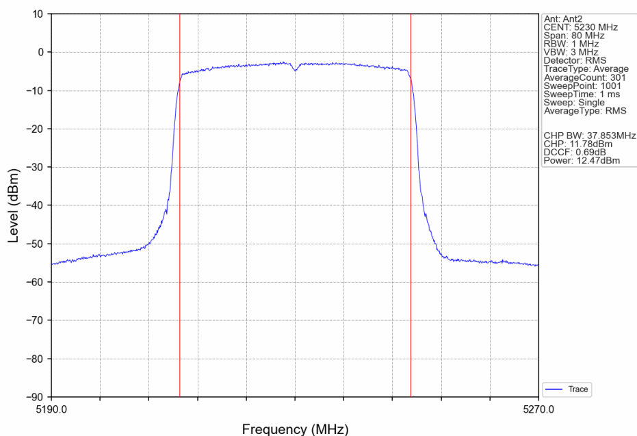
802.11ax(HEW40)_HCH_5230MHz_RU26_Right_Ant2_NTNV
