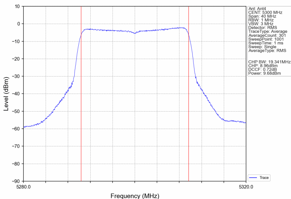
802.11ax(HEW20)_MCH_5300MHz_RU242_Left_Ant4_NTNV
