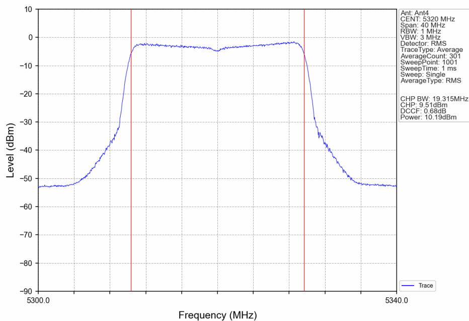
802.11ax(HEW20)_HCH_5320MHz_RU26_Mid_Ant4_NTNV
