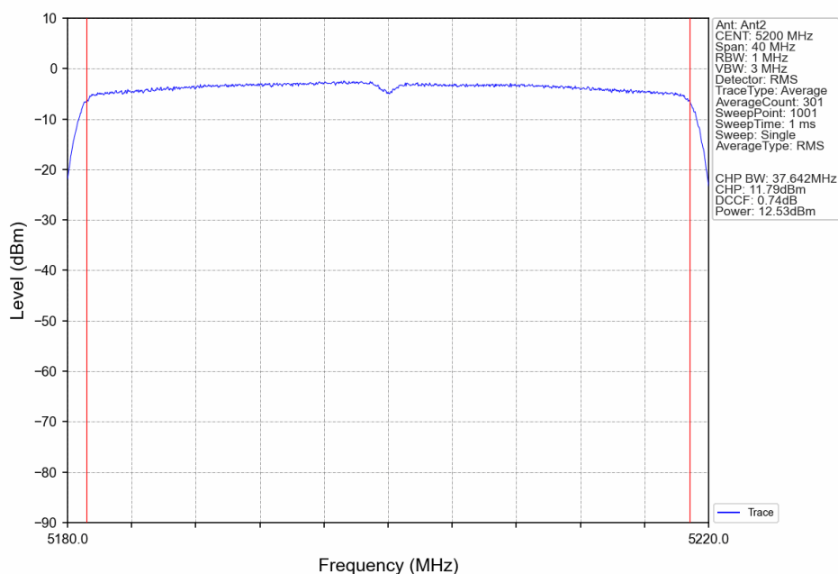
802.11ax(HEW20)_MCH_5200MHz_RU26_Left_Ant2_NTNV
