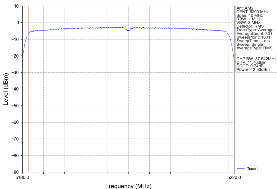
802.11ax(HEW20)_MCH_5200MHz_RU26_Right_Ant2_NTNV
