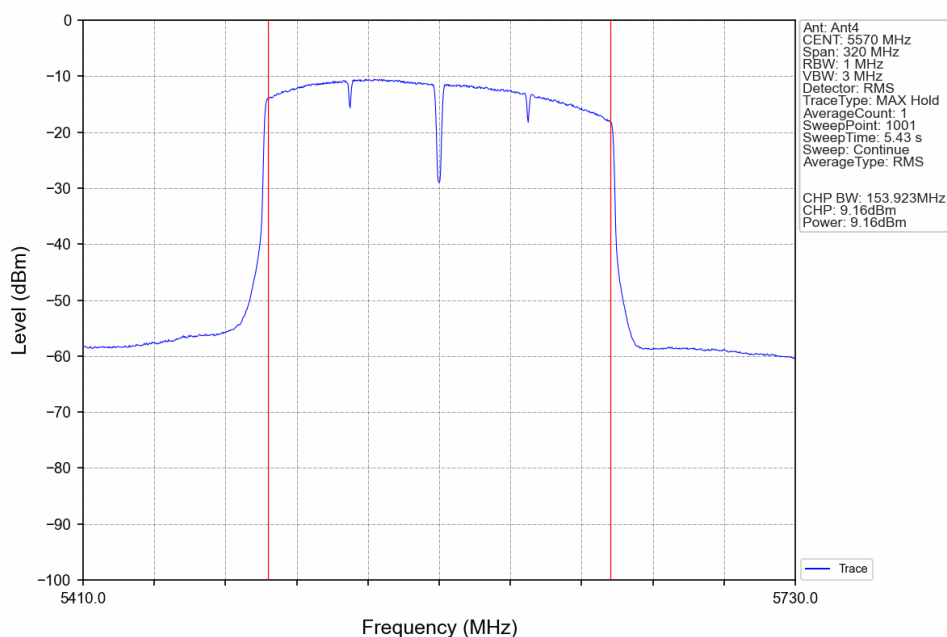
802.11ac(VHT160)_MCH_5570MHz_Ant4_NTNV
