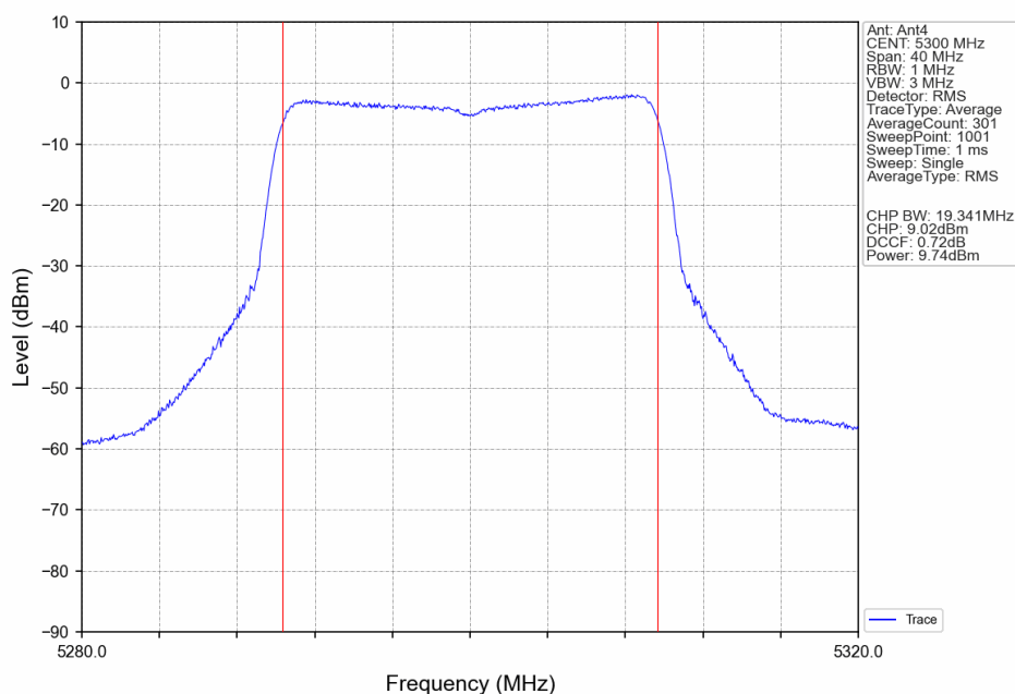
802.11ax(HEW20)_MCH_5300MHz_RU26_Left_Ant4_NTNV
