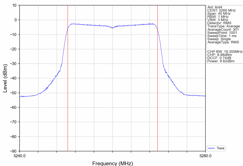
802.11ax(HEW20)_LCH_5260MHz_RU26_Right_Ant4_NTNV
