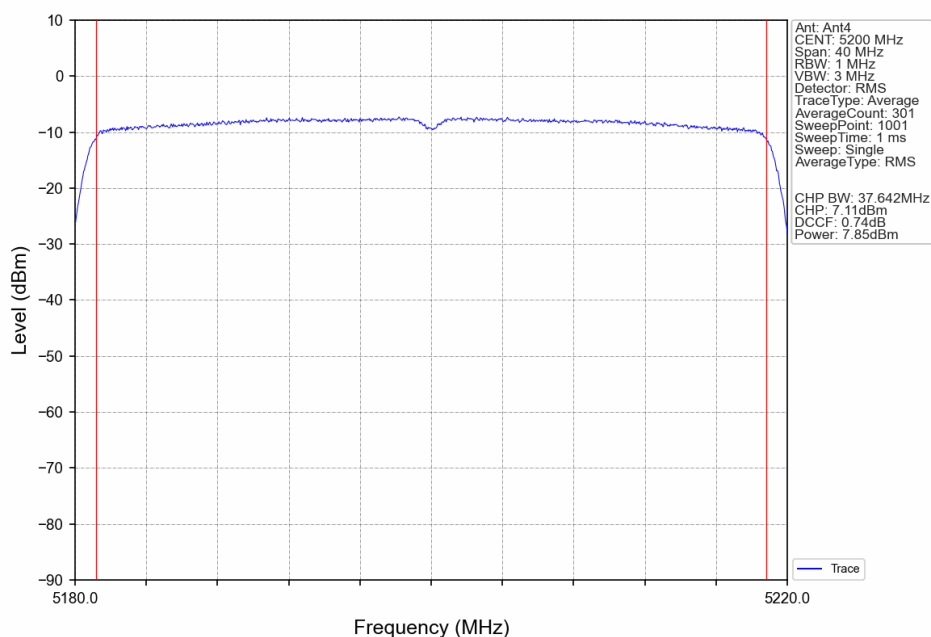
802.11ax(HEW20)_MCH_5200MHz_RU26_Left_Ant4_NTNV
