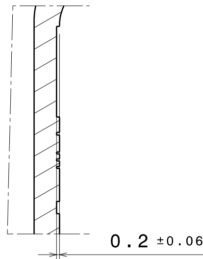
Section cut V-V 4:1
