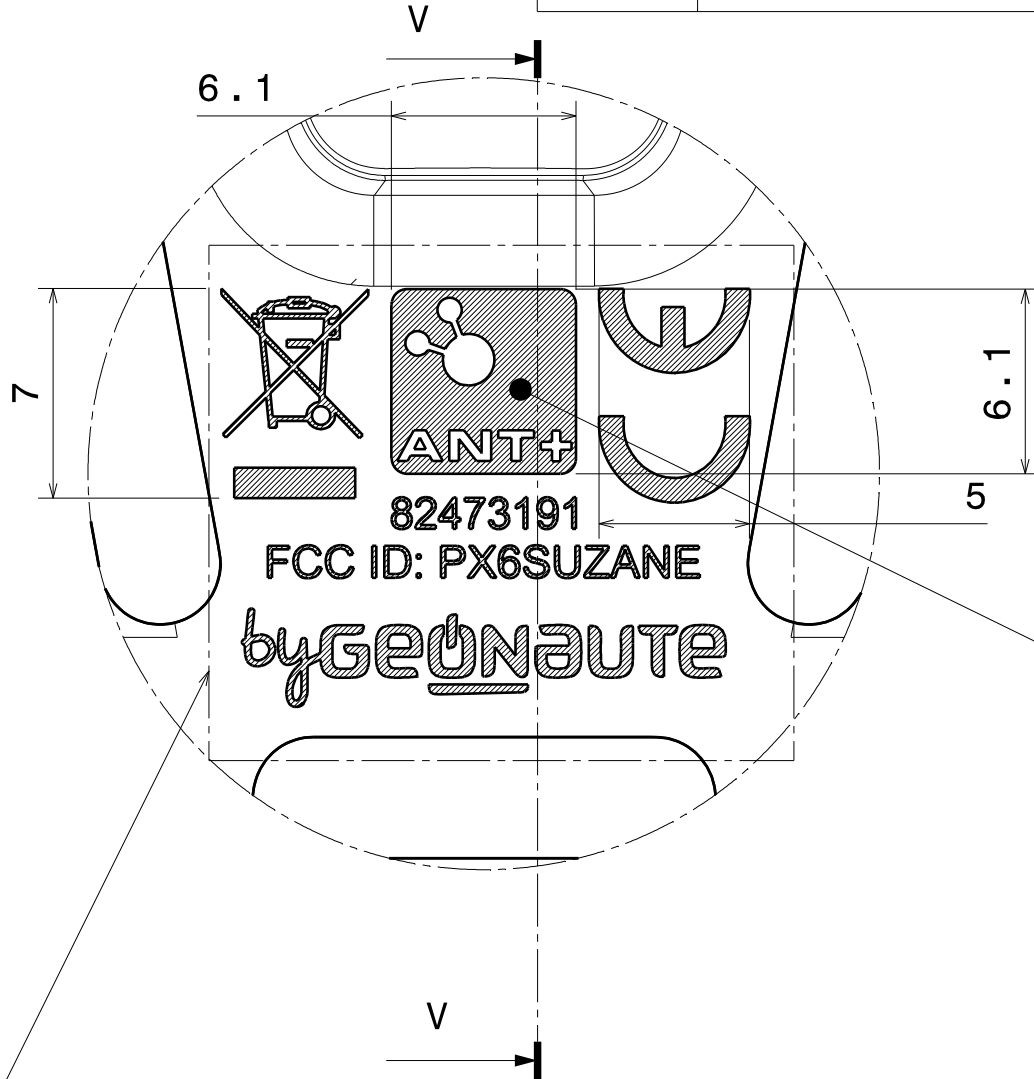
Detail U 4:1
