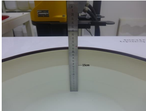
Photo 1: Tissue Simulant Liquid for Head 450MHz
