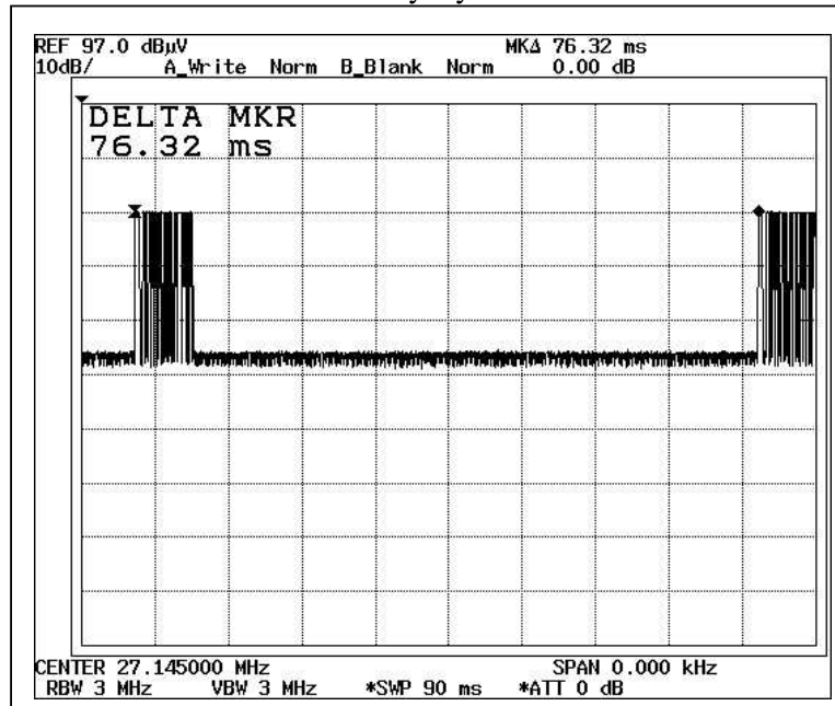
Duty Cycle
