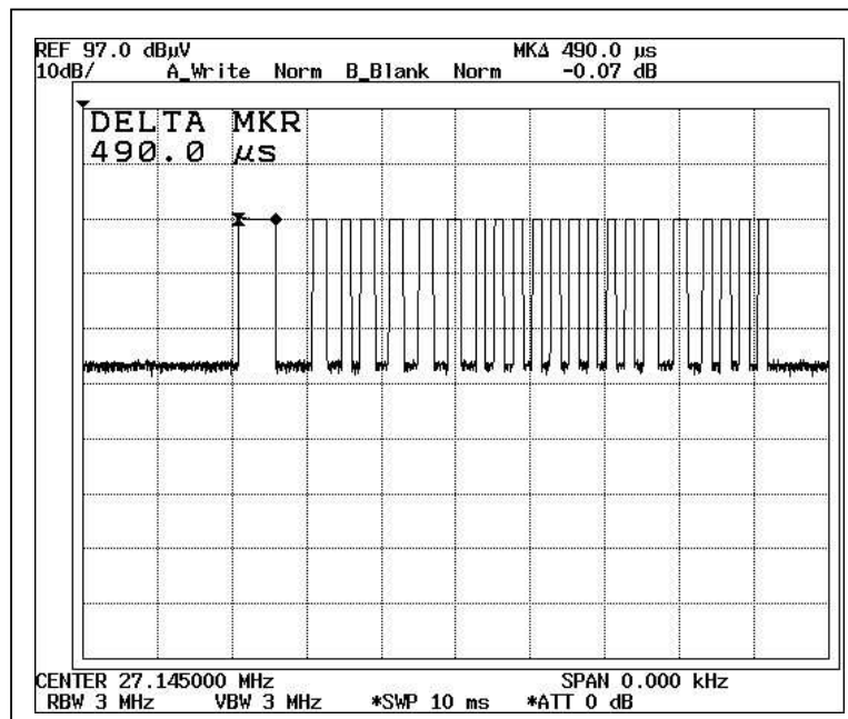
Duty Cycle 2
