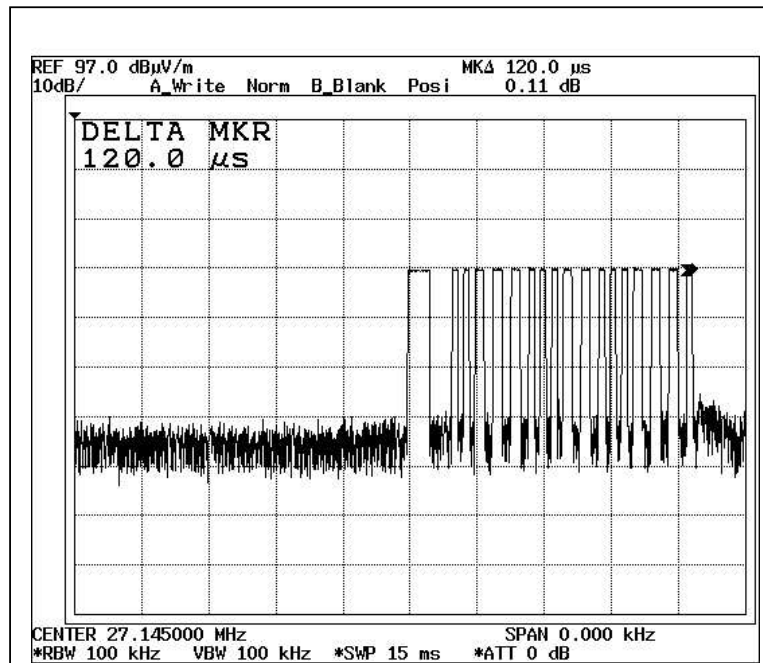
Duty Cycle 3
