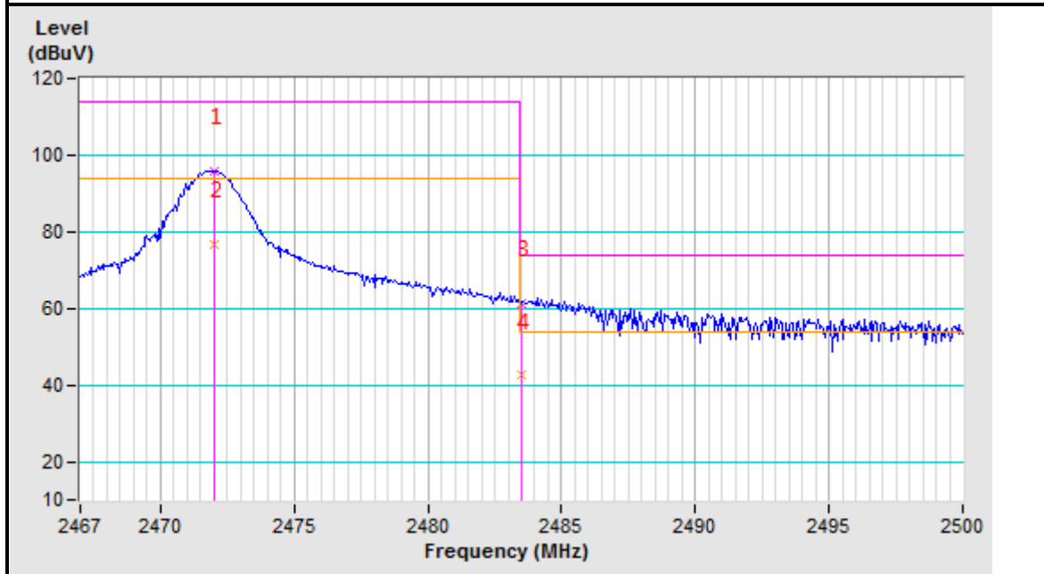
2472MHz Vertical
