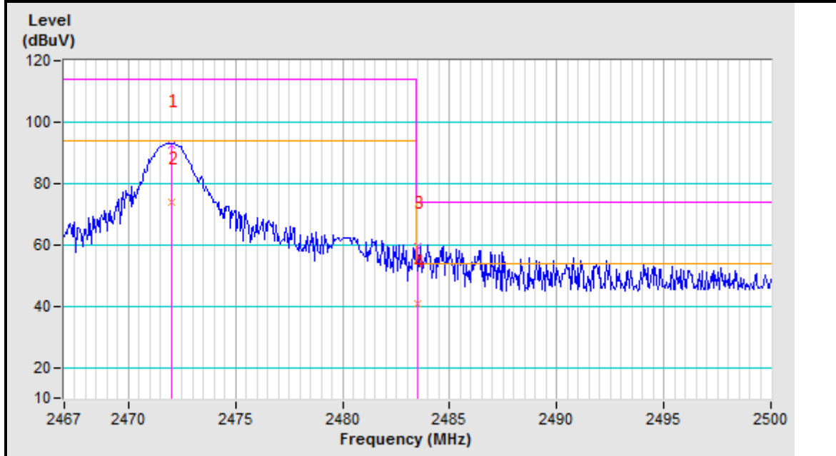
2472MHz Vertical
