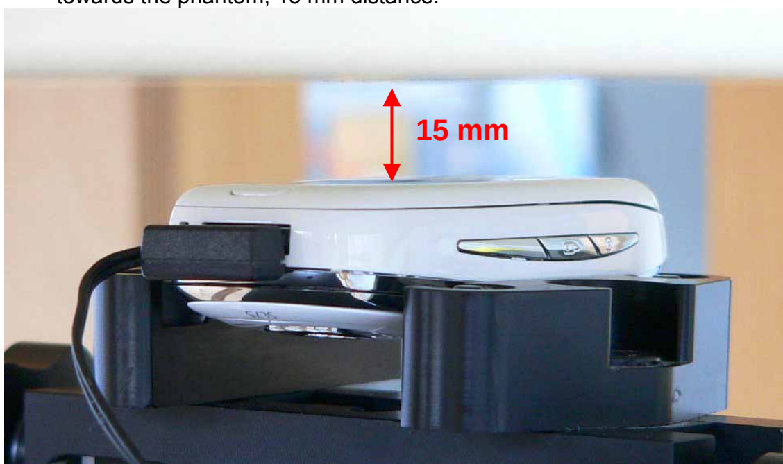
Fig. 36: Body worn configuration, GSM with headset, slider down, antenna towards the phantom, 15 mm distance.
