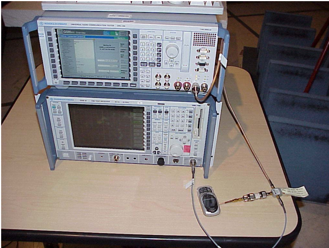
Test setup for Mobile Emissions in base band for SL56
