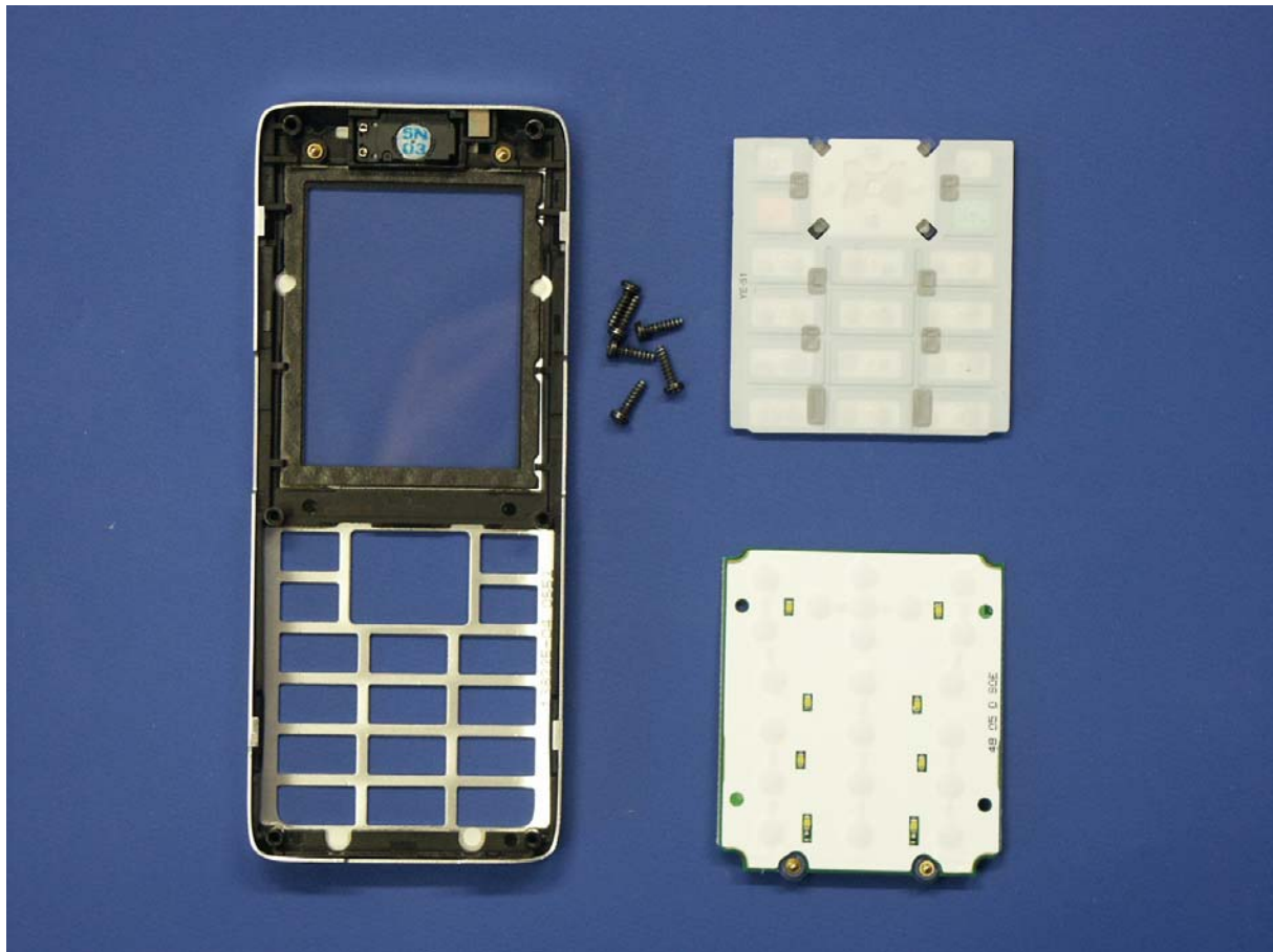
S68 MMI removed
