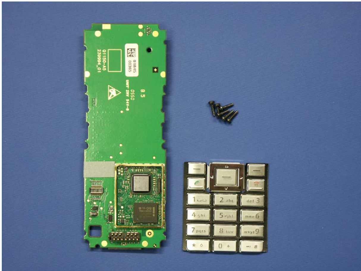
S68 PCB front view with removed shielding lids
