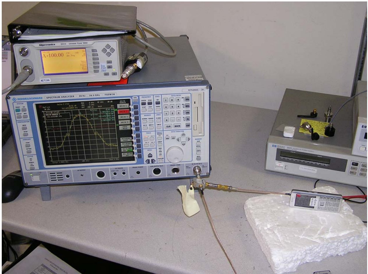
ANTENNA PORT CONDUCTED GSM
