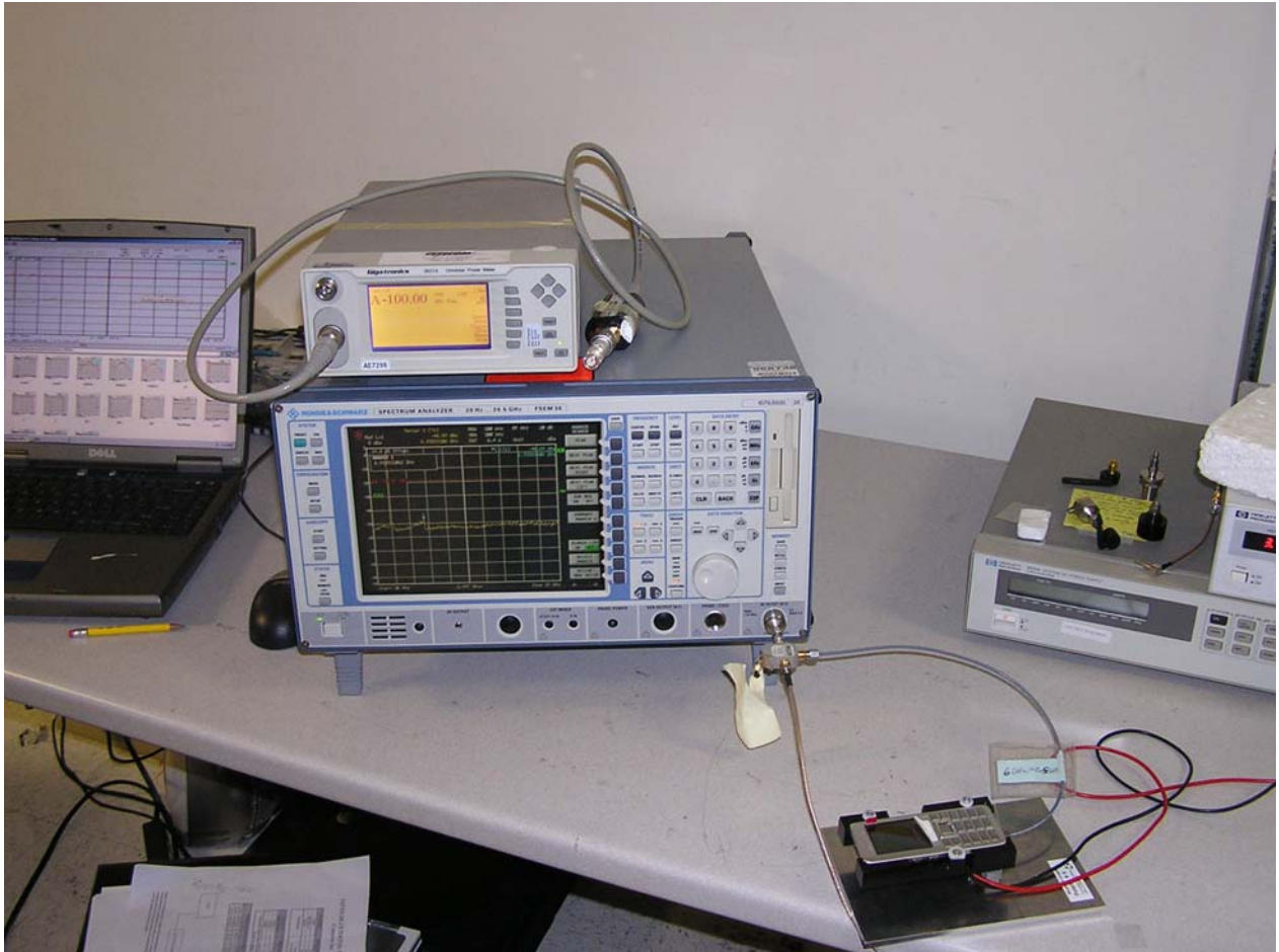
ANTENNA PORT CONDUCTED BLUETOOTH
