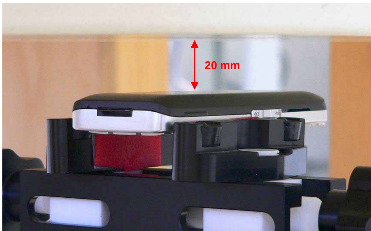
Fig. 24: Body worn configuration, GSM without accessory, antenna towards the phantom.
