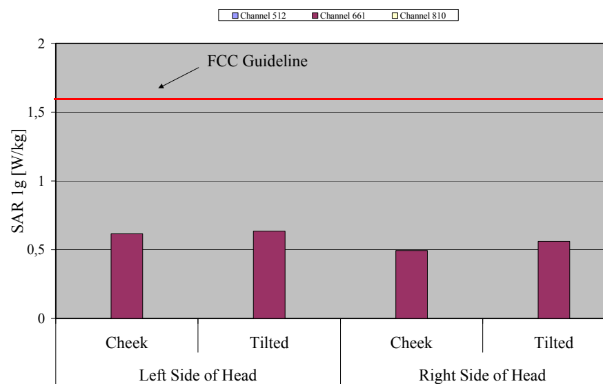
Fig. 11: The measured head phantom SAR values for the Siemens CX70 ARC for PCS 1900 in comparison to the FCC exposure limit.
