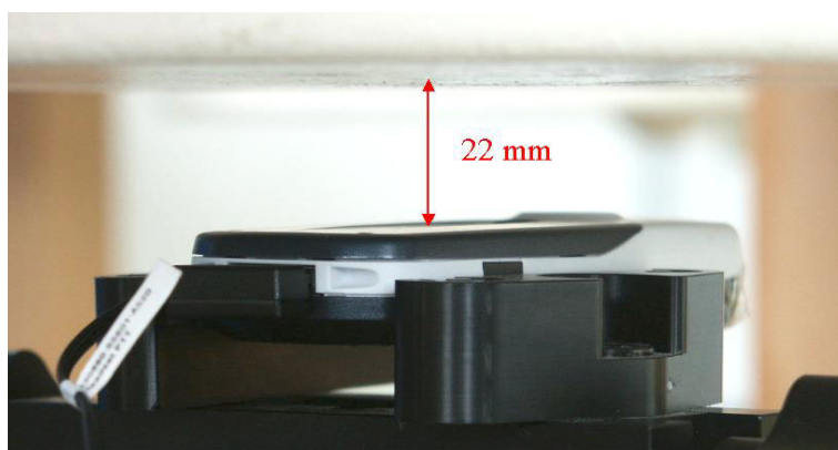
Fig. 64: Body worn configuration Standard, GSM mode (1 TX slot) with headset, antenna towards the phantom.
