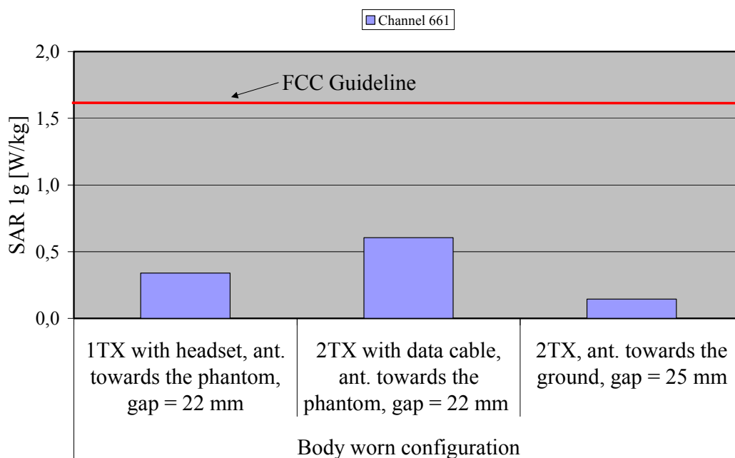
Fig. 16: The measured SAR values in body-worn configuration for the Siemens CX70 Standard for PCS 1900 in comparison to the FCC exposure limit.
