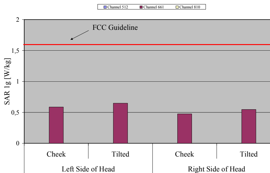
Fig. 9: The measured head phantom SAR values for the Siemens CX70 BF for PCS 1900 in comparison to the FCC exposure limit.
