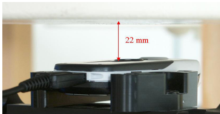
Fig. 71: Body worn configuration CX70 ARC, GPRS mode (2 TX slots) with data cable, antenna towards the phantom
