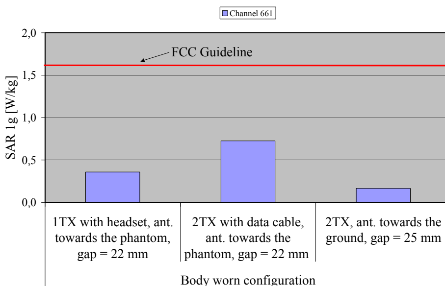
Fig. 19: The measured SAR values in body-worn configuration for the Siemens CX70 ARC for PCS 1900 in comparison to the FCC exposure limit.
