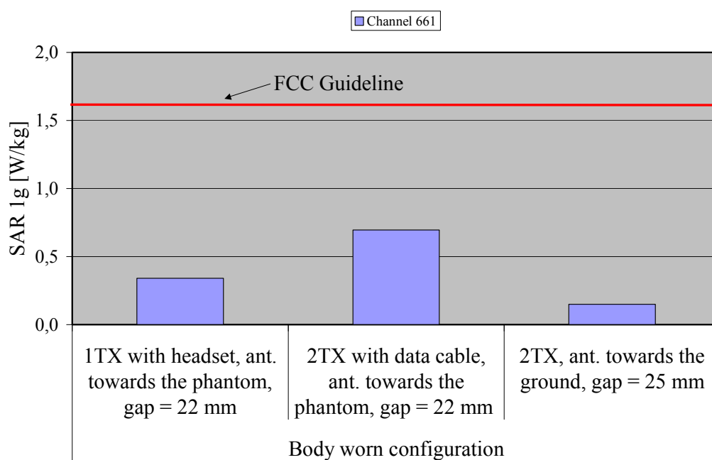
Fig. 17: The measured SAR values in body-worn configuration for the Siemens CX70 BF for PCS 1900 in comparison to the FCC exposure limit.
