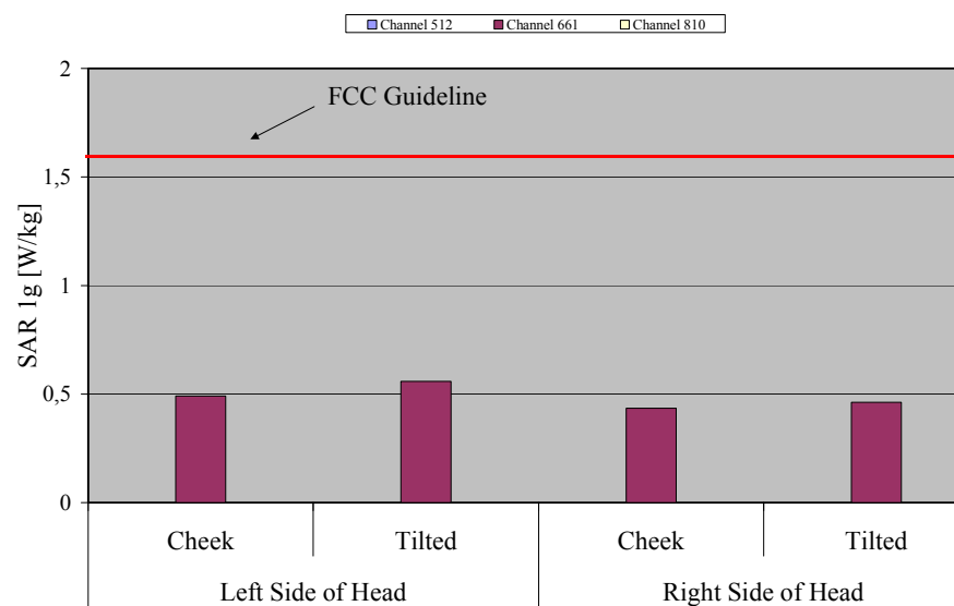
Fig. 13: The measured head phantom SAR values for the Siemens CX70 BF with Flash for PCS 1900 in comparison to the FCC exposure limit.
