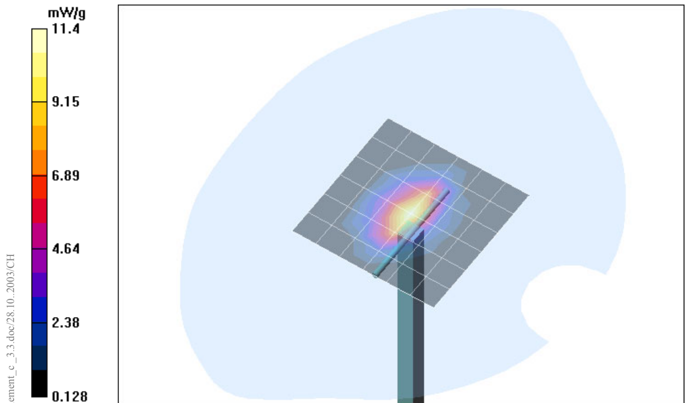
Fig. 20: Validation measurement 1900 MHz Head (August 11, 2004), coarse grid.
