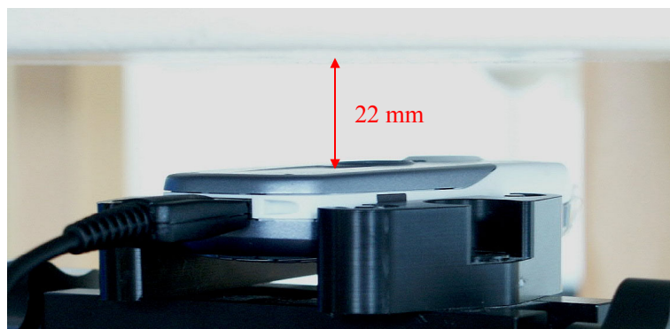
Fig. 69: Body worn configuration CX70 BF, GPRS mode (2 TX slots) with data cable, antenna towards the phantom
