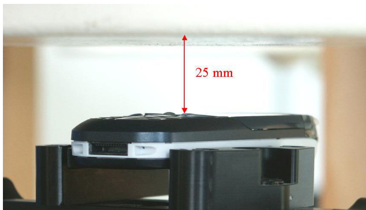
Fig. 72: Body worn configuration CX70 Standard, PTT GPRS mode (2 TX slots), antenna towards the ground.
