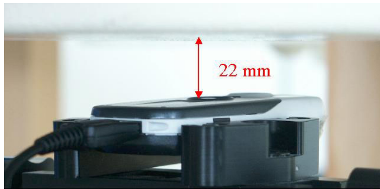
Fig. 70: Body worn configuration CX70 Butterfly, GPRS mode (2 TX slots) with data cable, antenna towards the phantom.
