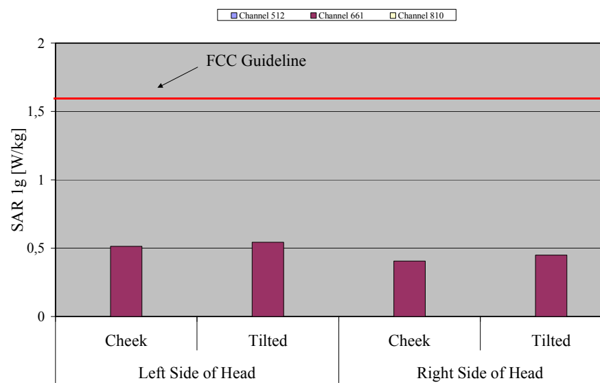
Fig. 15: The measured head phantom SAR values for the Siemens CX70 ARC with Flash for PCS 1900 in comparison to the FCC exposure limit.
