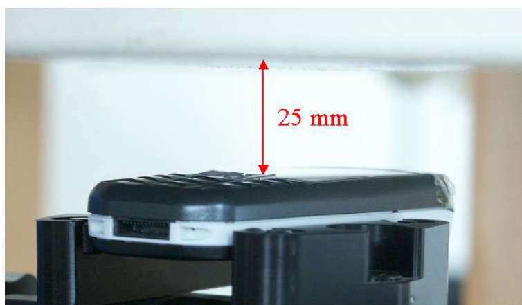
Fig. 74: Body worn configuration CX70 Butterfly, PTT GPRS mode (2 TX slots), antenna towards the ground..
