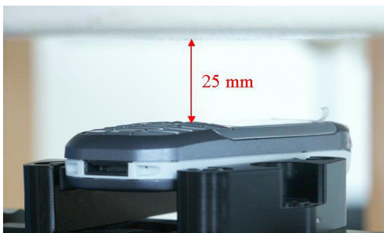
Fig. 73: Body worn configuration CX70 BF PTT GPRS mode (2 TX slots), antenna towards the ground..
