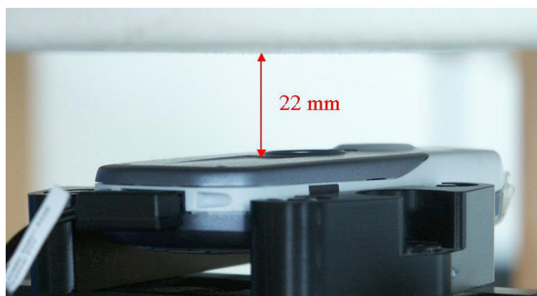
Fig. 67: Body worn configuration ARC, GSM mode (1 TX slot) with headset, antenna towards the phantom.
