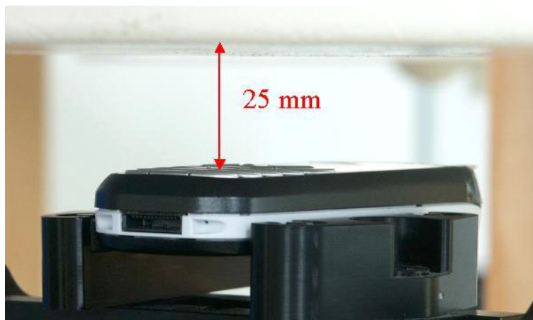
Fig. 75: Body worn configuration CX70 ARC, PTT GPRS mode (2 TX slots), antenna towards the ground.
