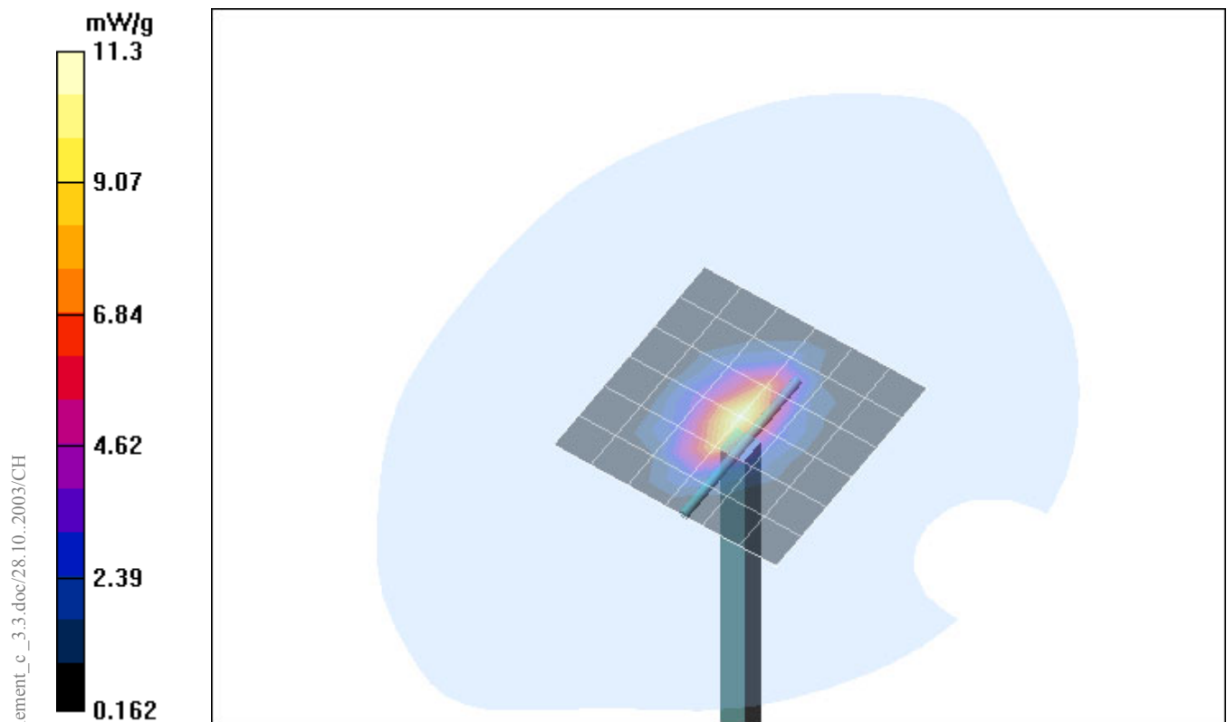
Fig. 21: Validation measurement 1900 MHz Head (August 12, 2004), coarse grid.
