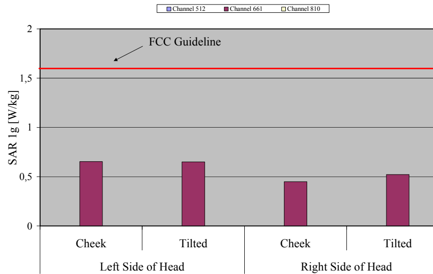
Fig. 10: The measured head phantom SAR values for the Siemens CX70 Butterfly for PCS 1900 in comparison to the FCC exposure limit.
