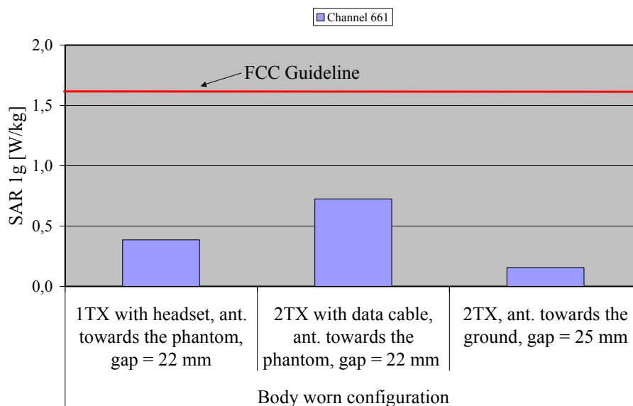
Fig. 18: The measured SAR values in body-worn configuration for the Siemens CX70 Butterfly for PCS 1900 in comparison to the FCC exposure limit.
