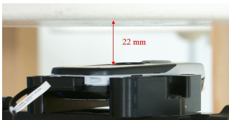
Fig. 65: Body worn configuration BF, GSM mode (1 TX slot) with headset, antenna towards the phantom.
