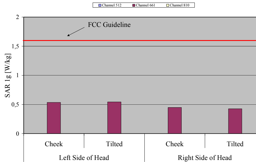
Fig. 14: The measured head phantom SAR values for the Siemens CX70 Butterfly with Flash for PCS 1900 in comparison to the FCC exposure limit.
