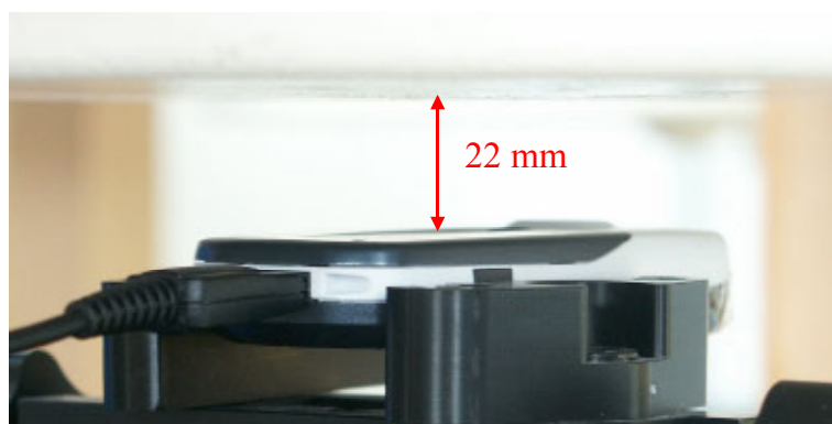
Fig. 68: Body worn configuration CX70 Standard, GPRS mode (2 TX slots) with data cable, antenna towards the phantom.
