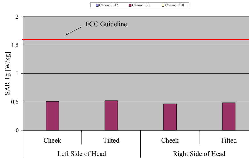
Fig. 12: The measured head phantom SAR values for the Siemens CX70 Standard with Flash for PCS 1900 in comparison to the FCC exposure limit.
