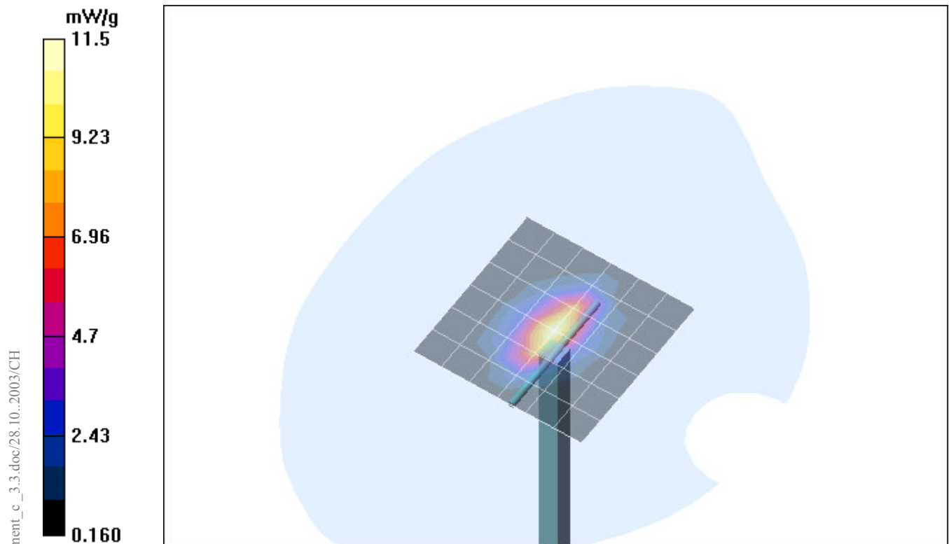
Fig. 22: Validation measurement 1900 MHz body (August 06, 2004), coarse grid. Ambient Temperature: 22.8° C, Liquid Temperature: 21.4° C.
