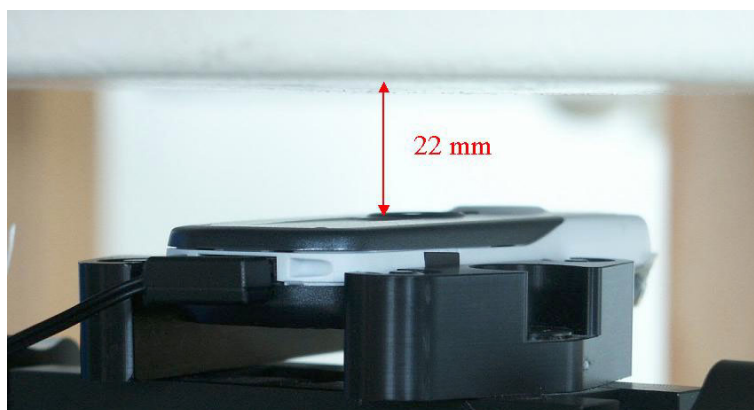
Fig. 66: Body worn configuration Butterfly, GSM mode (1 TX slot) with headset, antenna towards the phantom.
