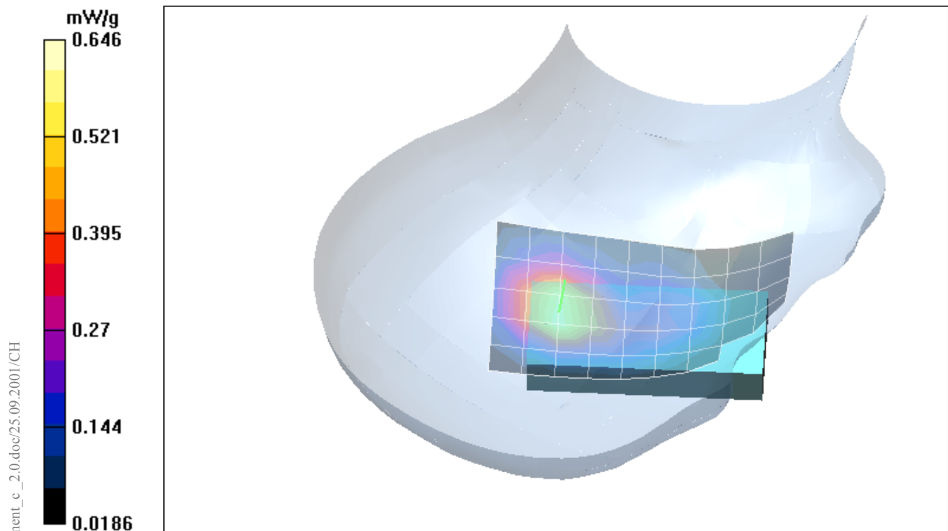
Fig. 11: SAR distribution for PCS 1900, channel 661, cheek position, right side of head, Butterfly. (18.02.2004; Ambient Temperature: 20.9° C; Liquid Temperature : 19.9° C).
