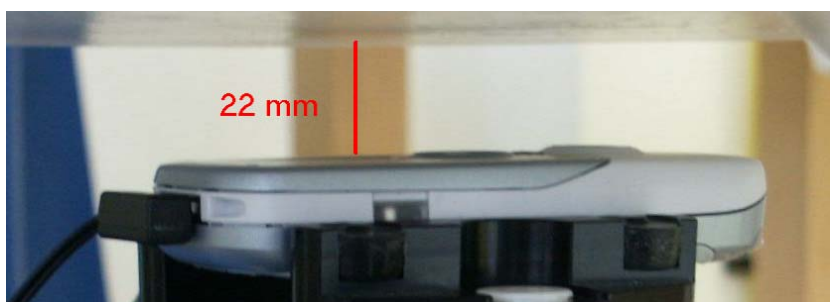
Fig. 55: Body worn configuration BF, GSM mode (1 TX slot) with headset, antenna towards the phantom.
