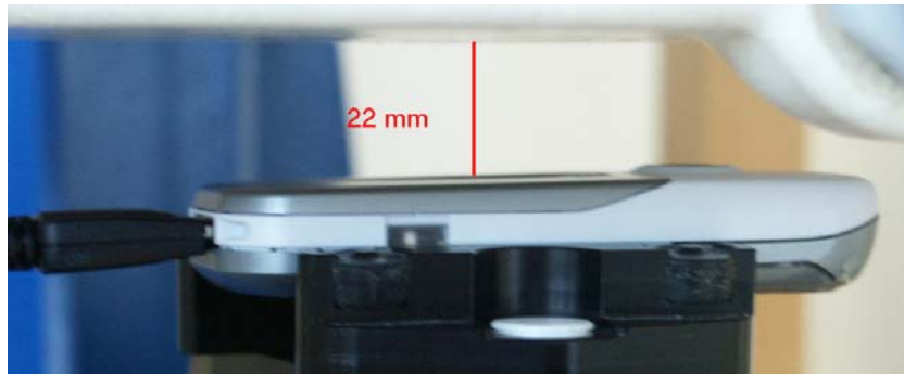
Fig. 58: Body worn configuration Standard, GPRS mode (2 TX slots) with data cable, antenna towards the phantom.
