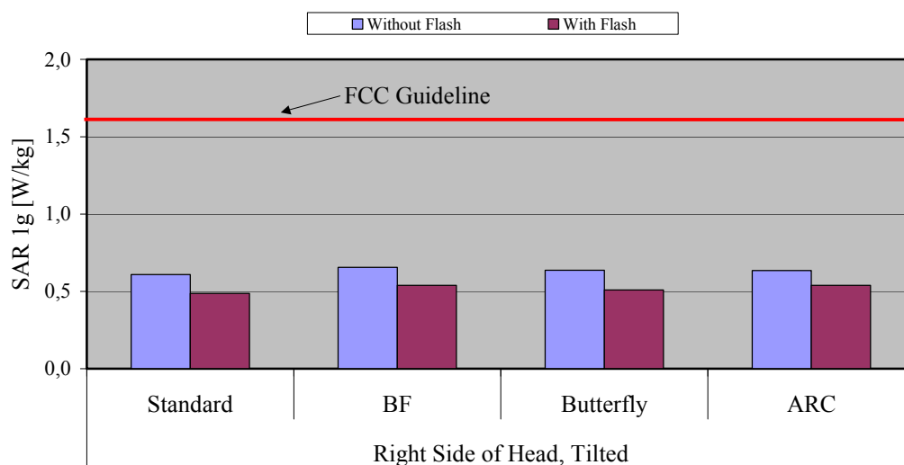
Fig. 11: The measured head phantom SAR values for the Siemens CX65 without and with flash for PCS 1900 in comparison to the FCC exposure limit.
