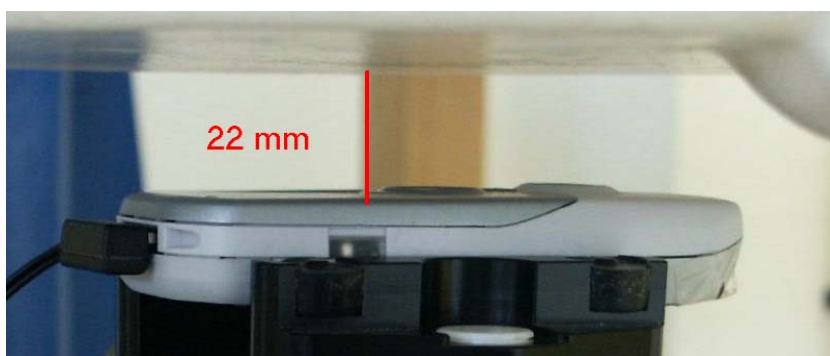
Fig. 57: Body worn configuration ARC, GSM mode (1 TX slot) with headset, antenna towards the phantom.
