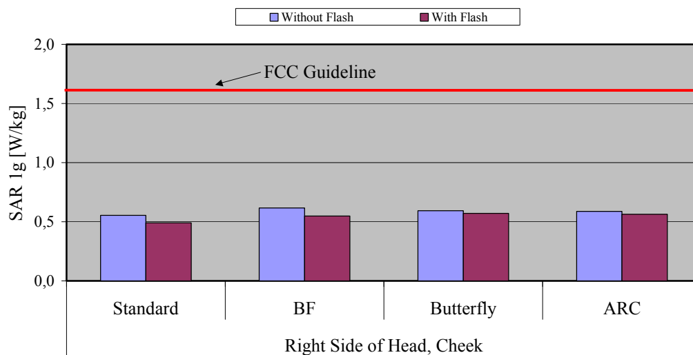
Fig. 10: The measured head phantom SAR values for the Siemens CX65 without and with flash for PCS 1900 in comparison to the FCC exposure limit.
