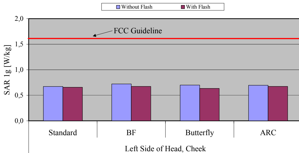
Fig. 8: The measured head phantom SAR values for the Siemens CX65 without and with flash for PCS 1900 in comparison to the FCC exposure limit.
