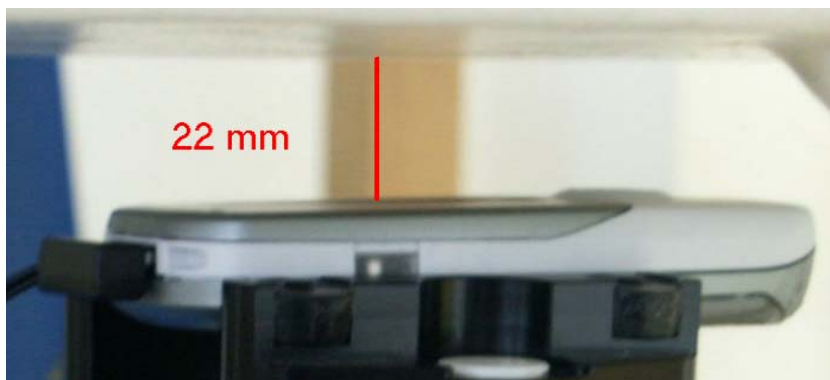
Fig. 54: Body worn configuration Standard, GSM mode (1 TX slot) with headset, antenna towards the phantom.
