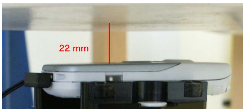
Fig. 56: Body worn configuration Butterfly, GSM mode (1 TX slot) with headset, antenna towards the phantom.
