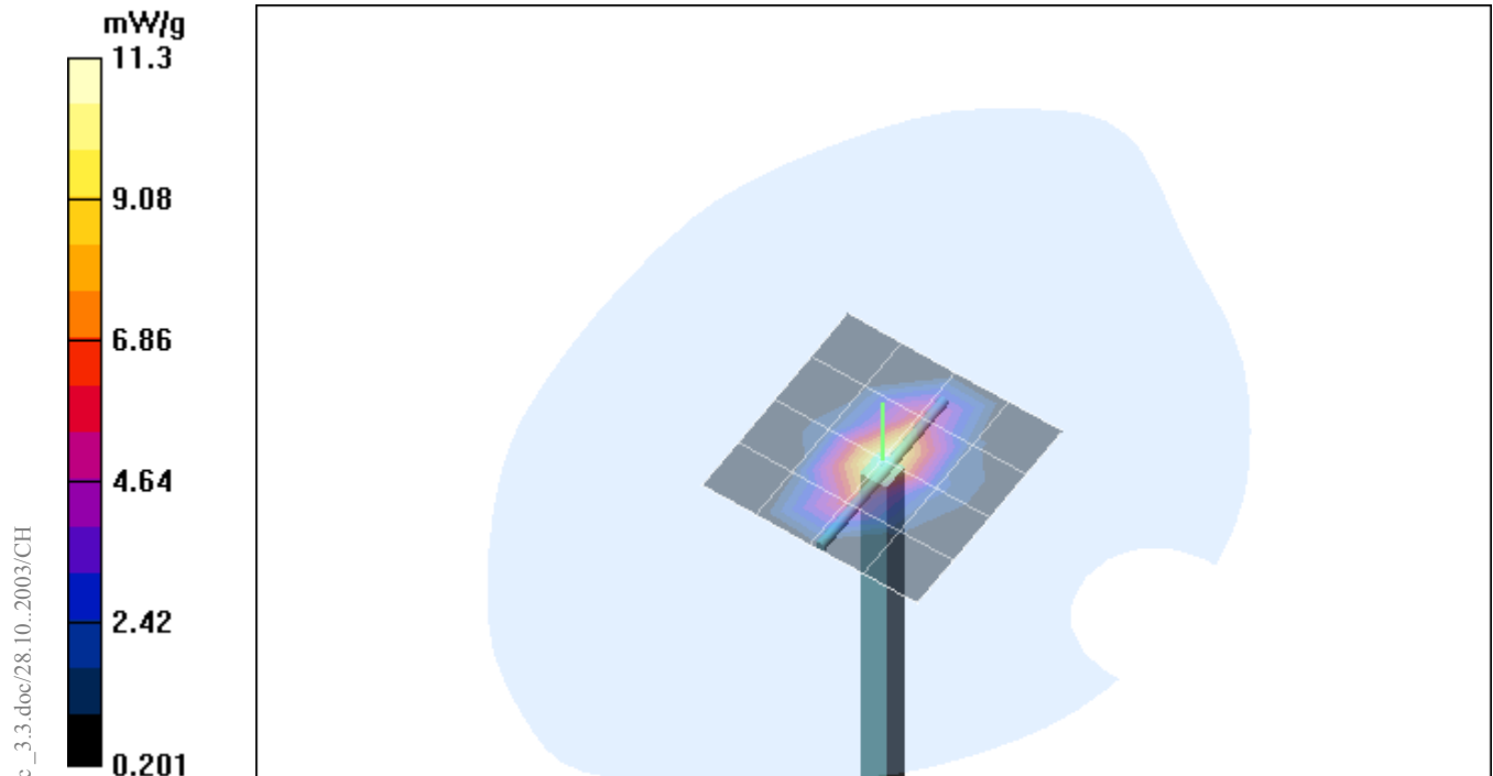
Fig. 13: Validation measurement 1900 MHz Head (February 18, 2004), coarse grid. Ambient Temperature: 20.9° C, Liquid Temperature: 19.8° C.
