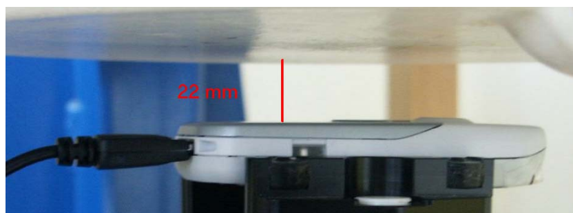
Fig. 61: Body worn configuration ARC, GPRS mode (2 TX slots) with data cable, antenna towards the phantom.
