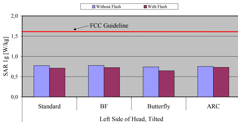
Fig. 9: The measured head phantom SAR values for the Siemens CX65 without and with flash for PCS 1900 in comparison to the FCC exposure limit.
