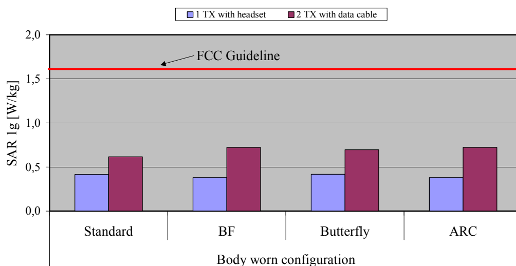
Fig. 12: The measured SAR values in body-worn configuration for the Siemens CX65 for PCS 1900 (1 TX slot with headset and 2 TX slots with data cable, gap = 22 mm) in comparison to the FCC exposure limit.
