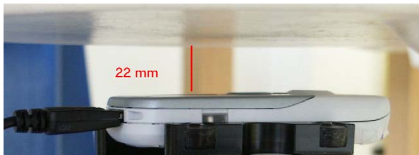
Fig. 60: Body worn configuration Butterfly, GPRS mode (2 TX slots) with data cable, antenna towards the phantom.
