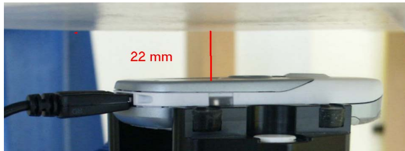
Fig. 59: Body worn configuration BF, GPRS mode (2 TX slots) with data cable, antenna towards the phantom.
