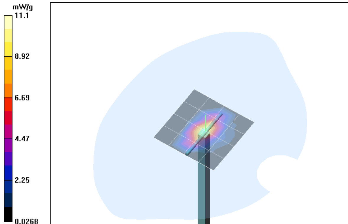
Fig. 14: Validation measurement 1900 MHz body (February 22, 2004), coarse grid. Ambient Temperature: 20.4° C, Liquid Temperature: 19.6° C.
