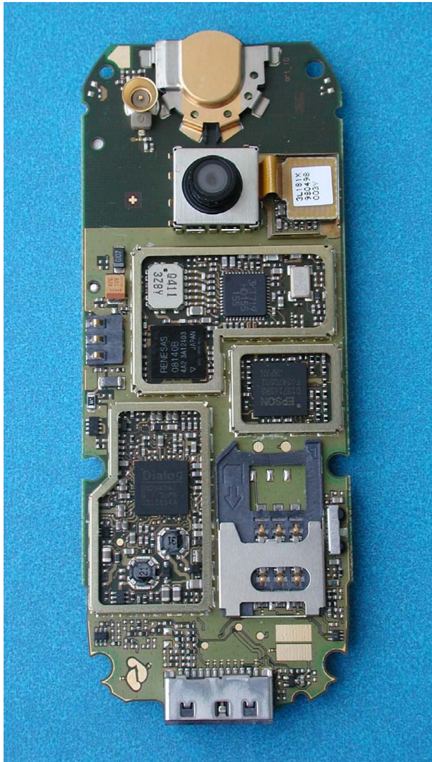
CX-65 PCB Rear View Shields Removed
