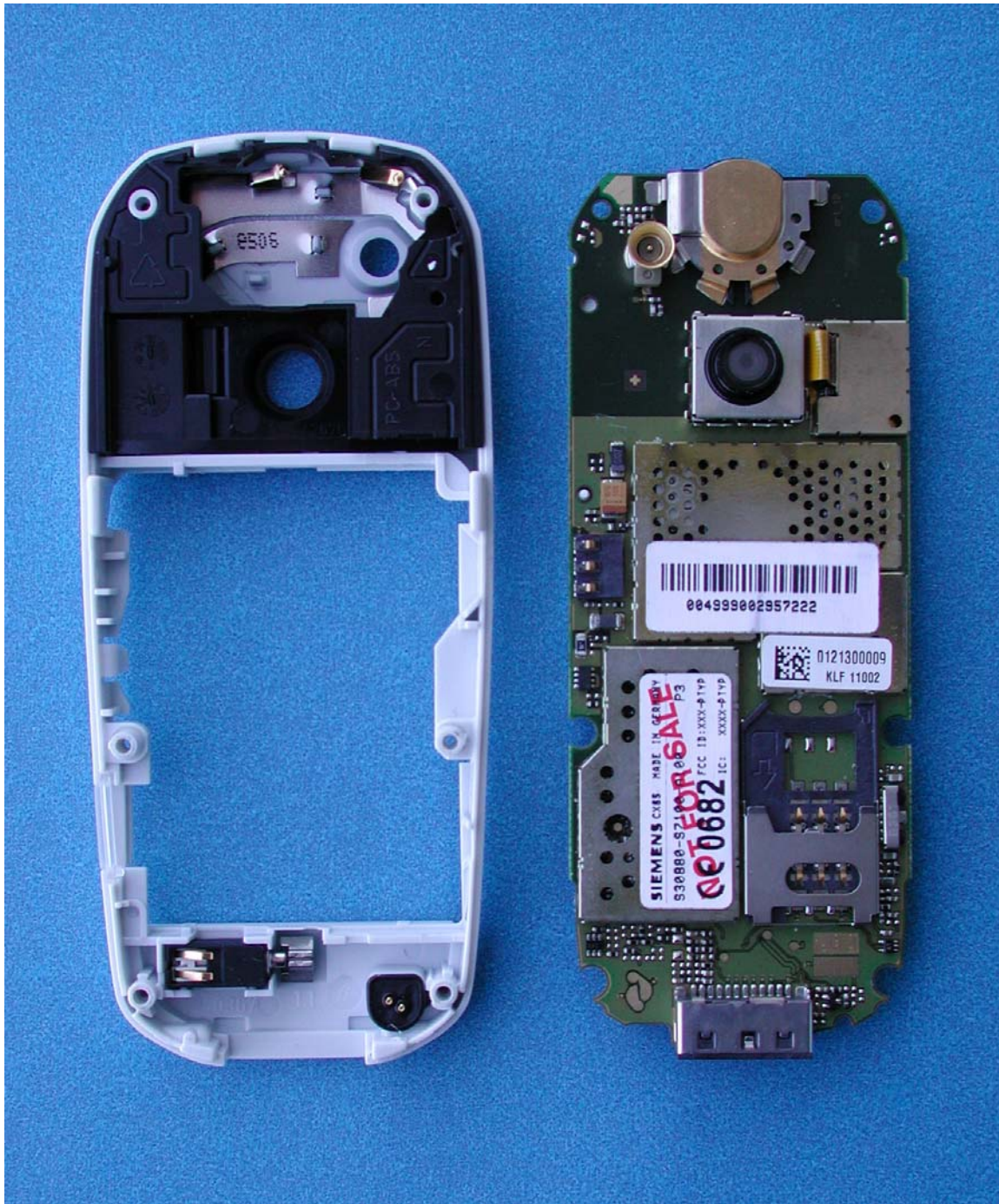
CX-65 Disassembly step 2
