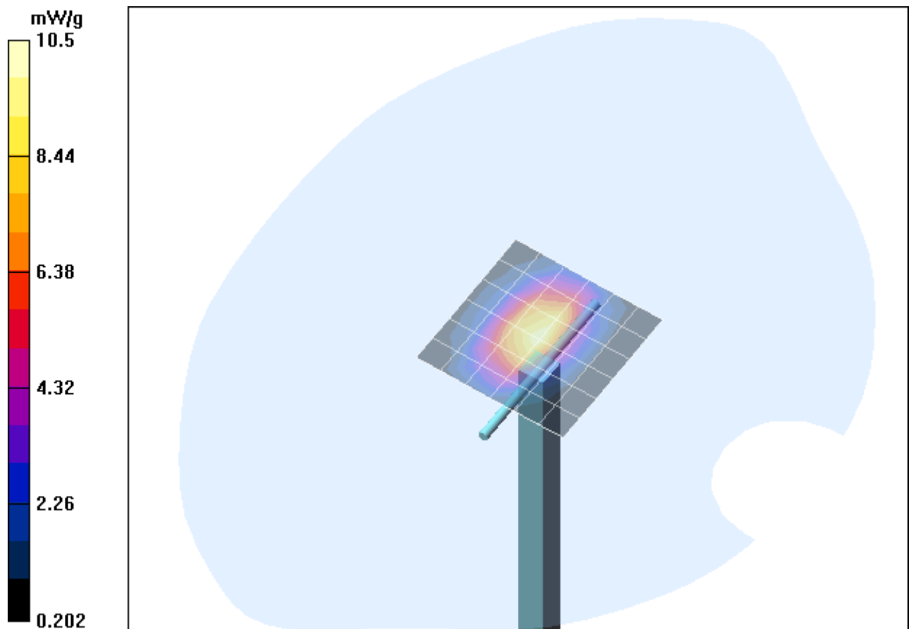
Fig. 11: Validation measurement 1900 MHz Head (September 09, 2005), coarse grid. Ambient Temperature: 21.8° C, Liquid Temperature: 20.9° C.
