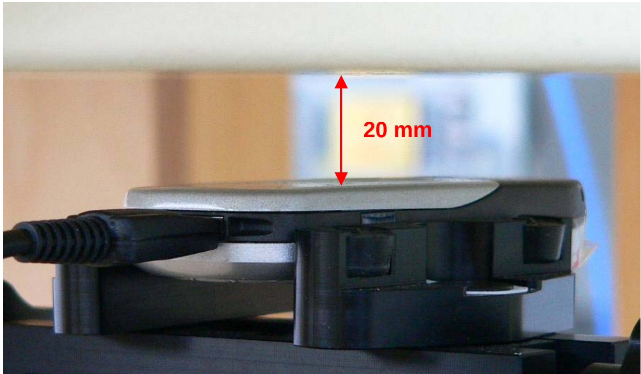
Fig. 29: Body worn configuration Siemens C72, GPRS Class 10, with data cable, antenna towards the phantom, gap= 20 mm.
