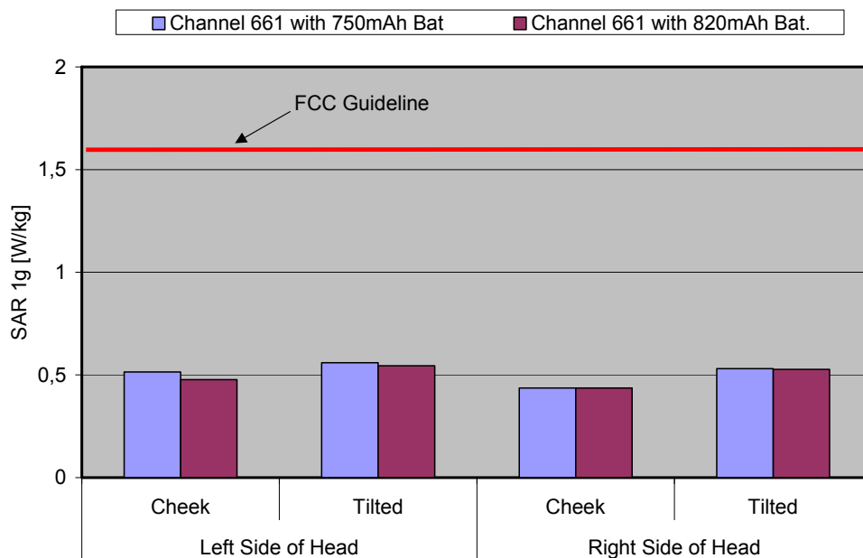
Fig. 8: The measured head phantom SAR values for the Siemens C72 for PCS 1900 in comparison to the FCC exposure limit.
