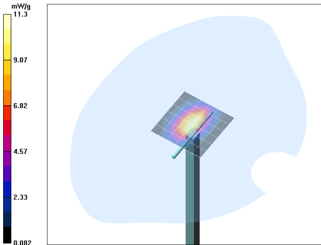
Fig. 12: Validation measurement 1900 MHz body (September 12, 2005), coarse grid. Ambient Temperature: 22.0° C, Liquid Temperature: 20.9° C.
