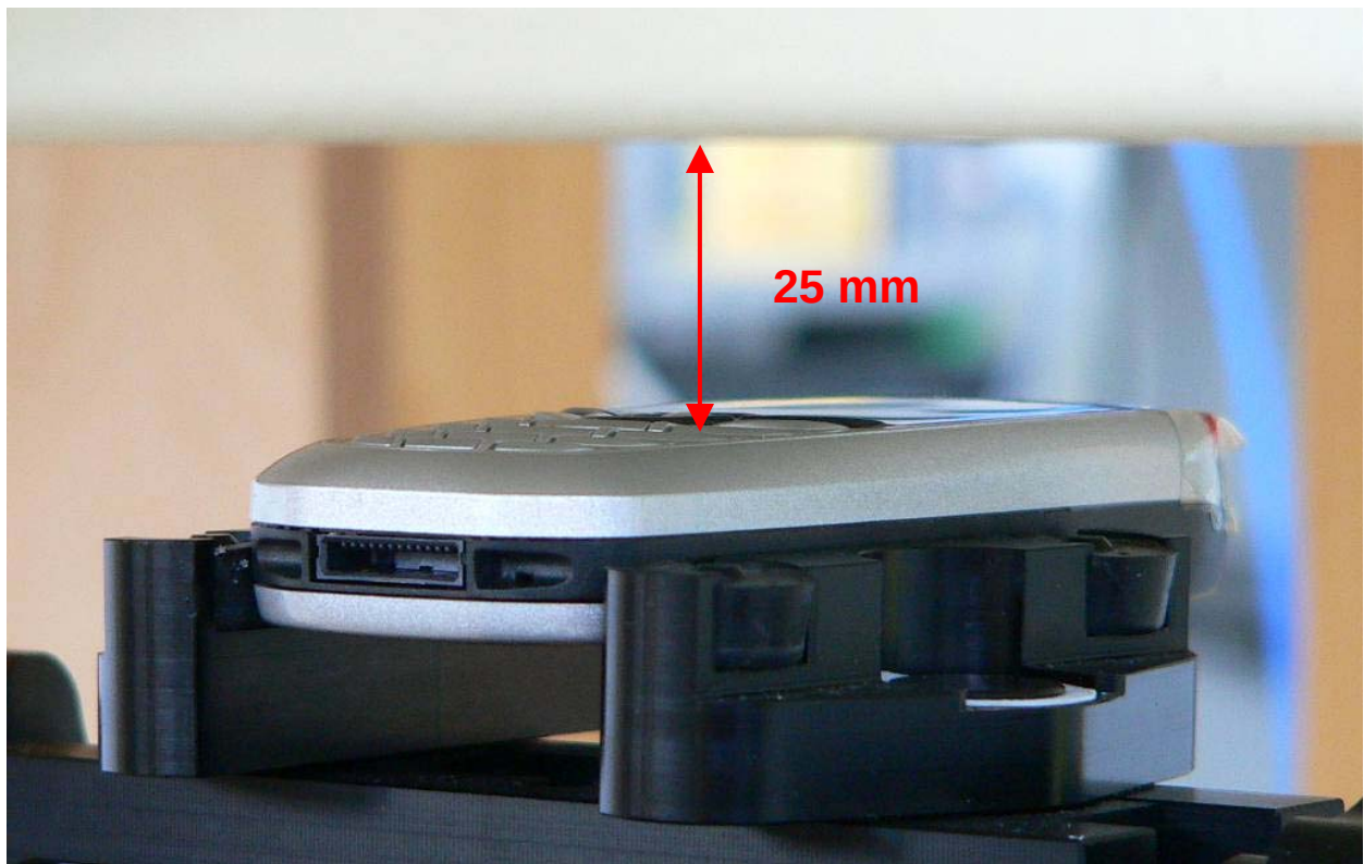
Fig. 30: Body worn configuration Siemens C72, GPRS Class 10, in PTT configuration, antenna towards the ground, gap= 25 mm.
