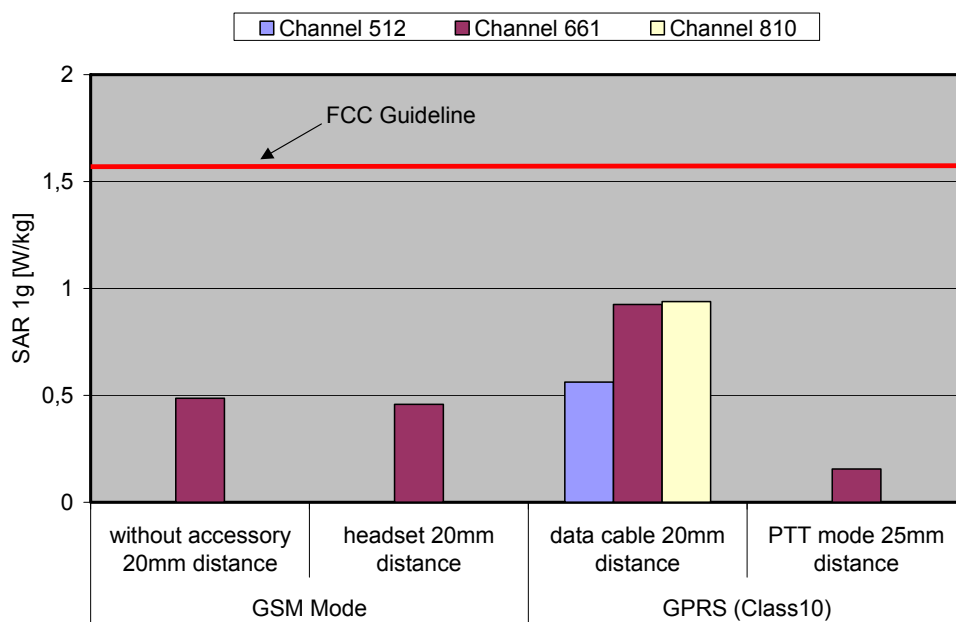
Fig. 10: The measured SAR values in body-worn configuration for the Siemens C72 for PCS 1900 in comparison to the FCC exposure limit.
