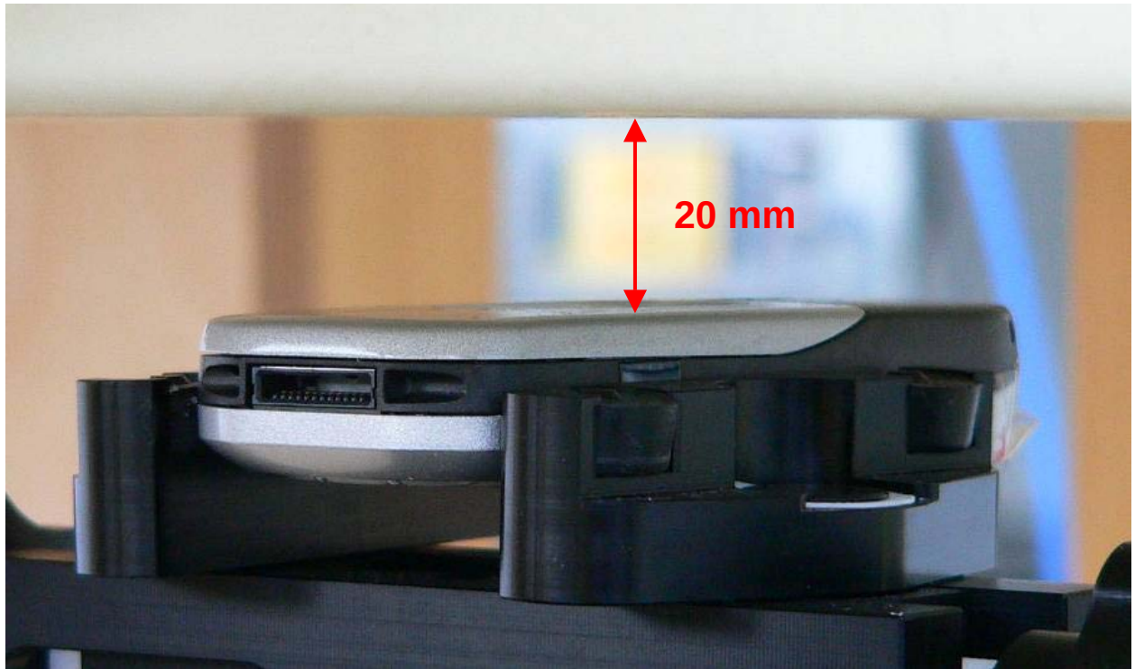
Fig. 27: Body worn configuration, GSM without accessory, antenna towards the phantom.
