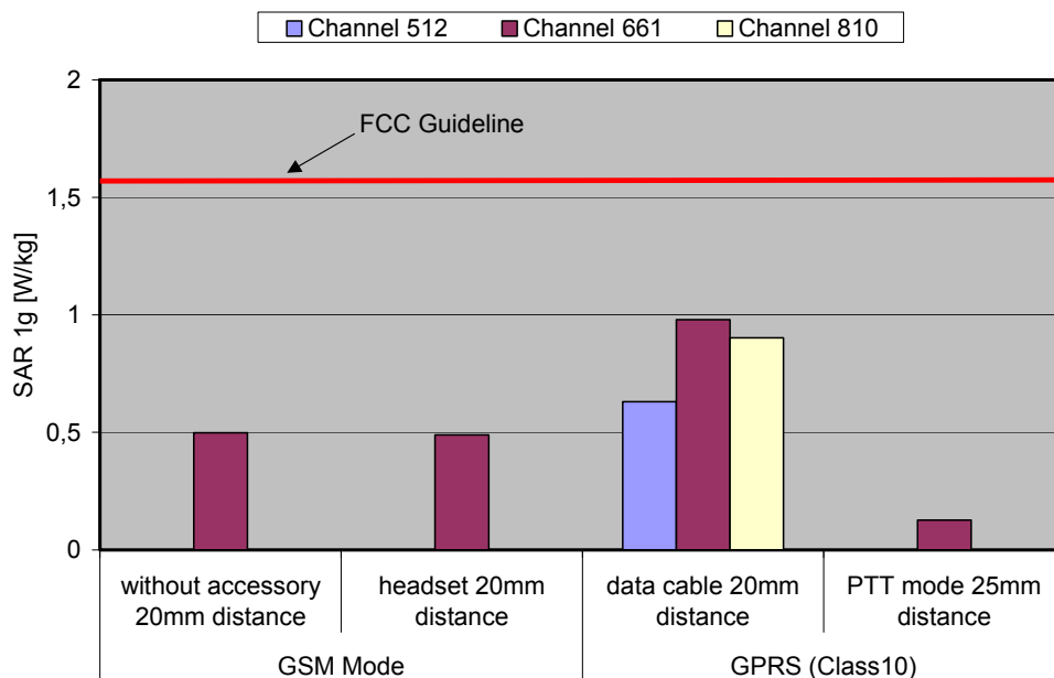
Fig. 9: The measured SAR values in body-worn configuration for the Siemens C72 with 750mAh bat. for PCS 1900 in comparison to the FCC exposure limit.
