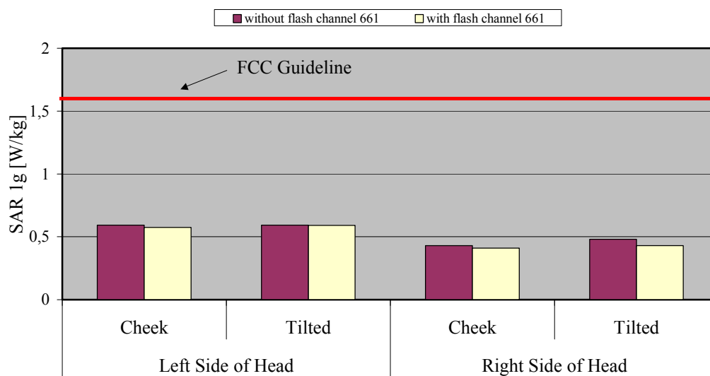
Fig. 11: The measured head phantom SAR values for the Siemens C66 Butterfly without and with flash for PCS 1900 in comparison to the FCC exposure limit.
