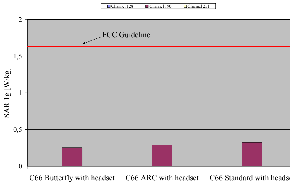
Fig. 14: The measured SAR values in body-worn configuration for the Siemens C66 for GSM 850 (1 TX slot with headset, gap = 22 mm) in comparison to the FCC exposure limit.
