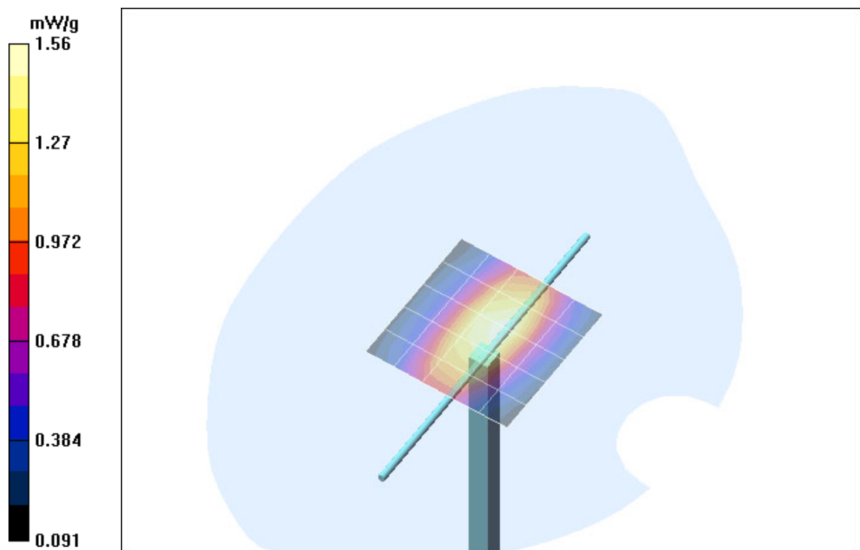
Fig. 22: Validation measurement 835MHz Head (Standard) (July 27, 2004), coarse grid. Ambient Temperature: 21.0° C, Liquid Temperature: 20.4° C.
