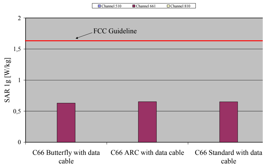
Fig. 17: The measured SAR values in body-worn configuration for the Siemens C66 for PCS 1900 (2 TX slots with data cable, gap = 22 mm) in comparison to the FCC exposure limit.
