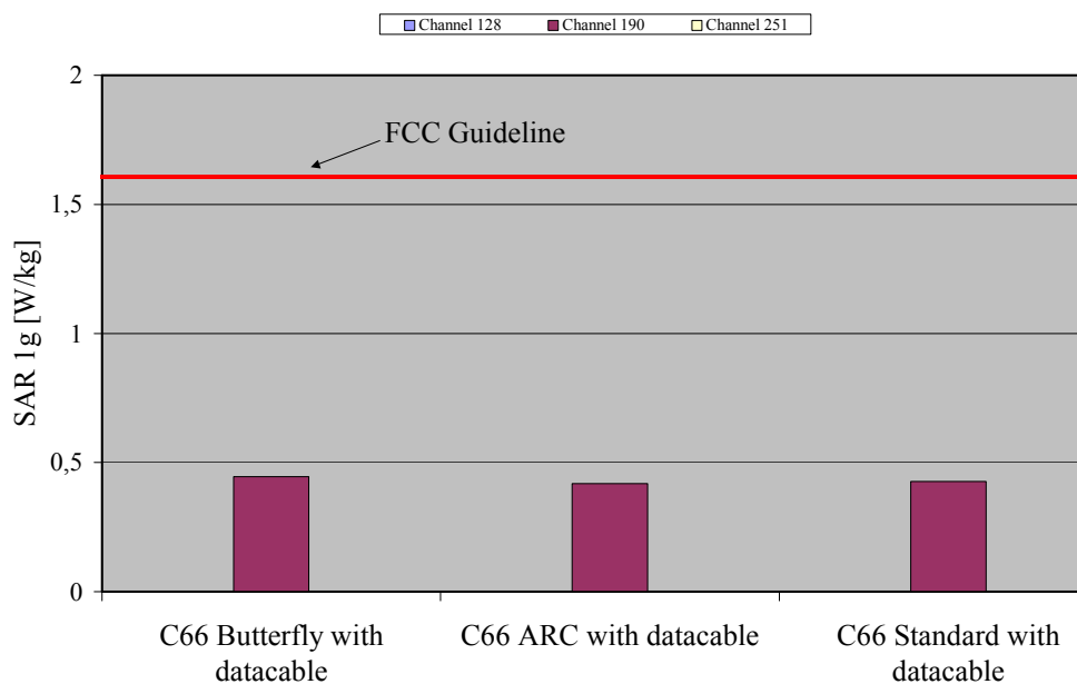
Fig. 15: The measured SAR values in body-worn configuration for the Siemens C66 for GSM 850 (2 TX slot with datacable, gap = 22 mm) in comparison to the FCC exposure limit.
