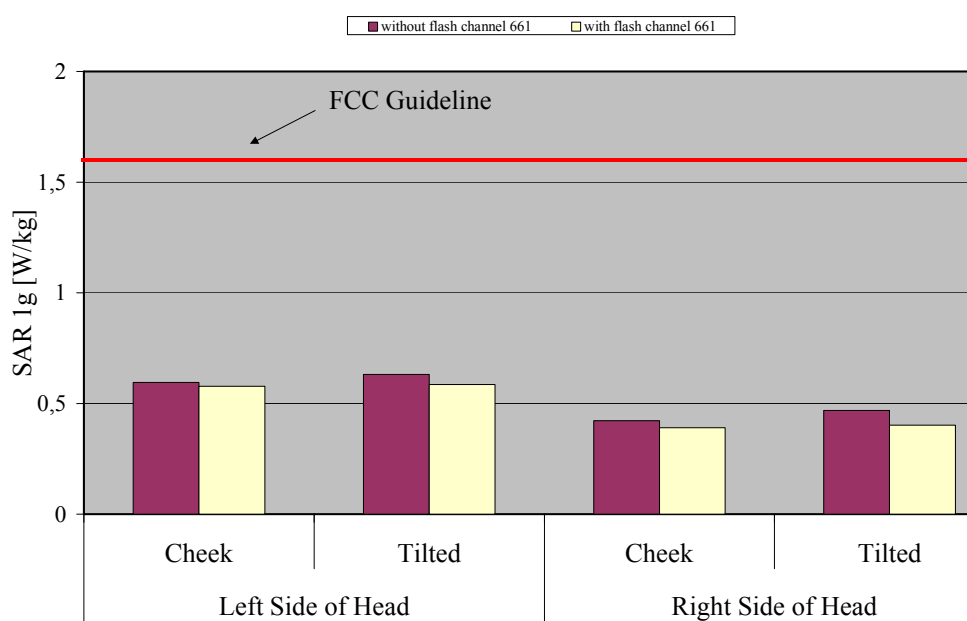
Fig. 13: The measured head phantom SAR values for the Siemens C66 Standard without and with flash for PCS 1900 in comparison to the FCC exposure limit.
