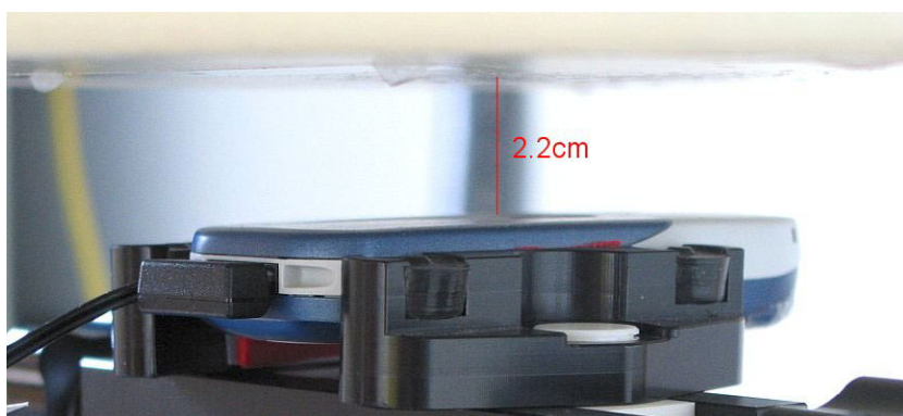
Fig. 58: Body worn configuration Standard, GSM mode (1 TX slot) with headset, antenna towards the phantom.
