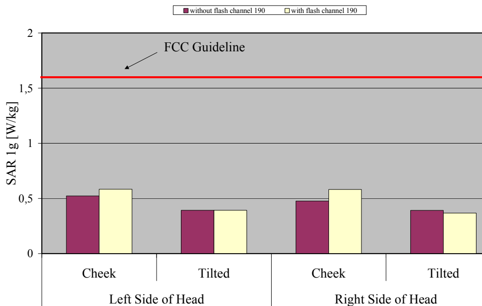
Fig. 10: The measured head phantom SAR values for the Siemens C66 Standard without and with flash for GSM 850 in comparison to the FCC exposure limit.
