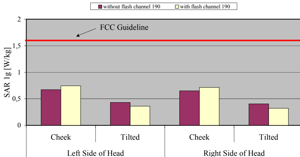
Fig. 8: The measured head phantom SAR values for the Siemens C66 Butterfly without and with flash for GSM 850 in comparison to the FCC exposure limit.
