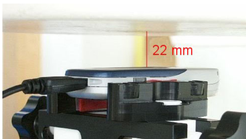
Fig. 60: Body worn configuration ARC, GPRS mode (2 TX slots) with data cable, antenna towards the phantom.
