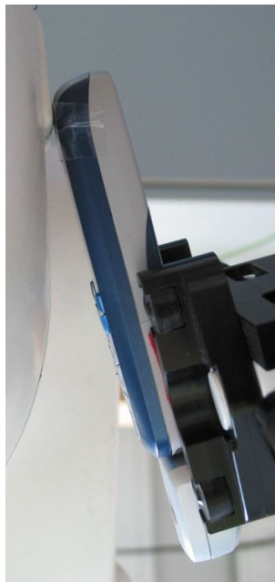
Fig. 53: Tilted position, left side, Standard with flash.
