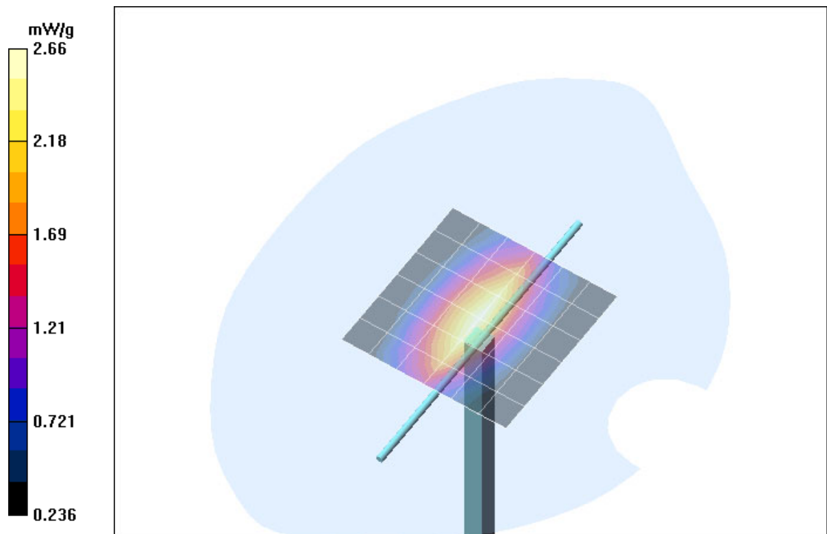
Fig. 19: Validation measurement 835 MHz body (ARC, Butterfly) (June 22, 2004), coarse grid. Ambient Temperature: 21.5° C, Liquid Temperature: 20.5° C.
