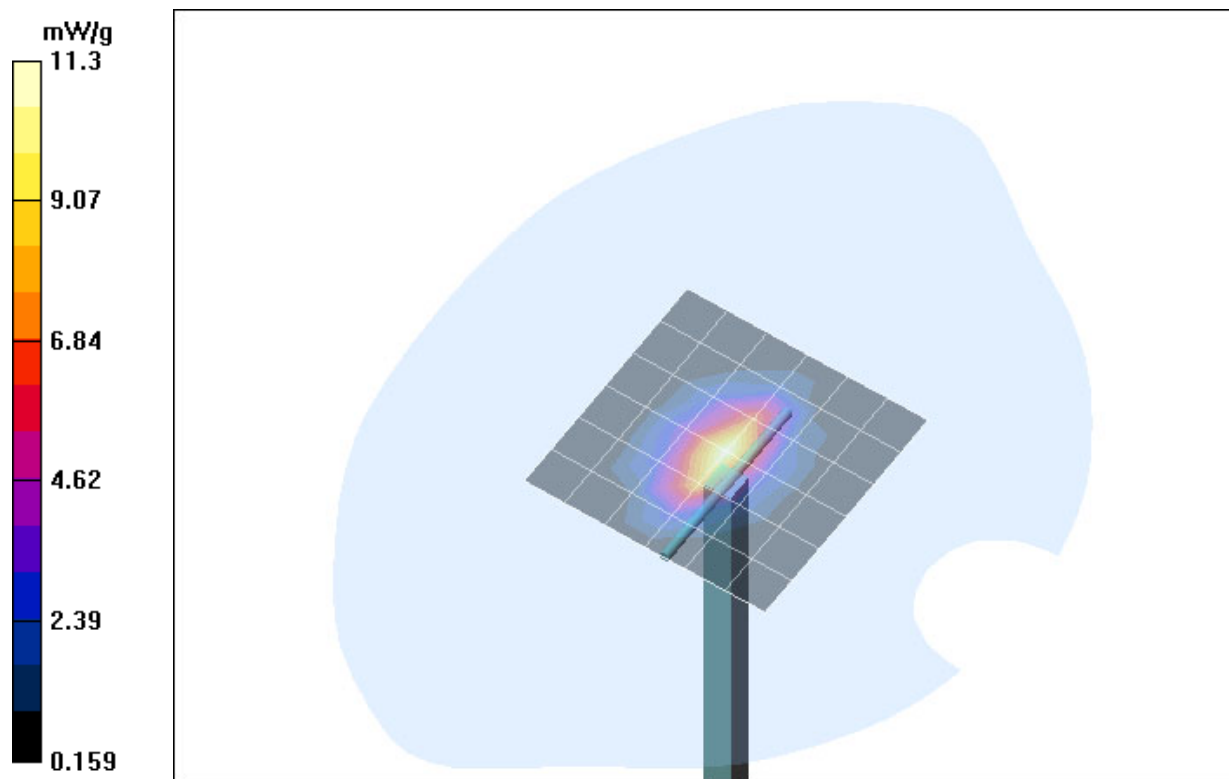
Fig. 20: Validation measurement 1900 MHz Head (ARC, Butterfly) (June 18, 2004), coarse grid. Ambient Temperature: 21.5° C, Liquid Temperature: 20.4° C.
