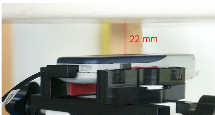
Fig. 57: Body worn configuration ARC, GSM mode (1 TX slot) with headset, antenna towards the phantom.
