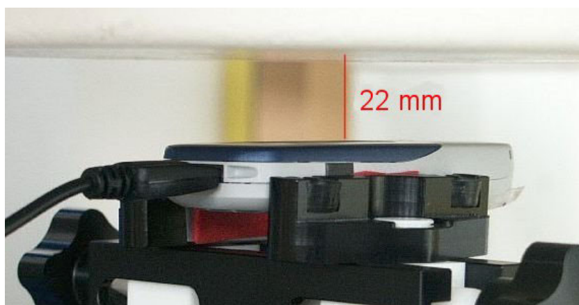
Fig. 59: Body worn configuration Butterfly, GPRS mode (2 TX slots) with data cable, antenna towards the phantom.
