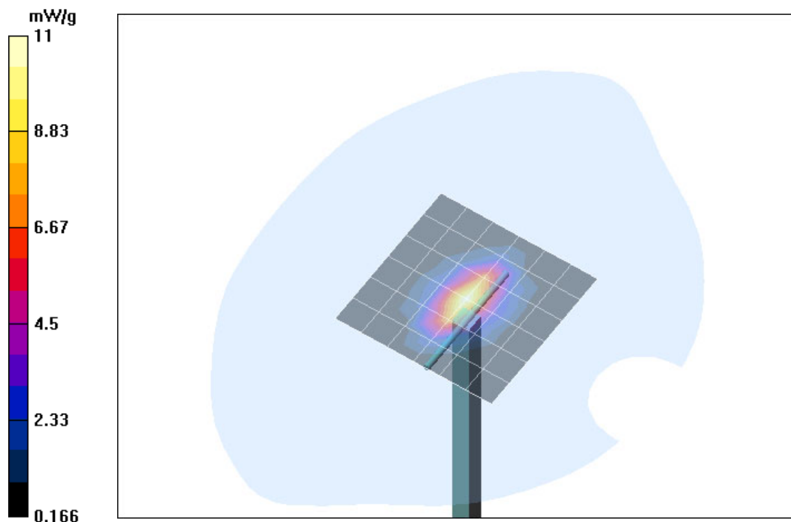
Fig. 21: Validation measurement 1900 MHz body (ARC, Butterfly) (June 21, 2004), coarse grid. Ambient Temperature: 21.4° C, Liquid Temperature: 20.7° C.
