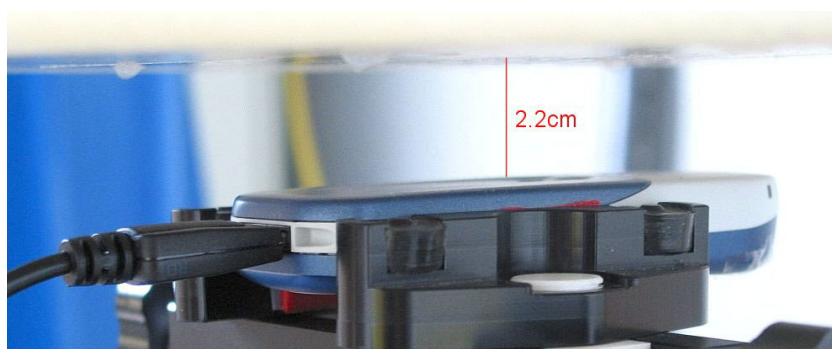
Fig. 61: Body worn configuration Standard, GPRS mode (2 TX slots) with data cable, antenna towards the phantom.
