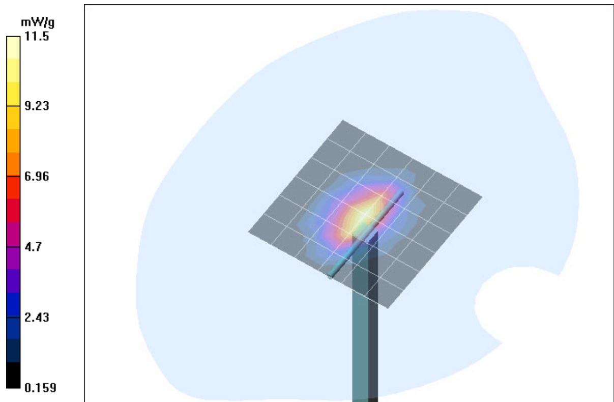
Fig. 24: Validation measurement 1900 MHz Head (Standard) (July 23, 2004), coarse grid. Ambient Temperature: 21.0° C, Liquid Temperature: 20.5° C.
