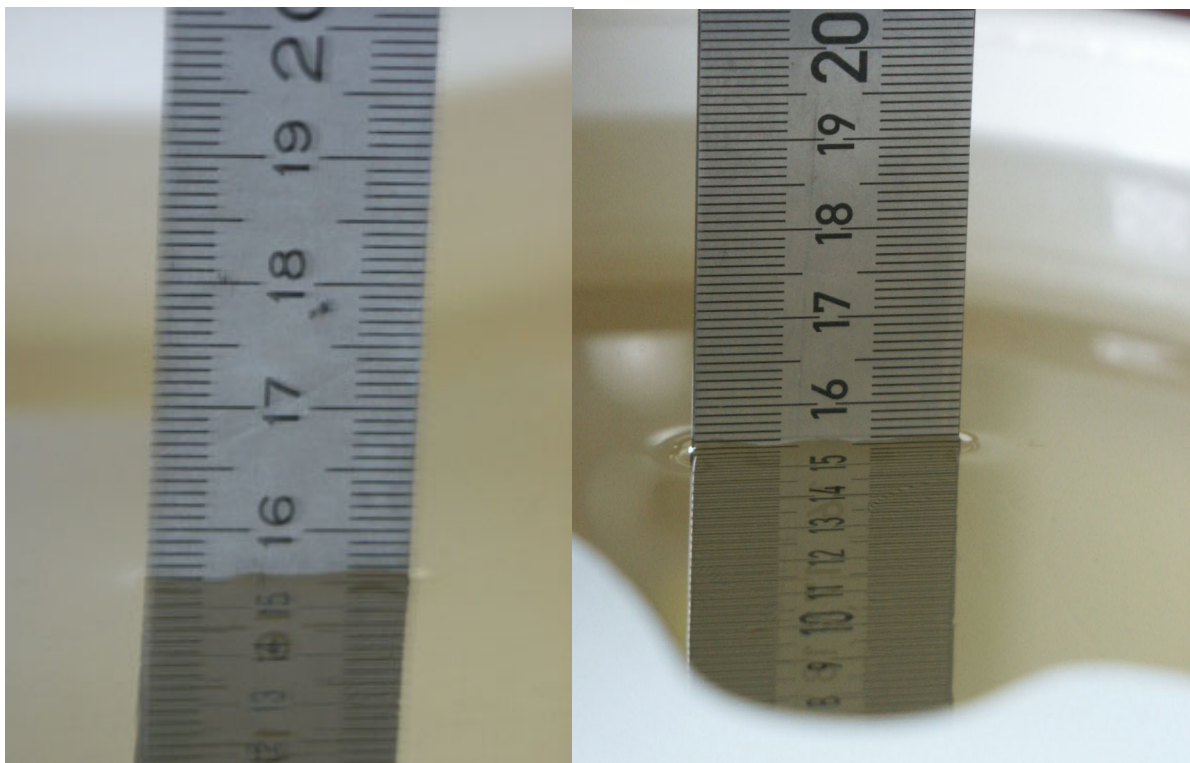
Fig. 62: Liquid depth for GSM 850 Head and Body measurements.
