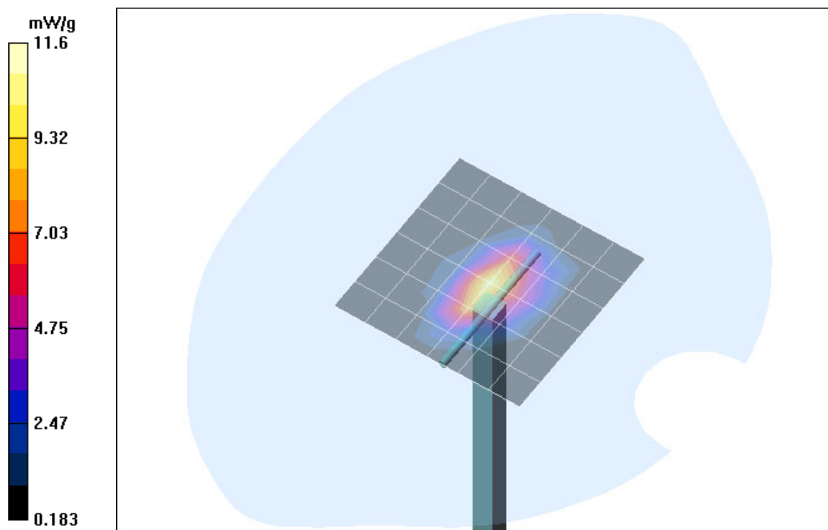
Fig. 25: Validation measurement 1900 MHz body (Standard) (July 27, 2004), coarse grid. Ambient Temperature: 21.7° C, Liquid Temperature: 20.7° C.
