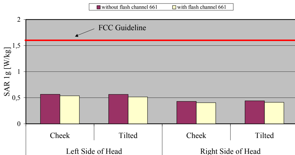
Fig. 12: The measured head phantom SAR values for the Siemens C66 ARC without and with flash for PCS 1900 in comparison to the FCC exposure limit.
