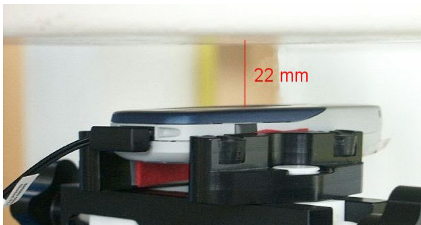
Fig. 56: Body worn configuration Butterfly, GSM mode (1 TX slot) with headset, antenna towards the phantom.
