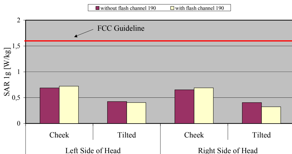
Fig. 9: The measured head phantom SAR values for the Siemens C66 ARC without and with flash for GSM 850 in comparison to the FCC exposure limit.
