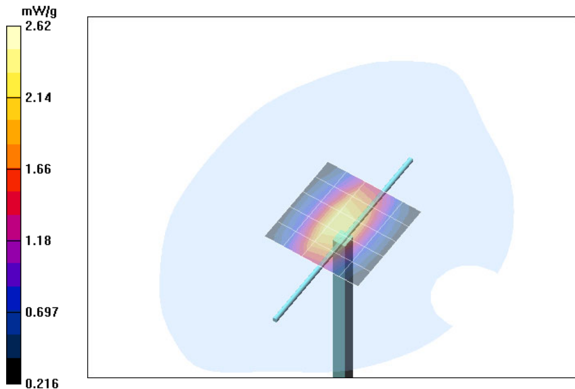
Fig. 18: Validation measurement 835MHz Head (ARC, Butterfly) (June 16, 2004), coarse grid. Ambient Temperature: 22.0° C, Liquid Temperature: 21.0° C.
