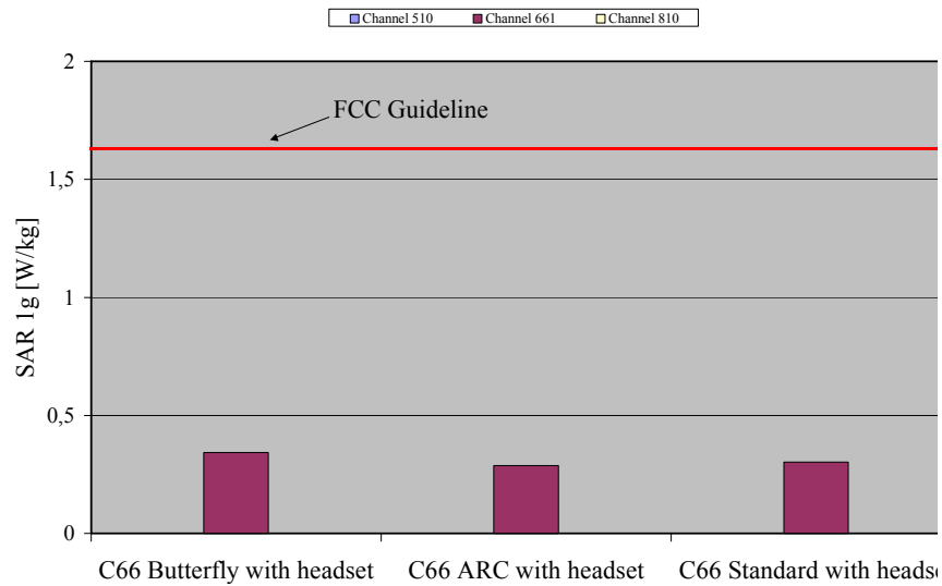
Fig. 16: The measured SAR values in body-worn configuration for the Siemens C66 for PCS 1900 (1 TX slots with headset, gap = 22 mm) in comparison to the FCC exposure limit.
