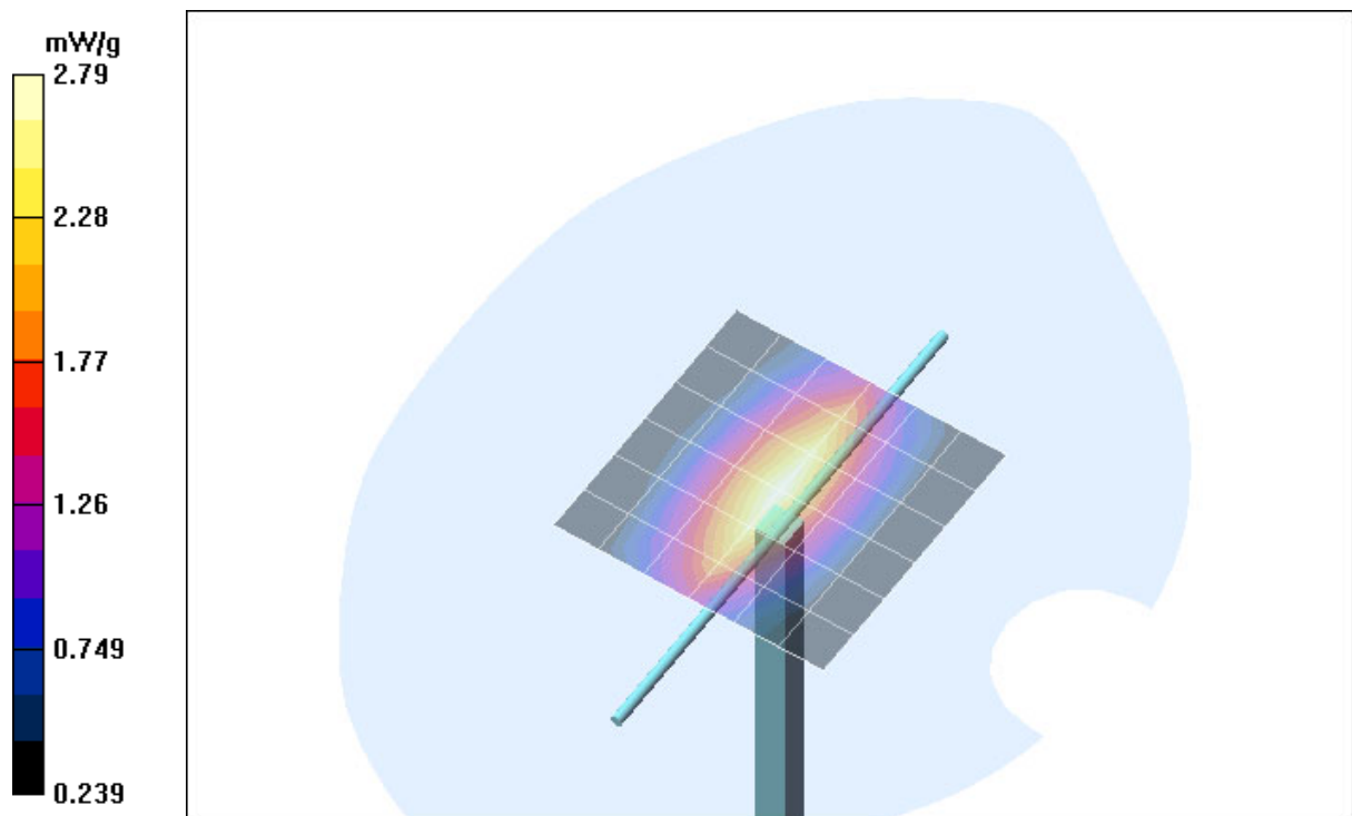
Fig. 23: Validation measurement 835 MHz body (Standard) (July 29, 2004), coarse grid. Ambient Temperature: 22.2° C, Liquid Temperature: 21.0° C.
