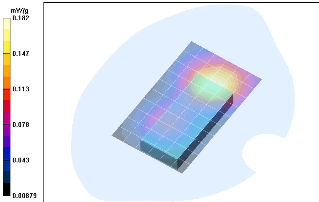
Fig. 1: SAR distribution for PCS 1900, channel 661, PoC (PTT) configuration, display towards the phantom, ARC cover, GPRS class 10 (18.10.2004; Ambient Temperature: 22.2° C; Liquid Temperature : 21.3° C).
