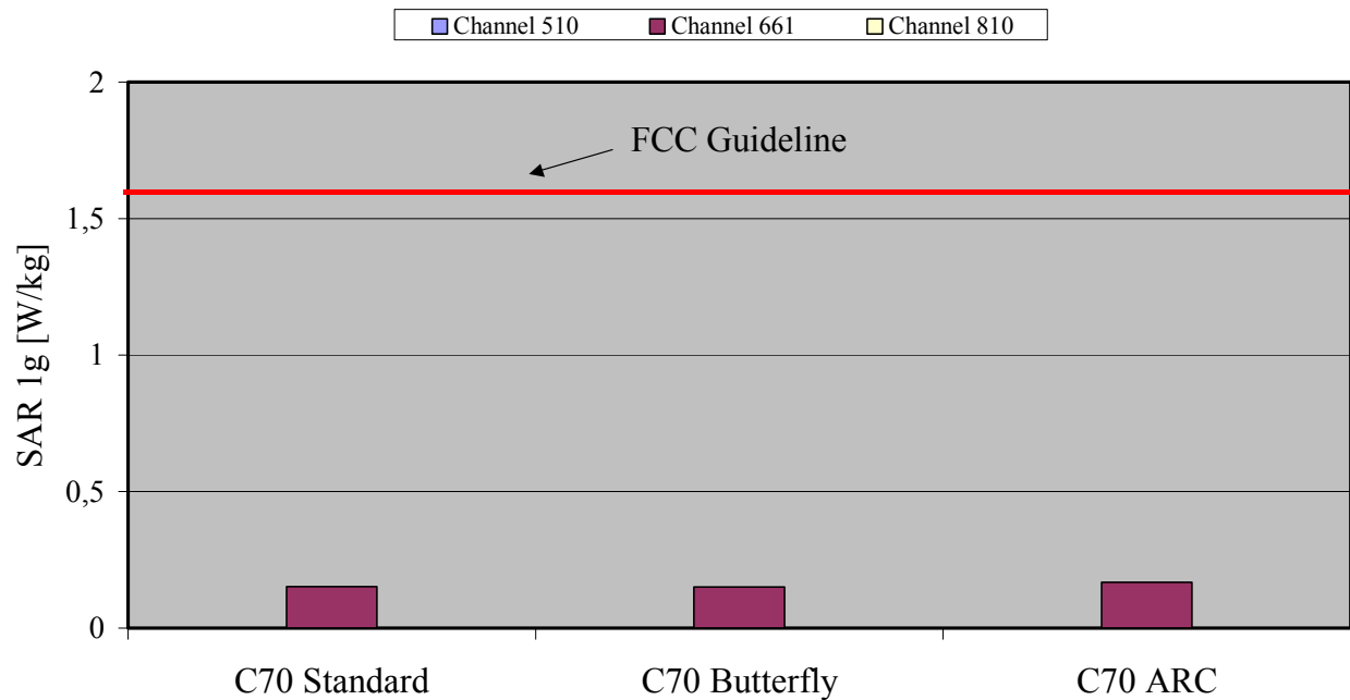
Fig. 8: The measured SAR values in PoC (PTT) configuration for the Siemens C70 for PCS 1900, GPRS class 10, gap = 25 mm, in comparison to the FCC exposure limit.
