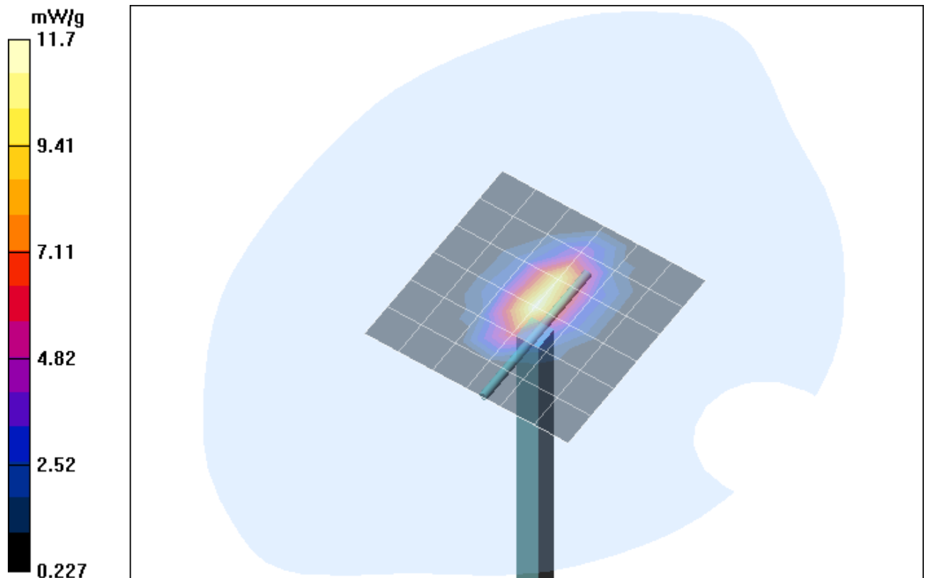
Fig. 9: Validation measurement 1900 MHz body (October 18, 2004), coarse grid. Ambient Temperature: 22.2° C, Liquid Temperature: 21.3° C.
